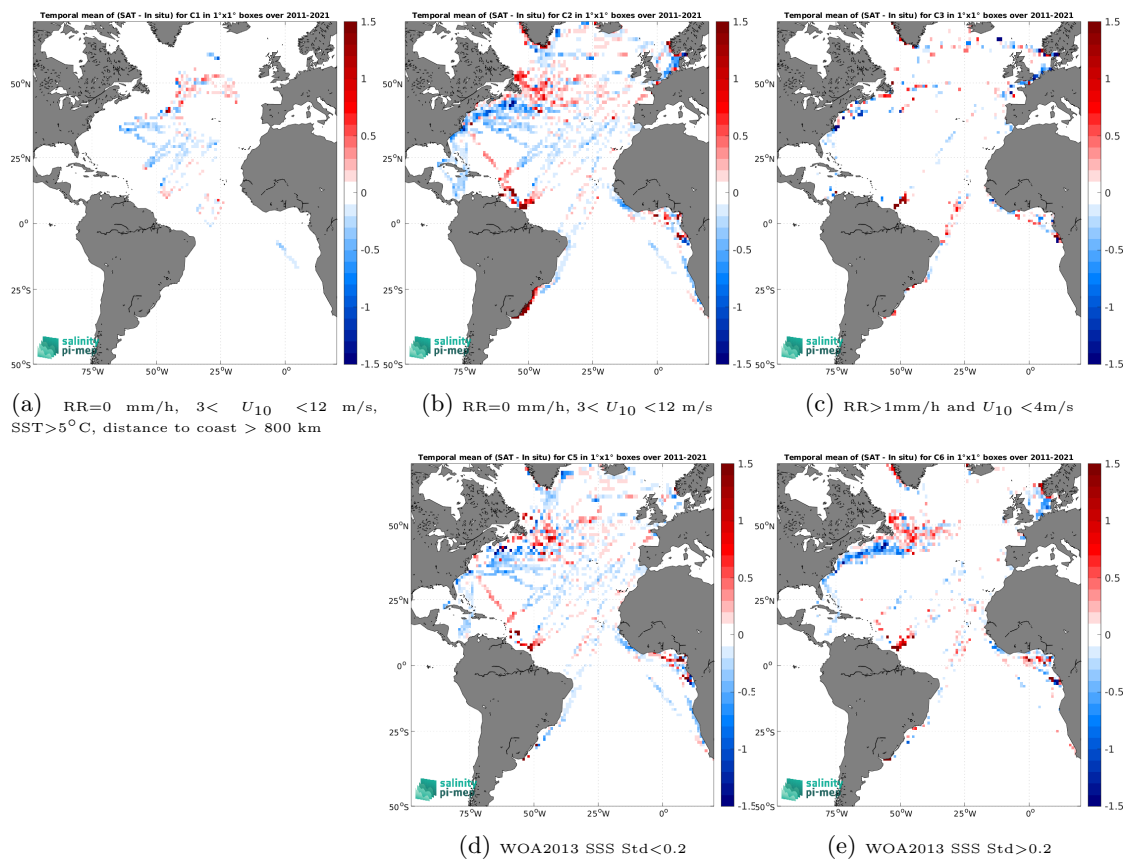
Figure 14: Temporal mean gridded over spatial boxes of size 1^\circ \times 1^\circ of \Delta\text{SSS} (SMOS SSS L4 v2 - Daily (BEC) - TSG (LEGOS-DM)) for 5 different subdatasets corresponding to:RR=0 mm/h, 3 < U_{10} < 12 m/s, SST >5^\circ\text{C} , distance to coast > 800 km (a), RR=0 mm/h, 3 < U_{10} < 12 m/s (b), RR >1 mm/h and U_{10} < 4 m/s (c), WOA2013 SSS Std <0.2 (d), WOA2013 SSS Std >0.2 (e).
