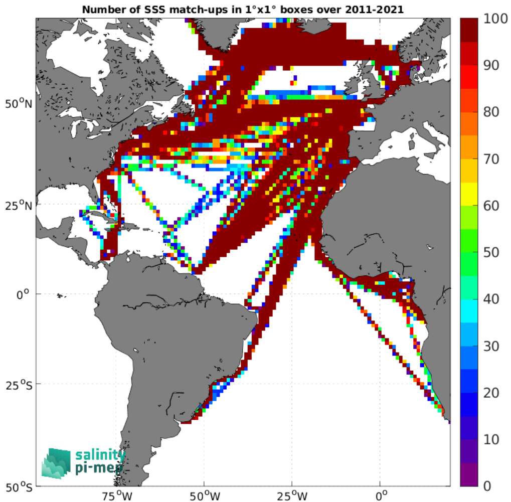
Figure 5: Number of SSS match-ups between TSG (LEGOS-DM) SSS and the SMOS SSS L4 v2 - Daily (BEC) SSS product for the Atlantic Ocean Pi-MEP region over 1°×1° boxes and for the full satellite product period.
