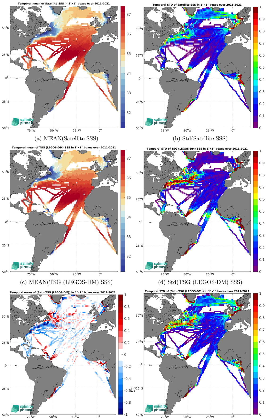
(e) MEAN( \Delta SSS) (Satellite - TSG (LEGOS-DM)) (f) Std( \Delta SSS) (Satellite - TSG (LEGOS-DM)) Figure 7: Temporal mean (left) and Std (right) of SSS from SMOS SSS L4 v2 - Daily (BEC) (top), TSG (LEGOS-DM) (middle), and of \Delta SSS (Satellite - TSG (LEGOS-DM)). Only match-pairs are used to generate these maps.
