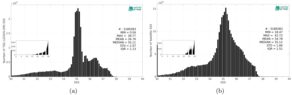
Figure 3: Histograms of SSS from TSG (LEGOS-DM) (a) and SMOS SSS L4 v2 - Daily (BEC) (b) considering all match-up pairs per bins of 0.1 over the Atlantic Ocean Pi-MEP region and for the full satellite product period.
