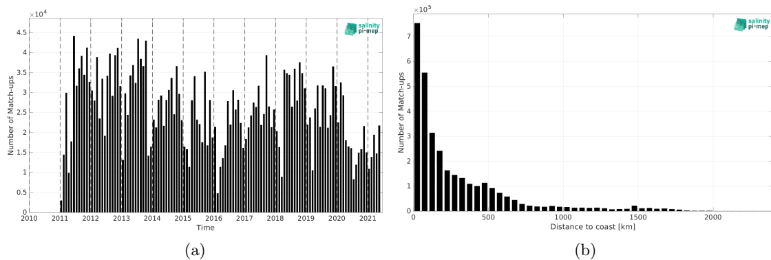
Figure 2: Number of match-ups between TSG (LEGOS-DM) and SMOS SSS L4 v2 - Daily (BEC) SSS as a function of time (a) and as function of the distance to coast (b) over the Atlantic Ocean Pi-MEP region and for the full satellite product period.
