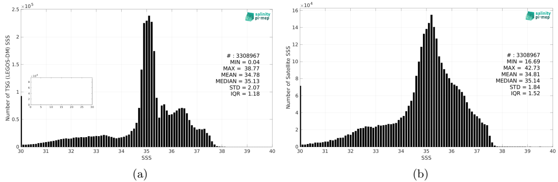
Figure 2: Histograms of SSS from TSG (LEGOS-DM) (a) and SMOS SSS L4 v2 - Daily (BEC) (b) considering all match-up pairs per bins of 0.1 over the Atlantic Ocean Pi-MEP region and for the full satellite product period.
