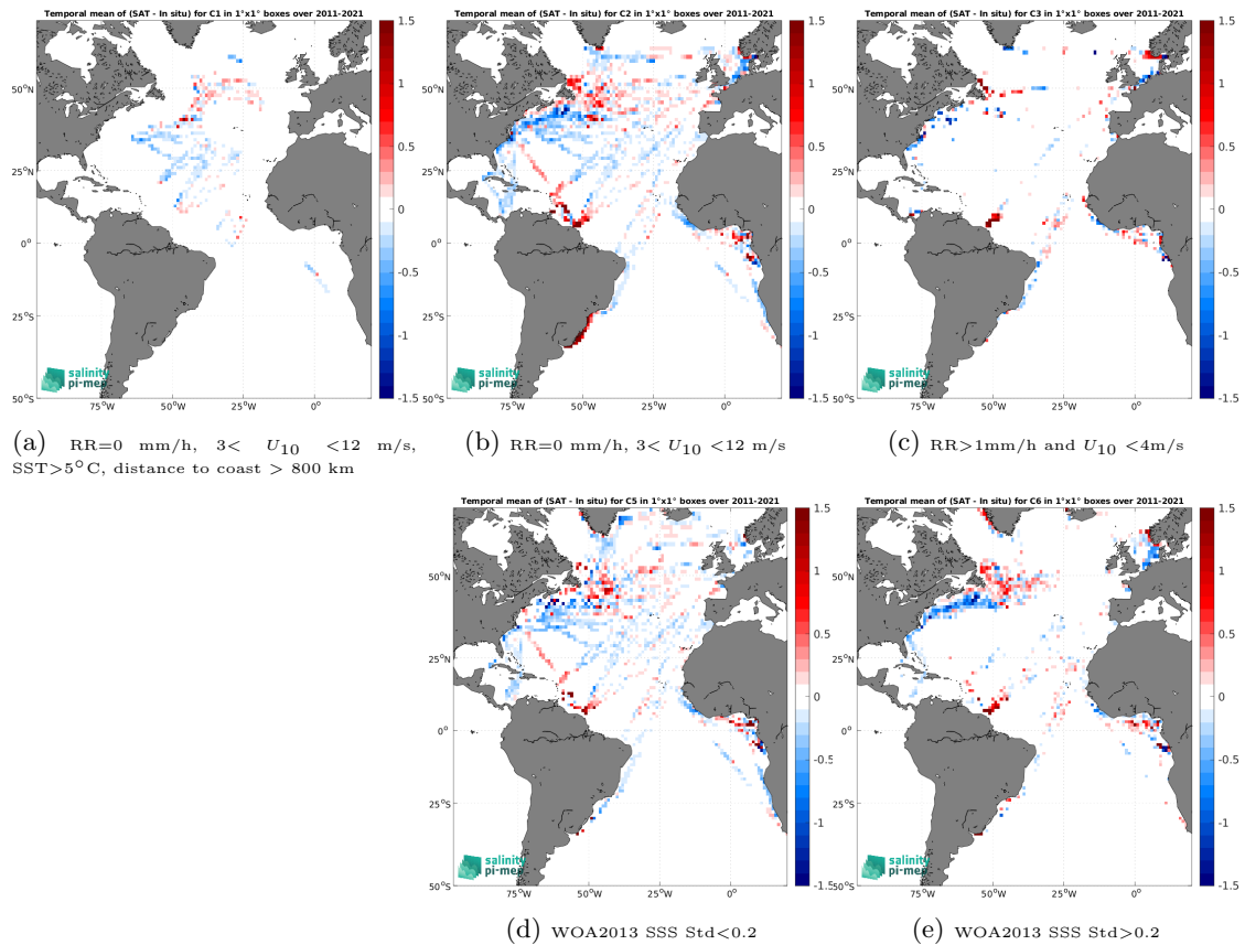
Figure 12: Temporal mean gridded over spatial boxes of size 1^\circ \times 1^\circ of \Delta SSS (SMOS SSS L4 v2 - Daily (BEC) - TSG (LEGOS-DM)) for 5 different subdatasets corresponding to:RR=0 mm/h, 3 < U_{10} < 12 m/s, SST >5^\circ\text{C} , distance to coast > 800 km (a), RR=0 mm/h, 3 < U_{10} < 12 m/s (b), RR >1 mm/h and U_{10} < 4 m/s (c), WOA2013 SSS Std <0.2 (d), WOA2013 SSS Std >0.2 (e).
