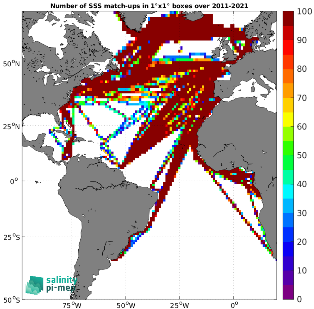
Figure 4: Number of SSS match-ups between TSG (LEGOS-DM) SSS and the SMOS SSS L4 v2 - Daily (BEC) SSS product for the Atlantic Ocean Pi-MEP region over 1^\circ \times 1^\circ boxes and for the full satellite product period.
