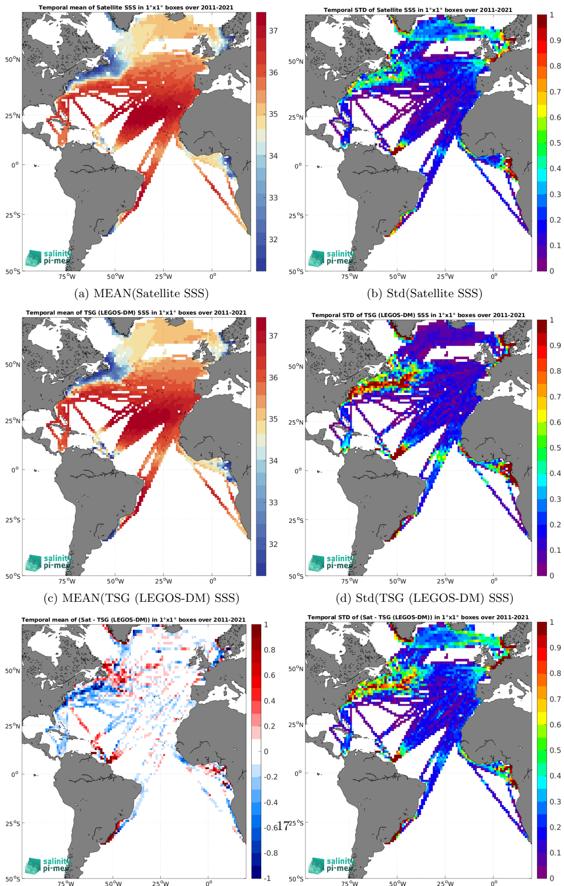
(e) MEAN( \Delta SSS) (Satellite - TSG (LEGOS-DM)) (f) Std( \Delta SSS) (Satellite - TSG (LEGOS-DM)) Figure 6: Temporal mean (left) and Std (right) of SSS from SMOS SSS L4 v2 - Daily (BEC) (top), TSG (LEGOS-DM) (middle), and of \Delta SSS (Satellite - TSG (LEGOS-DM)). Only match-pairs are used to generate these maps.
