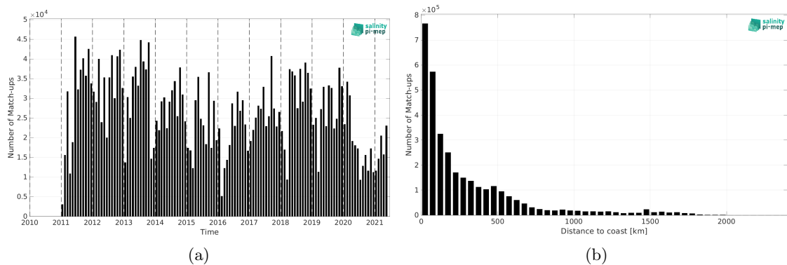
Figure 1: Number of match-ups between TSG (LEGOS-DM) and SMOS SSS L4 v2 - Daily (BEC) SSS as a function of time (a) and as function of the distance to coast (b) over the Atlantic Ocean Pi-MEP region and for the full satellite product period.
