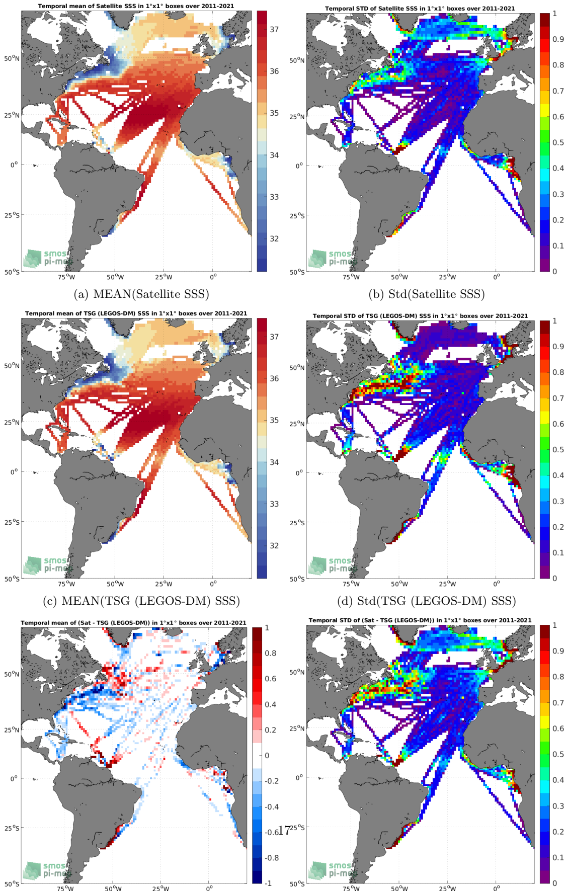
Figure 6: Temporal mean (left) and Std (right) of SSS from SMOS SSS L4 v2 - Daily (BEC) (top), TSG (LEGOS-DM) (middle), and of \Delta SSS (Satellite - TSG (LEGOS-DM)). Only match-up pairs are used to generate these maps.
