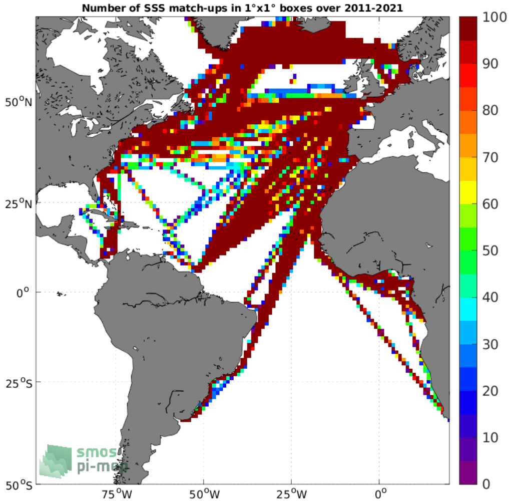
Figure 4: Number of SSS match-ups between TSG (LEGOS-DM) SSS and the SMOS SSS L4 v2 - Daily (BEC) SSS product for the Atlantic Ocean Pi-MEP region over 1°×1° boxes and for the full satellite product period.
