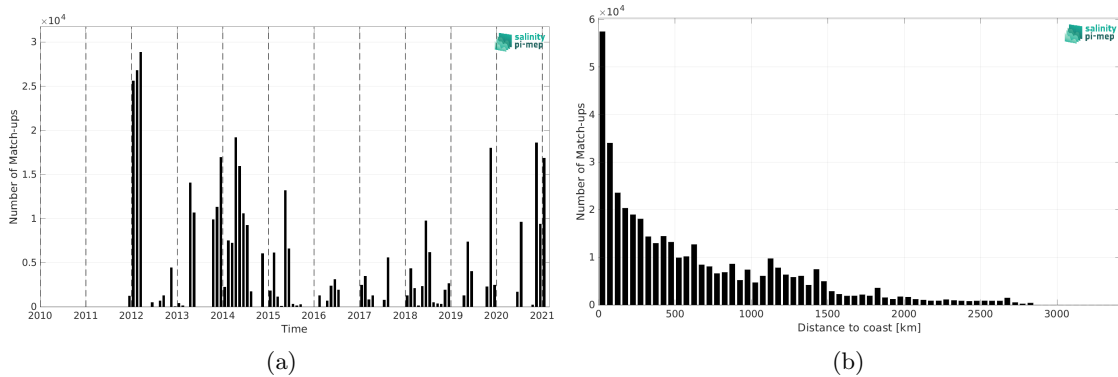
Figure 2: Number of match-ups between TSG (GOSUD-Sailing-ship) and SMOS SSS L4 v2 - Daily (BEC) SSS as a function of time (a) and as function of the distance to coast (b) over the Atlantic Ocean Pi-MEP region and for the full satellite product period.
