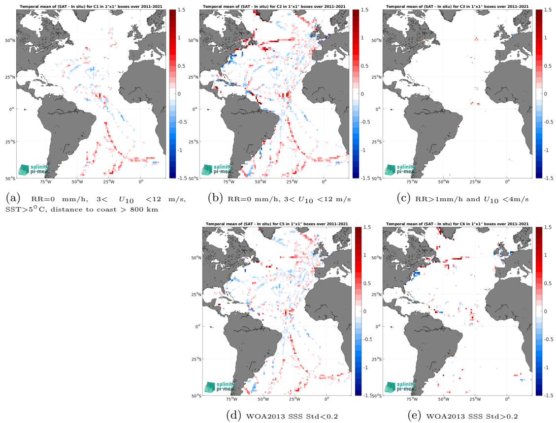
Figure 14: Temporal mean gridded over spatial boxes of size 1^\circ \times 1^\circ of \Delta\text{SSS} (SMOS SSS L4 v2 - Daily (BEC) - TSG (GOSUD-Sailing-ship)) for 5 different subdatasets corresponding to:RR=0 mm/h, 3 < U_{10} < 12 m/s, SST >5^\circ\text{C} , distance to coast > 800 km (a), RR=0 mm/h, 3 < U_{10} < 12 m/s (b), RR >1 mm/h and U_{10} < 4 m/s (c), WOA2013 SSS Std <0.2 (d), WOA2013 SSS Std >0.2 (e).
