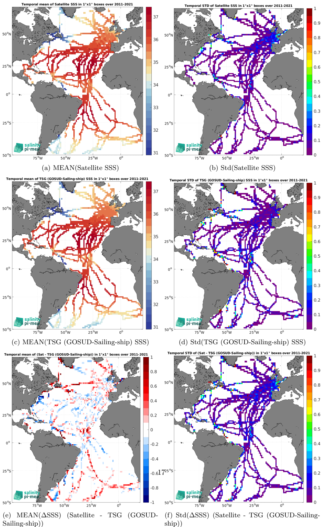
Figure 7: Temporal mean (left) and Std (right) of SSS from SMOS SSS L4 v2 - Daily (BEC) (top), TSG (GOSUD-Sailing-ship) (middle), and of \Delta SSS (Satellite - TSG (GOSUD-Sailing-ship)). Only match-up pairs are used to generate these maps.
