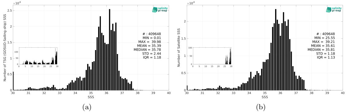
Figure 3: Histograms of SSS from TSG (GOSUD-Sailing-ship) (a) and SMOS SSS L4 v2 - Daily (BEC) (b) considering all match-up pairs per bins of 0.1 over the Atlantic Ocean Pi-MEP region and for the full satellite product period.
