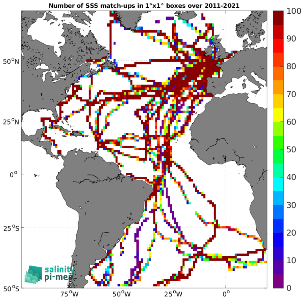
Figure 5: Number of SSS match-ups between TSG (GOSUD-Sailing-ship) SSS and the SMOS SSS L4 v2 - Daily (BEC) SSS product for the Atlantic Ocean Pi-MEP region over 1^\circ \times 1^\circ boxes and for the full satellite product period.
