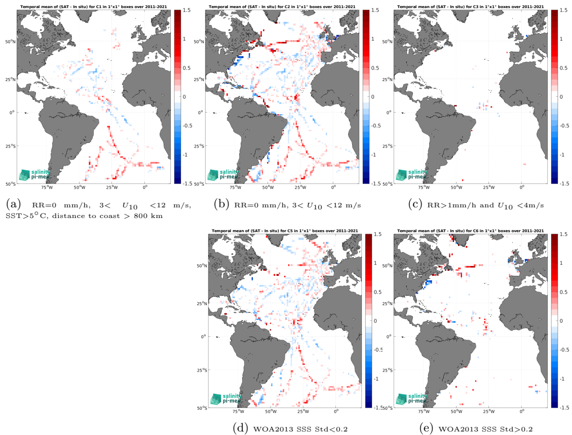
Figure 12: Temporal mean gridded over spatial boxes of size 1^\circ \times 1^\circ of \Delta\text{SSS} (SMOS SSS L4 v2 - Daily (BEC) - TSG (GOSUD-Sailing-ship)) for 5 different subdatasets corresponding to:RR=0 mm/h, 3 < U_{10} < 12 m/s, SST >5^\circ\text{C} , distance to coast > 800 km (a), RR=0 mm/h, 3 < U_{10} < 12 m/s (b), RR >1 mm/h and U_{10} < 4 m/s (c), WOA2013 SSS Std <0.2 (d), WOA2013 SSS Std >0.2 (e).
