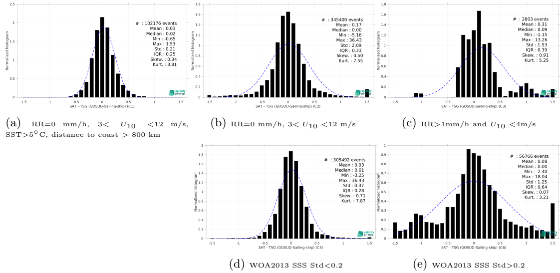
Figure 13: Normalized histogram of \Delta\text{SSS} (SMOS SSS L4 v2 - Daily (BEC) - TSG (GOSUD-Sailing-ship)) for 5 different subdatasets corresponding to: RR=0 mm/h, 3 < U_{10} < 12 m/s, SST>5°C, distance to coast > 800 km (a), RR=0 mm/h, 3 < U_{10} < 12 m/s (b), RR>1mm/h and U_{10} < 4 m/s (c), WOA2013 SSS Std<0.2 (d), WOA2013 SSS Std>0.2 (e).
