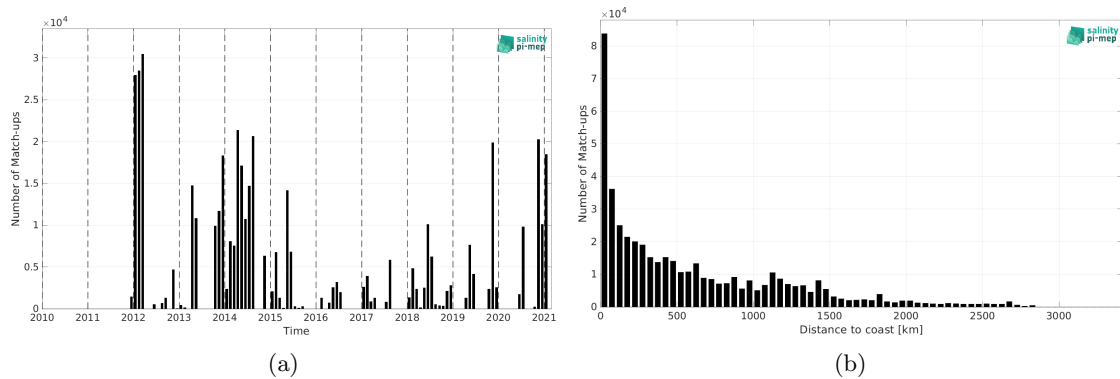
Figure 1: Number of match-ups between TSG (GOSUD-Sailing-ship) and SMOS SSS L4 v2 - Daily (BEC) SSS as a function of time (a) and as function of the distance to coast (b) over the Atlantic Ocean Pi-MEP region and for the full satellite product period.
