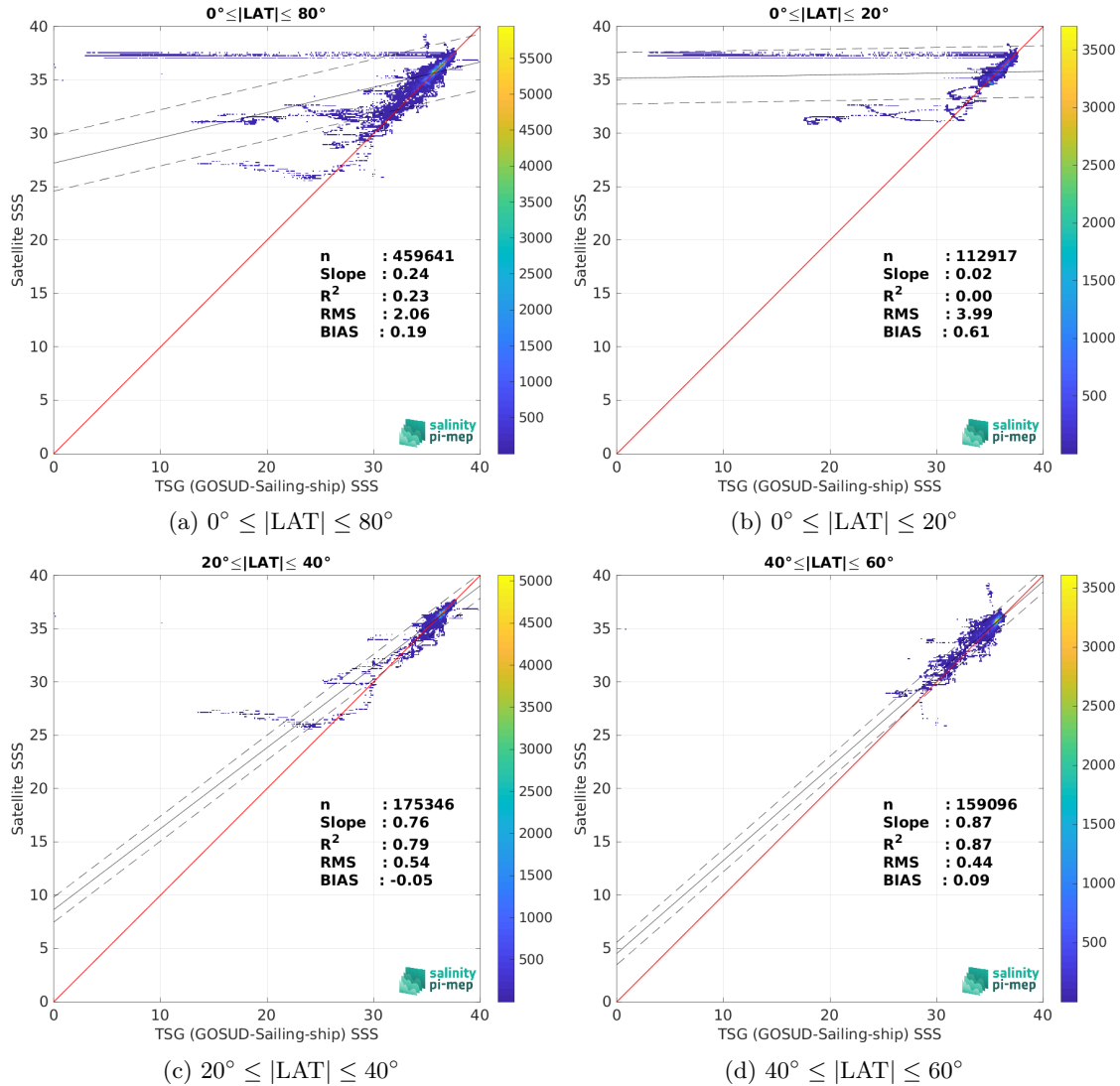
Figure 9: Contour maps of the concentration of SMOS SSS L4 v2 - Daily (BEC) SSS (y-axis) versus TSG (GOSUD-Sailing-ship) SSS (x-axis) at match-up pairs for different latitude bands. For each plot, the red line shows x=y . The black thin and dashed lines indicate a linear fit through the data cloud and the \pm 95\% confidence levels, respectively. The number of match-up pairs n , the slope and R^2 coefficient of the linear fit, the root mean square (RMS) and the mean bias between satellite and in situ data are indicated for each latitude band in each plot.
