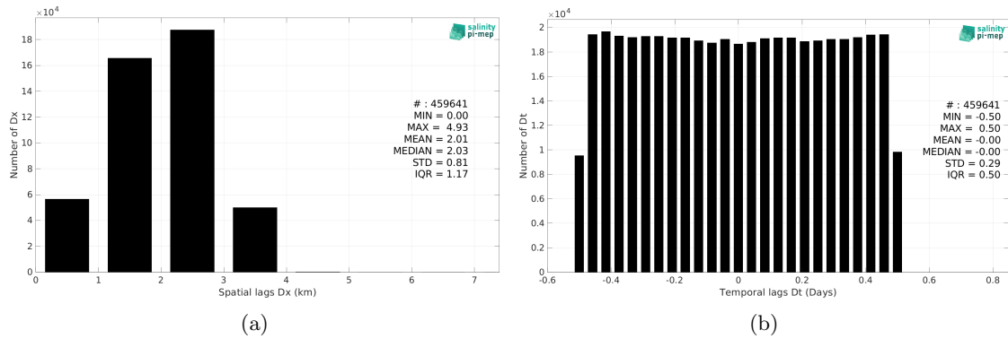
Figure 5: Histograms of the spatial (a) and temporal (b) lags between the location/time of the TSG (GOSUD-Sailing-ship) measurement and the date of the corresponding SMOS SSS L4 v2 - Daily (BEC) SSS pixel.
