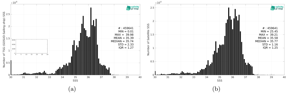
Figure 2: Histograms of SSS from TSG (GOSUD-Sailing-ship) (a) and SMOS SSS L4 v2 - Daily (BEC) (b) considering all match-up pairs per bins of 0.1 over the Atlantic Ocean Pi-MEP region and for the full satellite product period.
