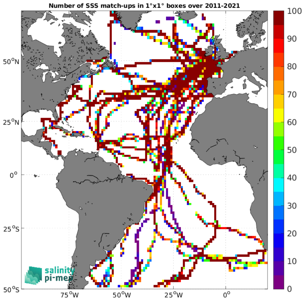
Figure 4: Number of SSS match-ups between TSG (GOSUD-Sailing-ship) SSS and the SMOS SSS L4 v2 - Daily (BEC) SSS product for the Atlantic Ocean Pi-MEP region over 1^\circ \times 1^\circ boxes and for the full satellite product period.
