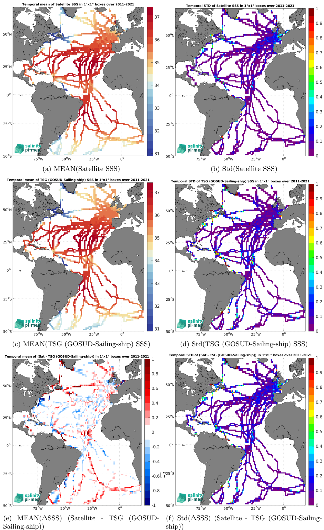
Figure 6: Temporal mean (left) and Std (right) of SSS from SMOS SSS L4 v2 - Daily (BEC) (top), TSG (GOSUD-Sailing-ship) (middle), and of \Delta SSS (Satellite - TSG (GOSUD-Sailing-ship)). Only match-up pairs are used to generate these maps.
