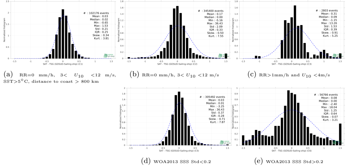
Figure 13: Normalized histogram of \Delta\text{SSS} (SMOS SSS L4 v2 - Daily (BEC) - TSG (GOSUD-Sailing-ship)) for 5 different subdatasets corresponding to: RR=0 mm/h, 3 < U_{10} < 12 m/s, SST>5°C, distance to coast > 800 km (a), RR=0 mm/h, 3 < U_{10} < 12 m/s (b), RR>1mm/h and U_{10} < 4 m/s (c), WOA2013 SSS Std<0.2 (d), WOA2013 SSS Std>0.2 (e).
