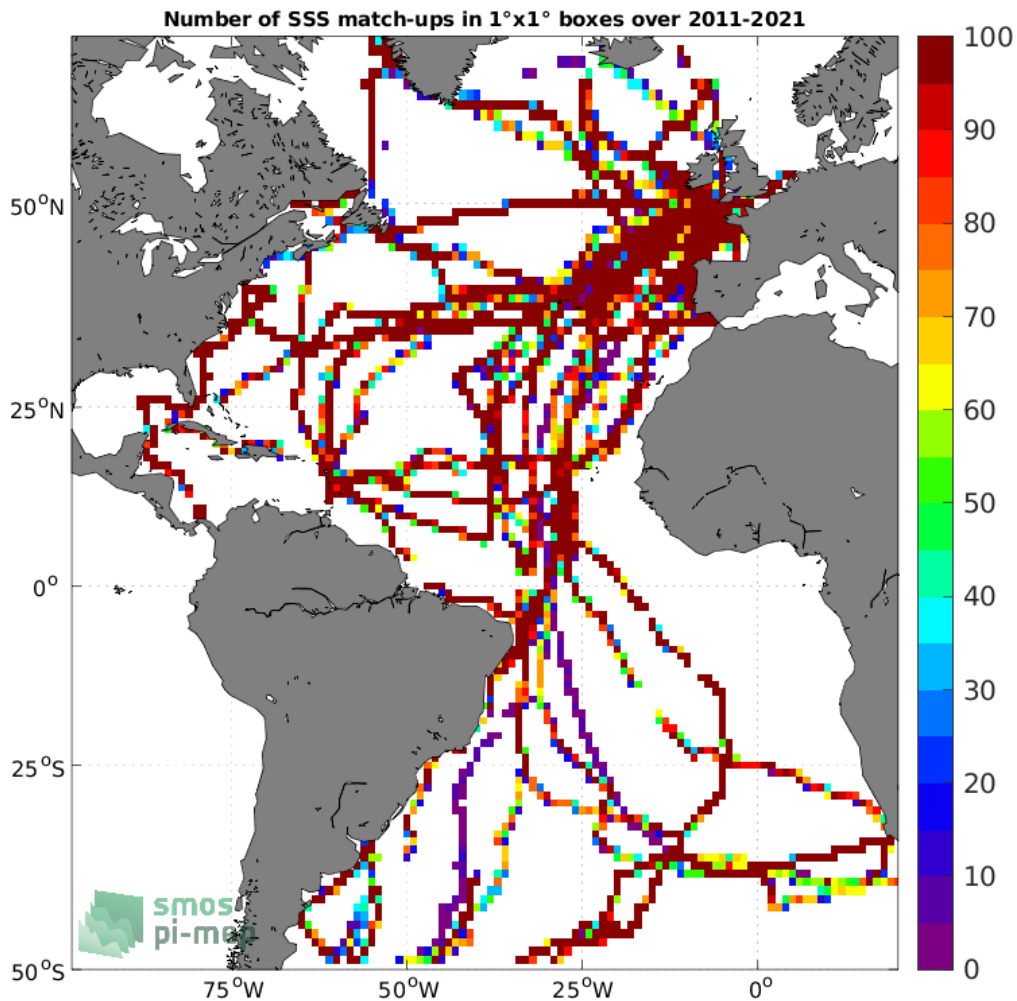
Figure 4: Number of SSS match-ups between TSG (GOSUD-Sailing-ship) SSS and the SMOS SSS L4 v2 - Daily (BEC) SSS product for the Atlantic Ocean Pi-MEP region over 1°×1° boxes and for the full satellite product period.
