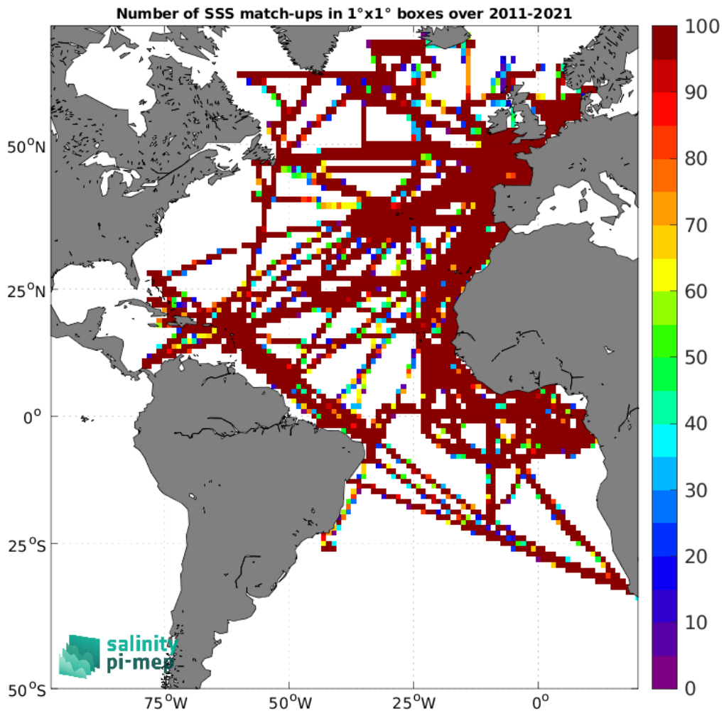
Figure 5: Number of SSS match-ups between TSG (GOSUD-Research-vessel) SSS and the SMOS SSS L4 v2 - Daily (BEC) SSS product for the Atlantic Ocean Pi-MEP region over 1°×1° boxes and for the full satellite product period.
