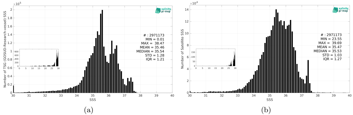
Figure 3: Histograms of SSS from TSG (GOSUD-Research-vessel) (a) and SMOS SSS L4 v2 - Daily (BEC) (b) considering all match-up pairs per bins of 0.1 over the Atlantic Ocean Pi-MEP region and for the full satellite product period.
