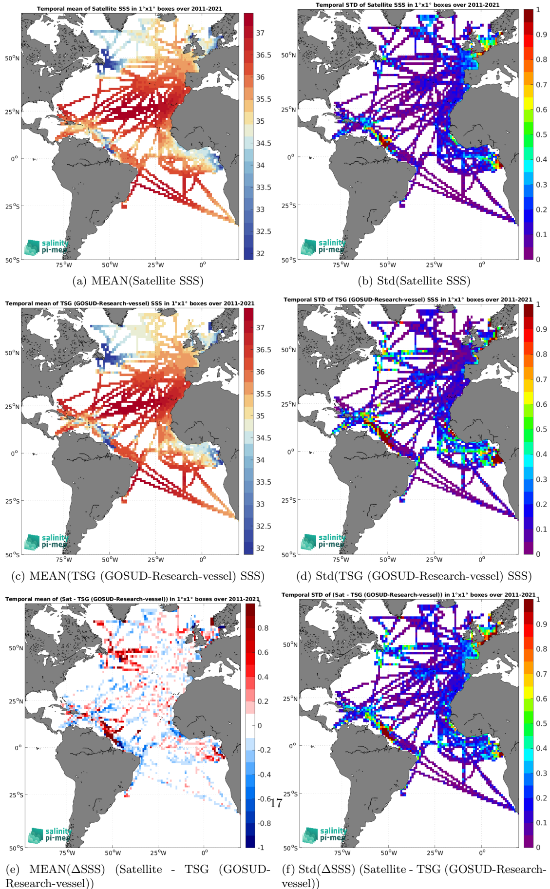
Figure 7: Temporal mean (left) and Std (right) of SSS from SMOS SSS L4 v2 - Daily (BEC) (top), TSG (GOSUD-Research-vessel) (middle), and of \Delta SSS (Satellite - TSG (GOSUD-Research-vessel)). Only match-up pairs are used to generate these maps.
