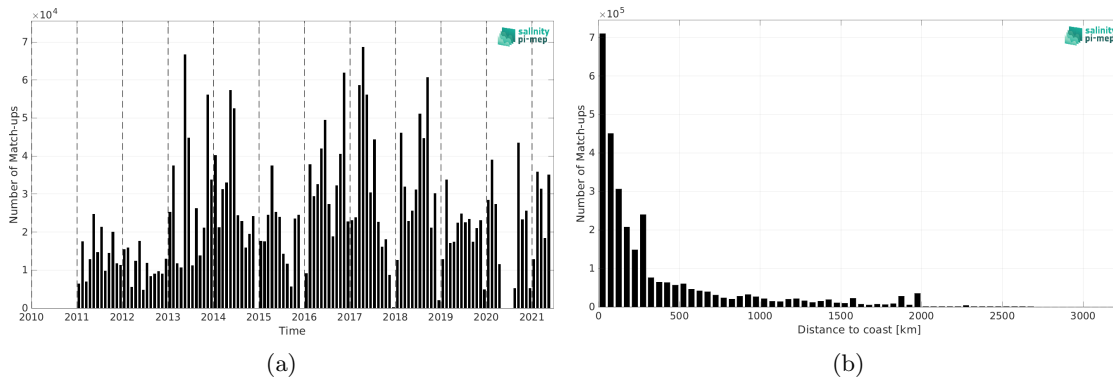
Figure 2: Number of match-ups between TSG (GOSUD-Research-vessel) and SMOS SSS L4 v2 - Daily (BEC) SSS as a function of time (a) and as function of the distance to coast (b) over the Atlantic Ocean Pi-MEP region and for the full satellite product period.
