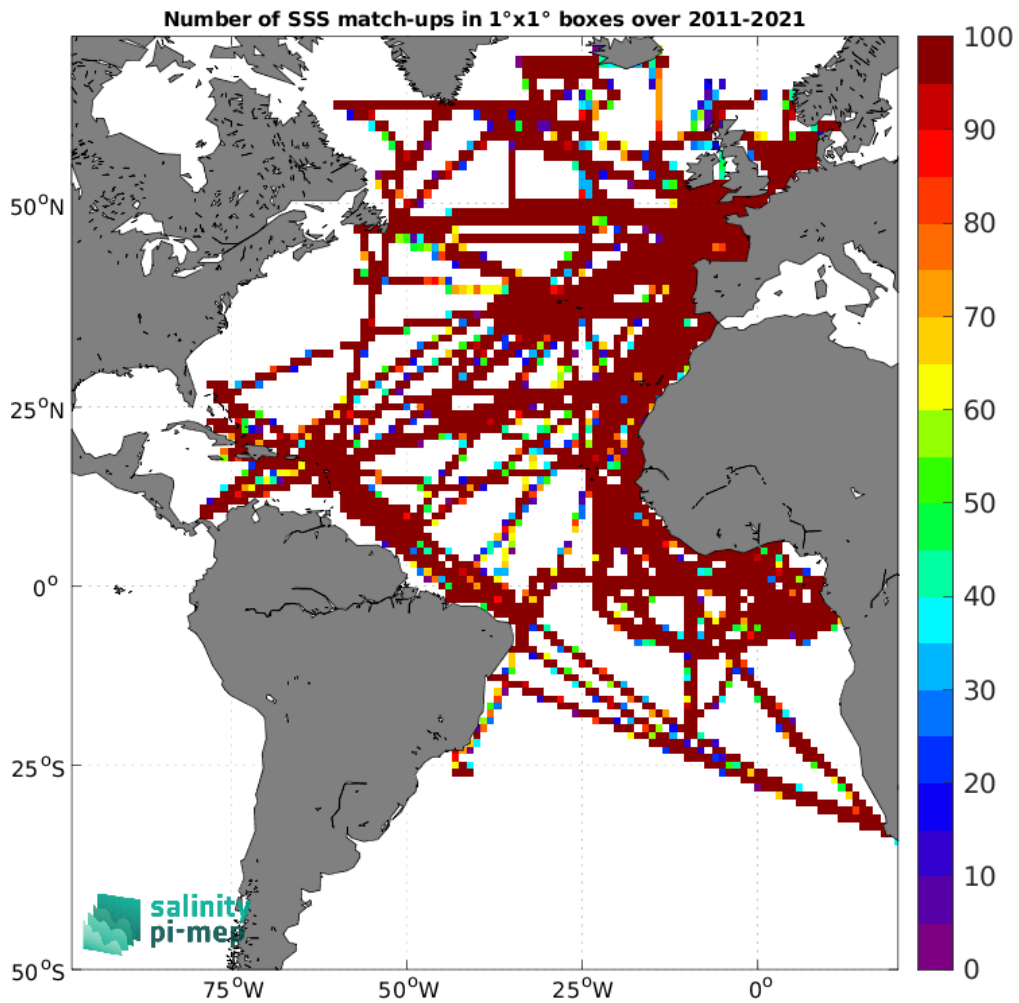
Figure 5: Number of SSS match-ups between TSG (GOSUD-Research-vessel) SSS and the SMOS SSS L4 v2 - Daily (BEC) SSS product for the Atlantic Ocean Pi-MEP region over 1^\circ \times 1^\circ boxes and for the full satellite product period.
