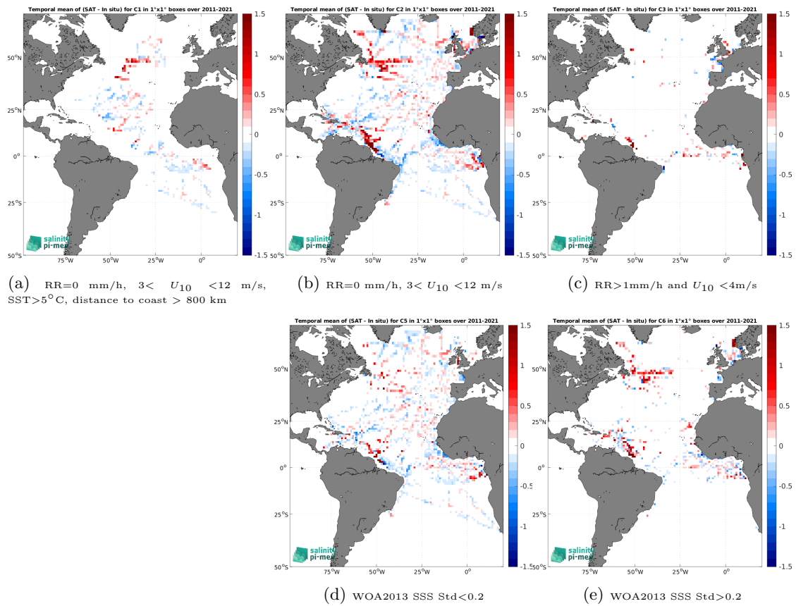
Figure 14: Temporal mean gridded over spatial boxes of size 1^\circ \times 1^\circ of \Delta\text{SSS} (SMOS SSS L4 v2 - Daily (BEC) - TSG (GOSUD-Research-vessel)) for 5 different subdatasets corresponding to:RR=0 mm/h, 3 < U_{10} < 12 m/s, SST>5°C, distance to coast > 800 km (a), RR=0 mm/h, 3 < U_{10} < 12 m/s (b), RR>1mm/h and U_{10} < 4 m/s (c), WOA2013 SSS Std<0.2 (d), WOA2013 SSS Std>0.2 (e).
