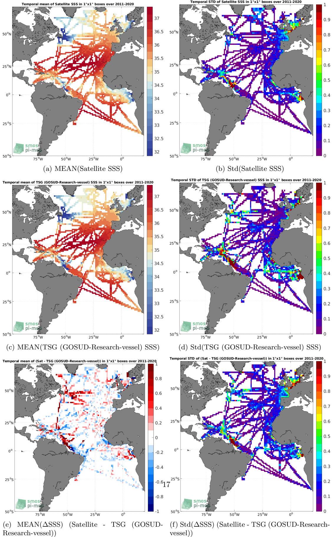
Figure 6: Temporal mean (left) and Std (right) of SSS from SMOS SSS L4 v2 - Daily (BEC) (top), TSG (GOSUD-Research-vessel) (middle), and of \Delta SSS (Satellite - TSG (GOSUD-Research-vessel)). Only match-up pairs are used to generate these maps.
