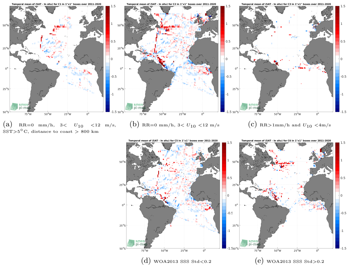
Figure 12: Temporal mean gridded over spatial boxes of size 1^\circ \times 1^\circ of \Delta\text{SSS} (SMOS SSS L4 v2 - Daily (BEC) - TSG (GOSUD-Research-vessel)) for 5 different subdatasets corresponding to:RR=0 mm/h, 3 < U_{10} < 12 m/s, SST>5°C, distance to coast > 800 km (a), RR=0 mm/h, 3 < U_{10} < 12 m/s (b), RR>1mm/h and U_{10} < 4 m/s (c), WOA2013 SSS Std<0.2 (d), WOA2013 SSS Std>0.2 (e).
