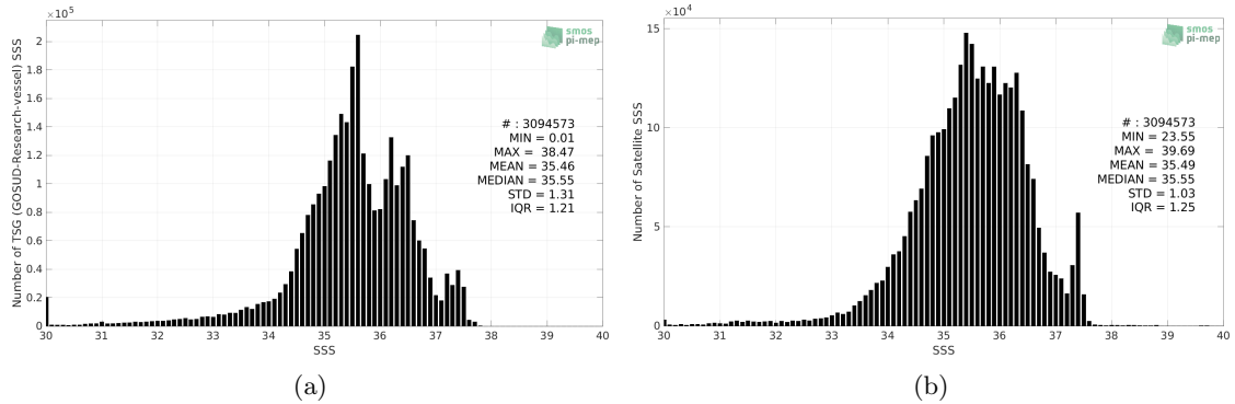
Figure 2: Histograms of SSS from TSG (GOSUD-Research-vessel) (a) and SMOS SSS L4 v2 - Daily (BEC) (b) considering all match-up pairs per bins of 0.1 over the Atlantic Ocean Pi-MEP region and for the full satellite product period.
