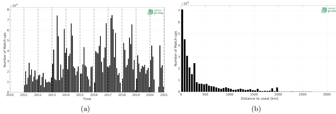
Figure 1: Number of match-ups between TSG (GOSUD-Research-vessel) and SMOS SSS L4 v2 - Daily (BEC) SSS as a function of time (a) and as function of the distance to coast (b) over the Atlantic Ocean Pi-MEP region and for the full satellite product period.
