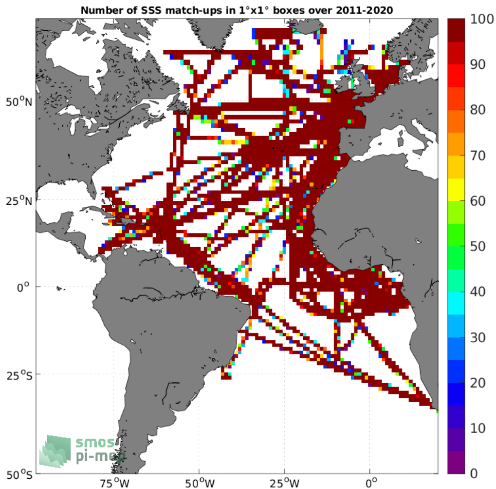
Figure 4: Number of SSS match-ups between TSG (GOSUD-Research-vessel) SSS and the SMOS SSS L4 v2 - Daily (BEC) SSS product for the Atlantic Ocean Pi-MEP region over 1^\circ \times 1^\circ boxes and for the full satellite product period.
