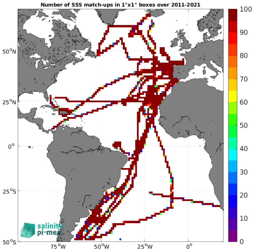
Figure 5: Number of SSS match-ups between TSG (CSIC-UTM) SSS and the SMOS SSS L4 v2 - Daily (BEC) SSS product for the Atlantic Ocean Pi-MEP region over 1^\circ \times 1^\circ boxes and for the full satellite product period.
