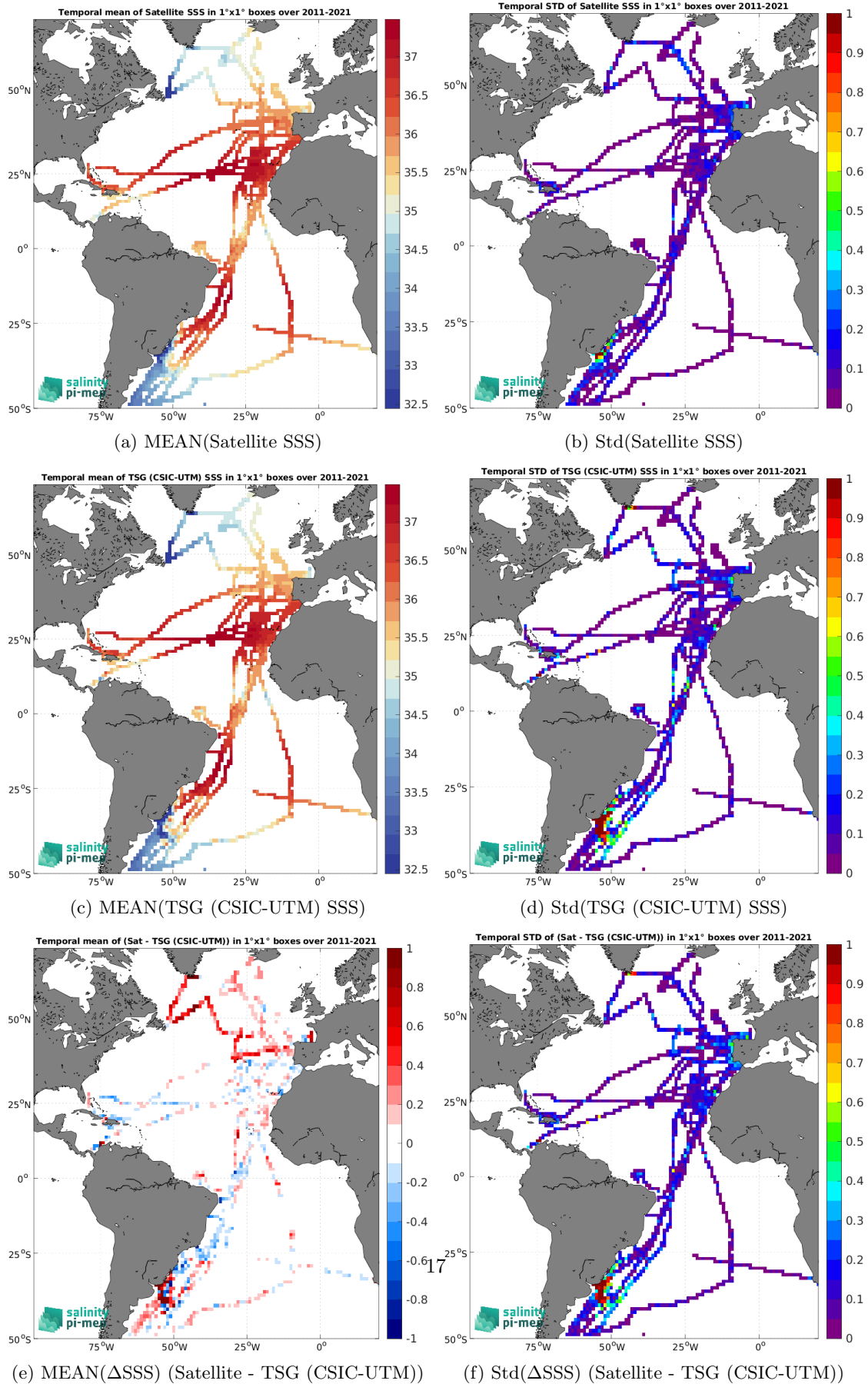
Figure 7: Temporal mean (left) and Std (right) of SSS from SMOS SSS L4 v2 - Daily (BEC) (top), TSG (CSIC-UTM) (middle), and of \Delta SSS (Satellite - TSG (CSIC-UTM)). Only match-up pairs are used to generate these maps.
