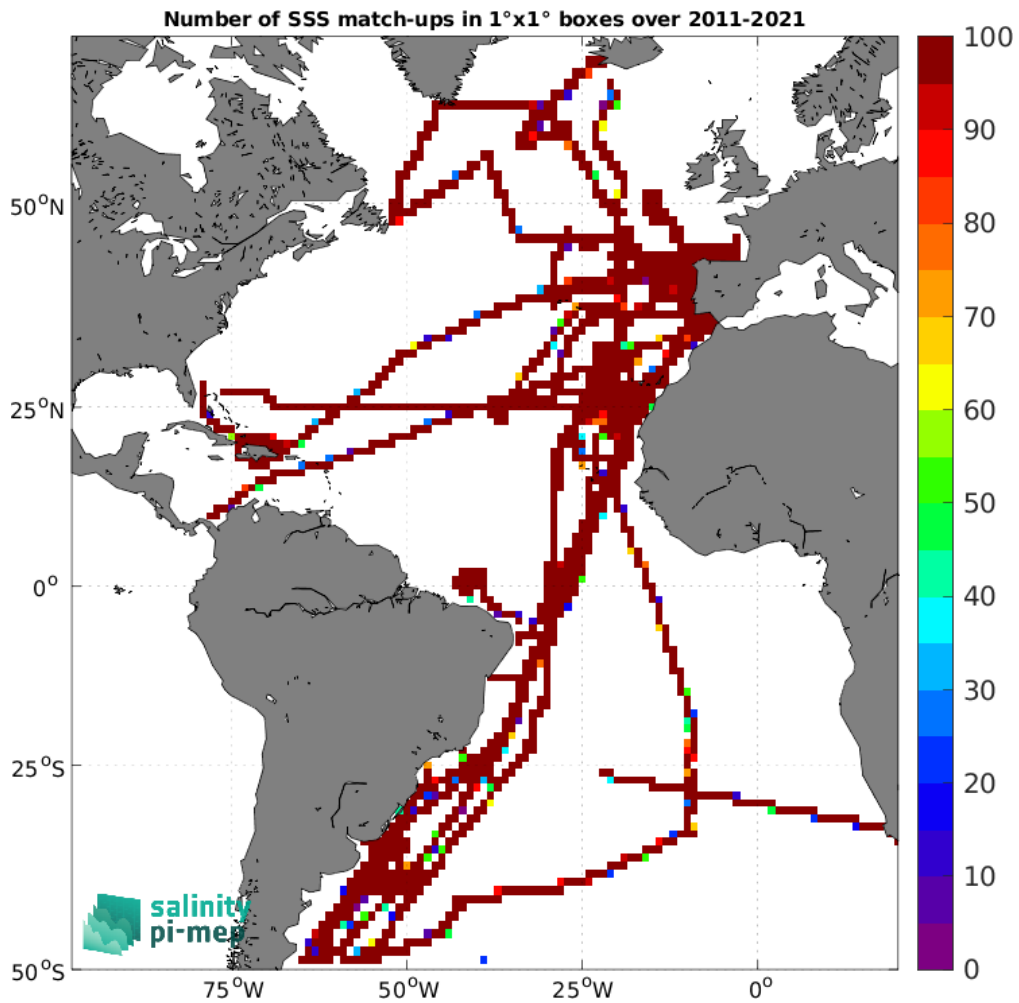
Figure 5: Number of SSS match-ups between TSG (CSIC-UTM) SSS and the SMOS SSS L4 v2 - Daily (BEC) SSS product for the Atlantic Ocean Pi-MEP region over 1°×1° boxes and for the full satellite product period.
