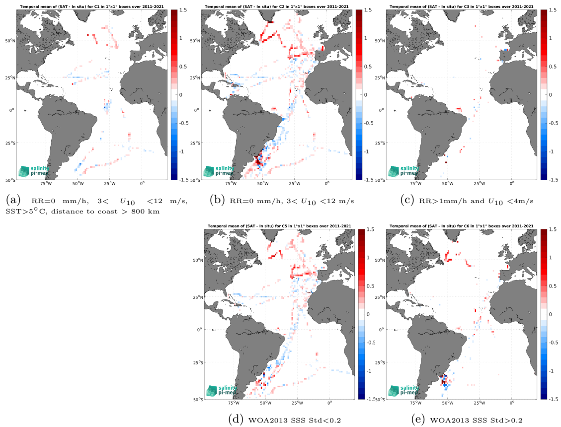
Figure 14: Temporal mean gridded over spatial boxes of size 1^\circ \times 1^\circ of \Delta\text{SSS} (SMOS SSS L4 v2 - Daily (BEC) - TSG (CSIC-UTM)) for 5 different subdatasets corresponding to:RR=0 mm/h, 3 < U_{10} < 12 m/s, SST>5°C, distance to coast > 800 km (a), RR=0 mm/h, 3 < U_{10} < 12 m/s (b), RR>1mm/h and U_{10} < 4 m/s (c), WOA2013 SSS Std<0.2 (d), WOA2013 SSS Std>0.2 (e).
