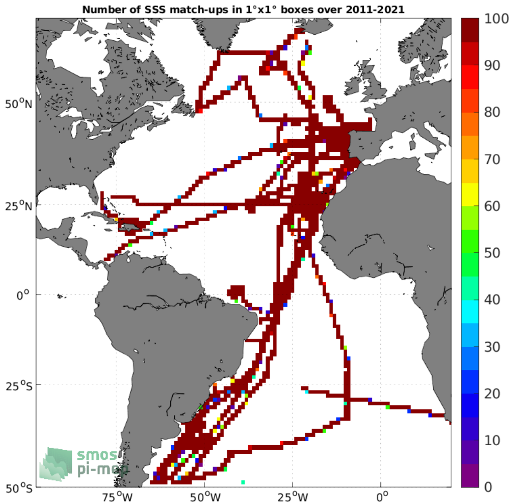
Figure 4: Number of SSS match-ups between TSG (CSIC-UTM) SSS and the SMOS SSS L4 v2 - Daily (BEC) SSS product for the Atlantic Ocean Pi-MEP region over 1°×1° boxes and for the full satellite product period.
