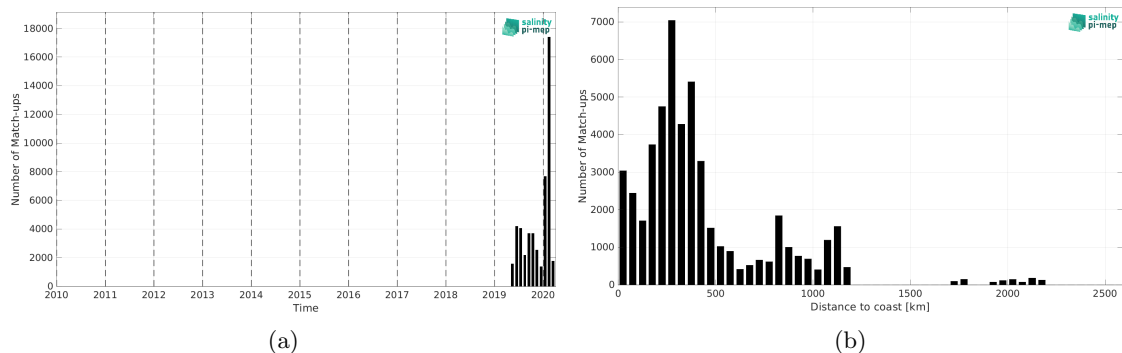
Figure 2: Number of match-ups between Saildrone and SMOS SSS L4 v2 - Daily (BEC) SSS as a function of time (a) and as function of the distance to coast (b) over the Atlantic Ocean Pi-MEP region and for the full satellite product period.
