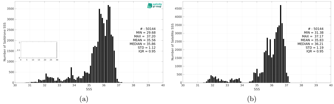
Figure 3: Histograms of SSS from Saildrone (a) and SMOS SSS L4 v2 - Daily (BEC) (b) considering all match-up pairs per bins of 0.1 over the Atlantic Ocean Pi-MEP region and for the full satellite product period.
