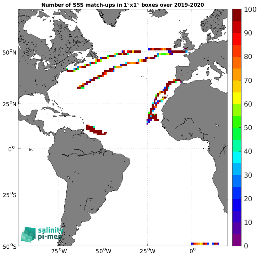
Figure 5: Number of SSS match-ups between Saildrone SSS and the SMOS SSS L4 v2 - Daily (BEC) SSS product for the Atlantic Ocean Pi-MEP region over 1°×1° boxes and for the full satellite product period.
