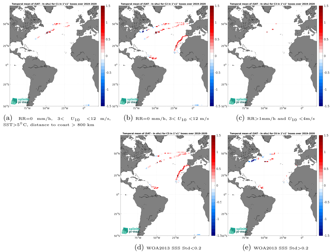
Figure 14: Temporal mean gridded over spatial boxes of size 1^\circ \times 1^\circ of \Delta SSS (SMOS SSS L4 v2 - Daily (BEC) - Saicdrone) for 5 different subdatasets corresponding to:RR=0 mm/h, 3 < U_{10} < 12 m/s, SST >5^\circ\text{C} , distance to coast > 800 km (a), RR=0 mm/h, 3 < U_{10} < 12 m/s (b), RR >1 mm/h and U_{10} < 4 m/s (c), WOA2013 SSS Std <0.2 (d), WOA2013 SSS Std >0.2 (e).
