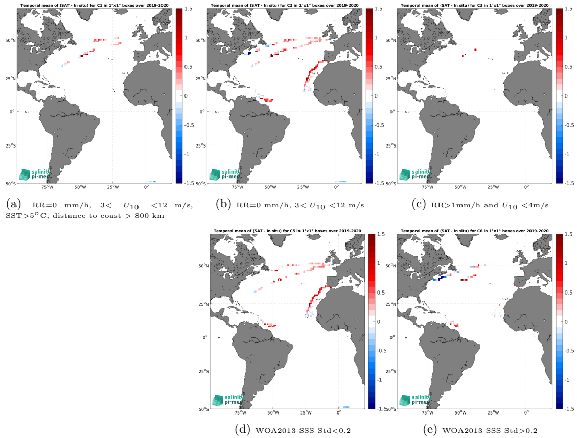
Figure 12: Temporal mean gridded over spatial boxes of size 1^\circ \times 1^\circ of \Delta SSS (SMOS SSS L4 v2 - Daily (BEC) - Saicdrone) for 5 different subdatasets corresponding to:RR=0 mm/h, 3 < U_{10} < 12 m/s, SST >5^\circ\text{C} , distance to coast > 800 km (a), RR=0 mm/h, 3 < U_{10} < 12 m/s (b), RR >1 mm/h and U_{10} < 4 m/s (c), WOA2013 SSS Std <0.2 (d), WOA2013 SSS Std >0.2 (e).
