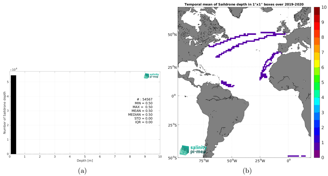
Figure 3: Histograms of the depth of the upper level SSS measurements from Sairdron in the Match-up DataBase for the Atlantic Ocean Pi-MEP region (a) and temporal mean spatial distribution of pressure of the in situ SSS data over 1^\circ \times 1^\circ boxes and for the full satellite product period (b).
