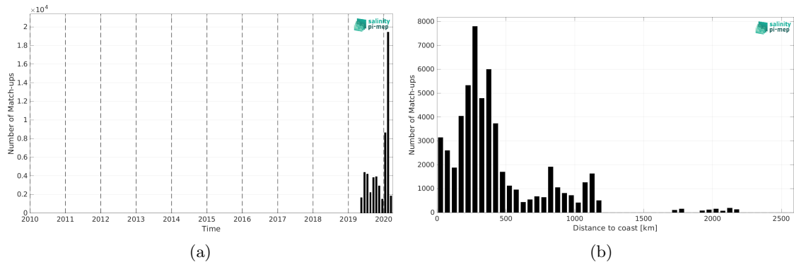
Figure 1: Number of match-ups between Saildrone and SMOS SSS L4 v2 - Daily (BEC) SSS as a function of time (a) and as function of the distance to coast (b) over the Atlantic Ocean Pi-MEP region and for the full satellite product period.
