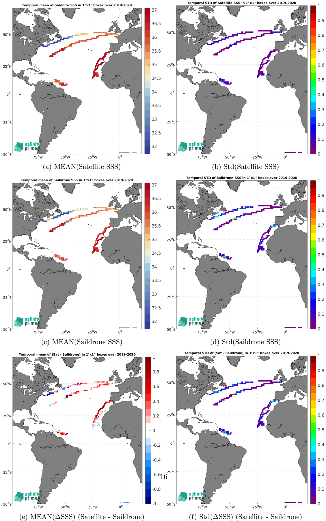
Figure 6: Temporal mean (left) and Std (right) of SSS from SMOS SSS L4 v2 - Daily (BEC) (top), Saildrone (middle), and of \Delta SSS (Satellite - Saildrone). Only match-up pairs are used to generate these maps.
