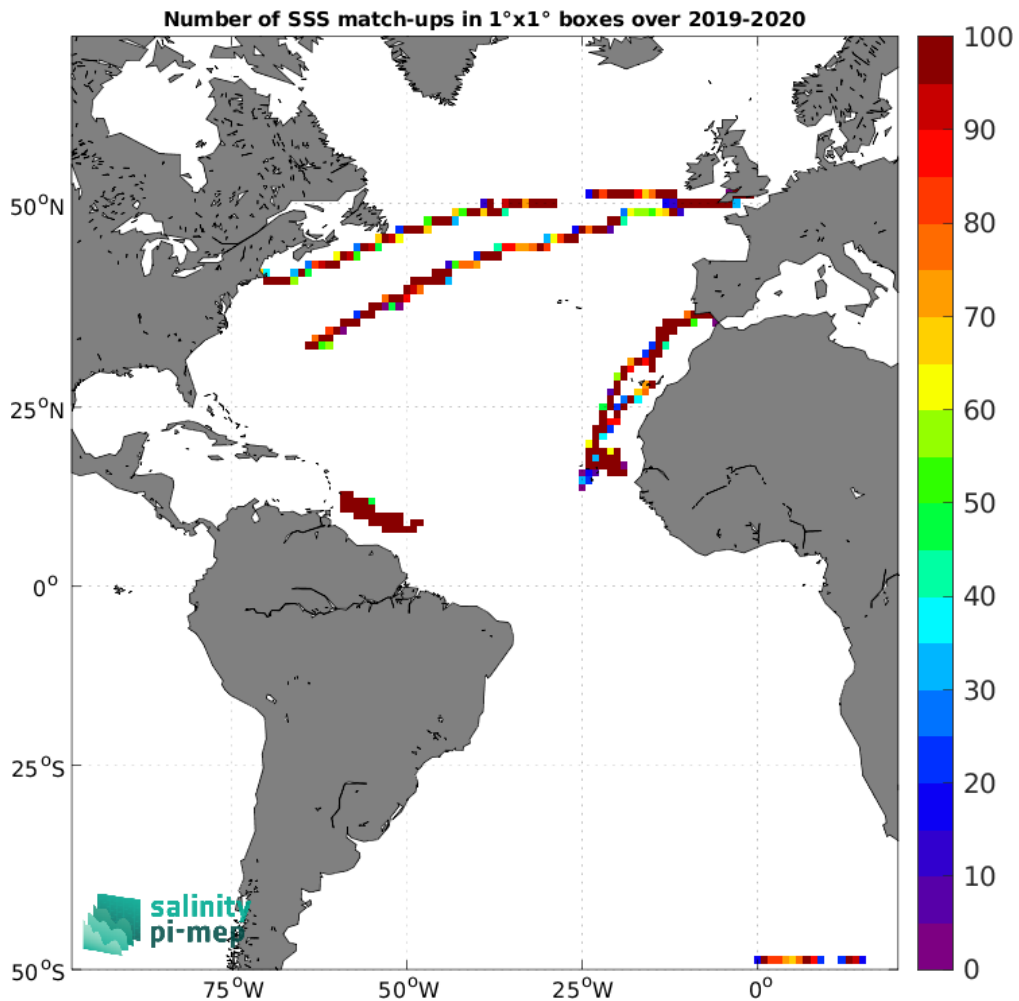
Figure 4: Number of SSS match-ups between Saildrone SSS and the SMOS SSS L4 v2 - Daily (BEC) SSS product for the Atlantic Ocean Pi-MEP region over 1°×1° boxes and for the full satellite product period.
