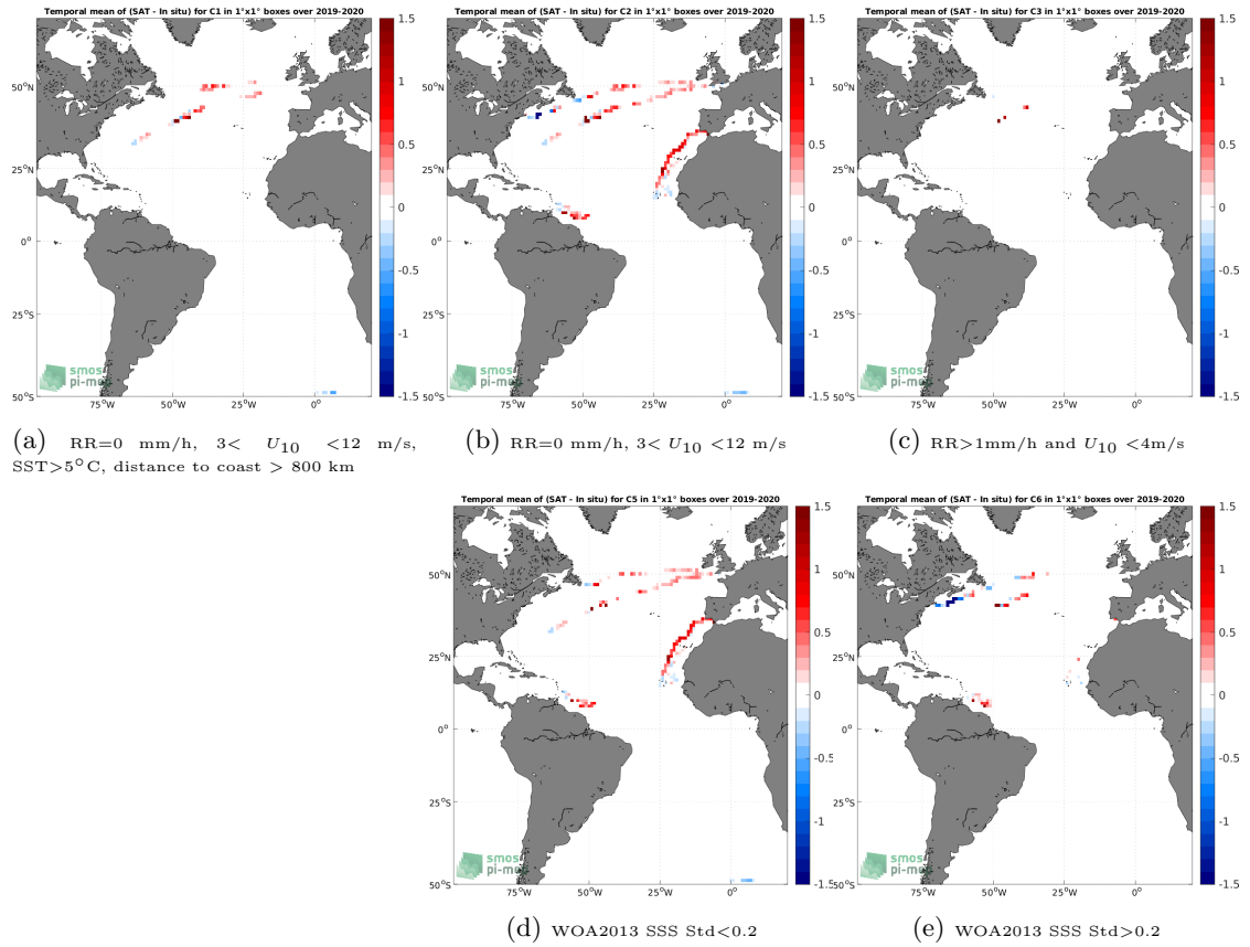
Figure 12: Temporal mean gridded over spatial boxes of size 1^\circ \times 1^\circ of \Delta SSS (SMOS SSS L4 v2 - Daily (BEC) - Saldrone) for 5 different subdatasets corresponding to:RR=0 mm/h, 3 < U_{10} < 12 m/s, SST>5°C, distance to coast > 800 km (a), RR=0 mm/h, 3 < U_{10} < 12 m/s (b), RR>1mm/h and U_{10} < 4 m/s (c), WOA2013 SSS Std<0.2 (d), WOA2013 SSS Std>0.2 (e).
