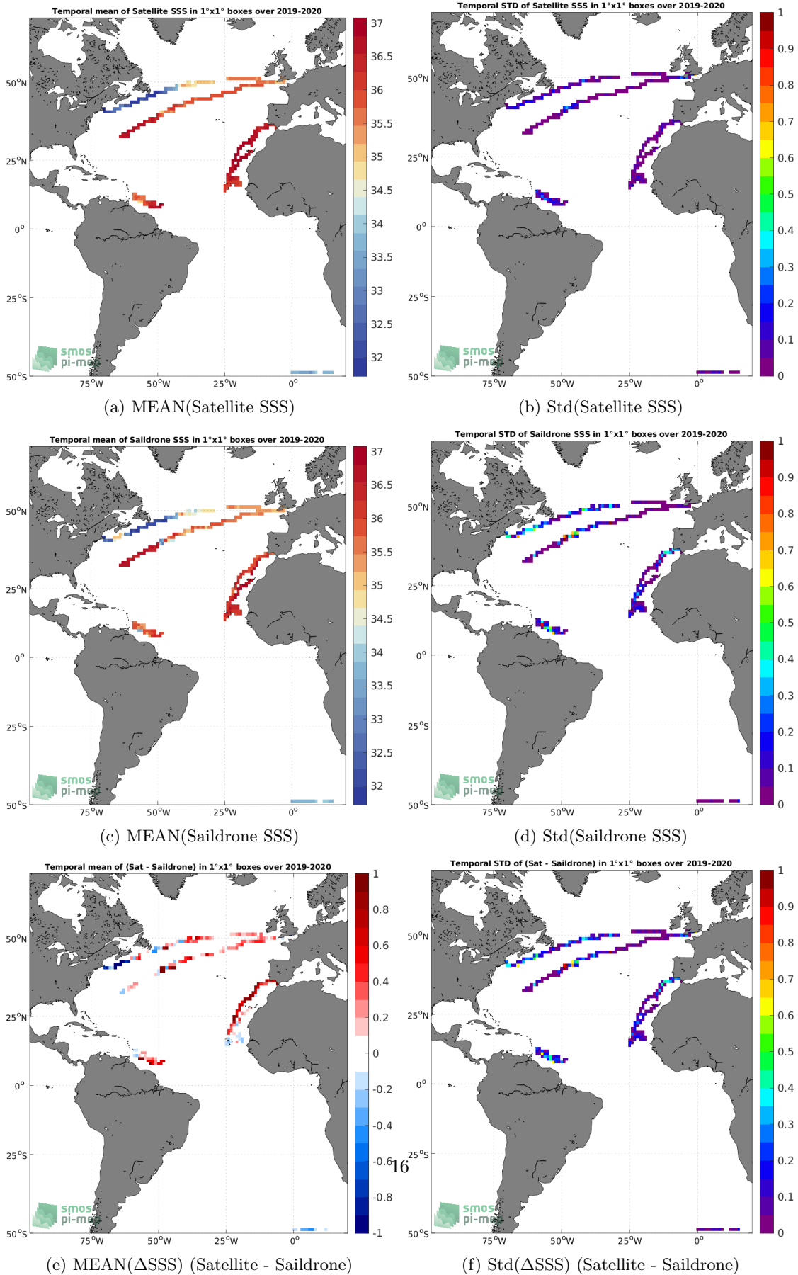
(e) MEAN( \Delta SSS) (Satellite - Saildrone) (f) Std( \Delta SSS) (Satellite - Saildrone) Figure 6: Temporal mean (left) and Std (right) of SSS from SMOS SSS L4 v2 - Daily (BEC) (top), Saildrone (middle), and of \Delta SSS (Satellite - Saildrone). Only match-up pairs are used to generate these maps.
