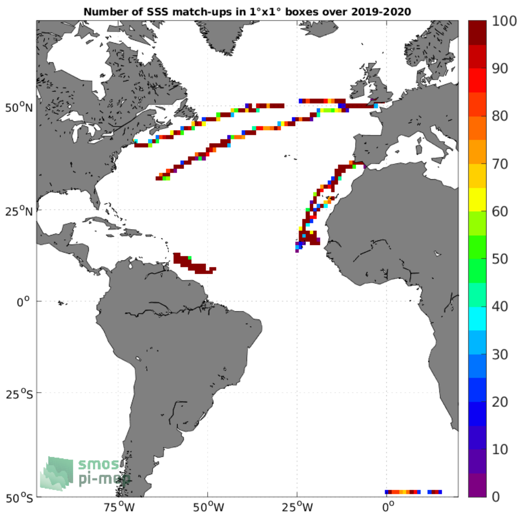
Figure 4: Number of SSS match-ups between Saildrone SSS and the SMOS SSS L4 v2 - Daily (BEC) SSS product for the Atlantic Ocean Pi-MEP region over 1°x1° boxes and for the full satellite product period.
