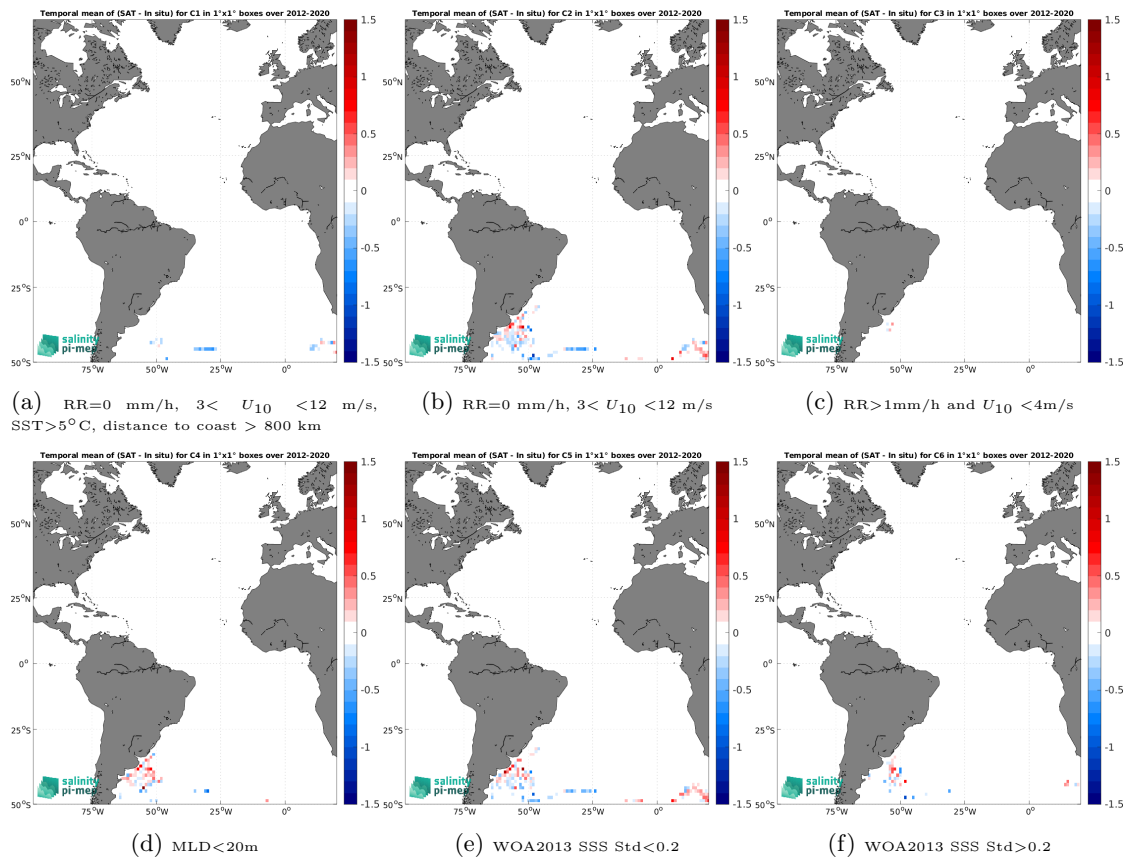
Figure 14: Temporal mean gridded over spatial boxes of size 1^\circ \times 1^\circ of \Delta\text{SSS} (SMOS SSS L4 v2 - Daily (BEC) - Marine mammals) for 6 different subdatasets corresponding to: RR=0 mm/h, 3 < U_{10} < 12 m/s, SST > 5°C, distance to coast > 800 km (a), RR=0 mm/h, 3 < U_{10} < 12 m/s (b), RR > 1 mm/h and U_{10} < 4 m/s (c), MLD < 20m (d), WOA2013 SSS Std < 0.2 (e), WOA2013 SSS Std > 0.2 (f).
