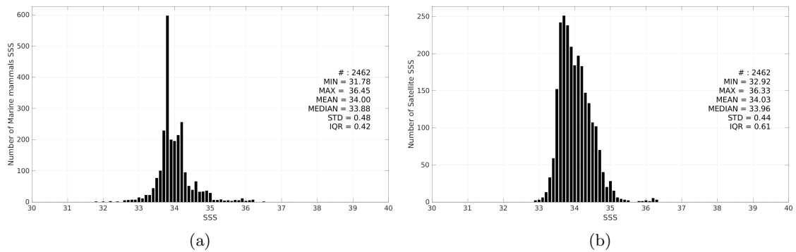
Figure 3: Histograms of SSS from Marine mammals (a) and SMOS SSS L4 v2 - Daily (BEC) (b) considering all match-up pairs per bins of 0.1 over the Atlantic Ocean Pi-MEP region and for the full satellite product period.
