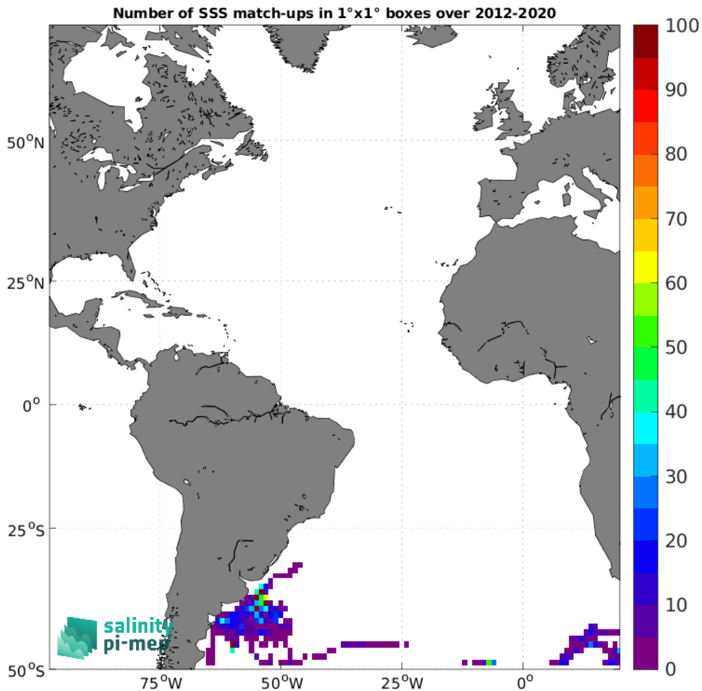
Figure 5: Number of SSS match-ups between Marine mammals SSS and the SMOS SSS L4 v2 - Daily (BEC) SSS product for the Atlantic Ocean Pi-MEP region over 1°×1° boxes and for the full satellite product period.
