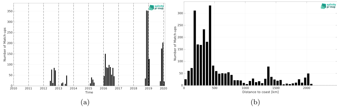
Figure 2: Number of match-ups between Marine mammals and SMOS SSS L4 v2 - Daily (BEC) SSS as a function of time (a) and as function of the distance to coast (b) over the Atlantic Ocean Pi-MEP region and for the full satellite product period.
