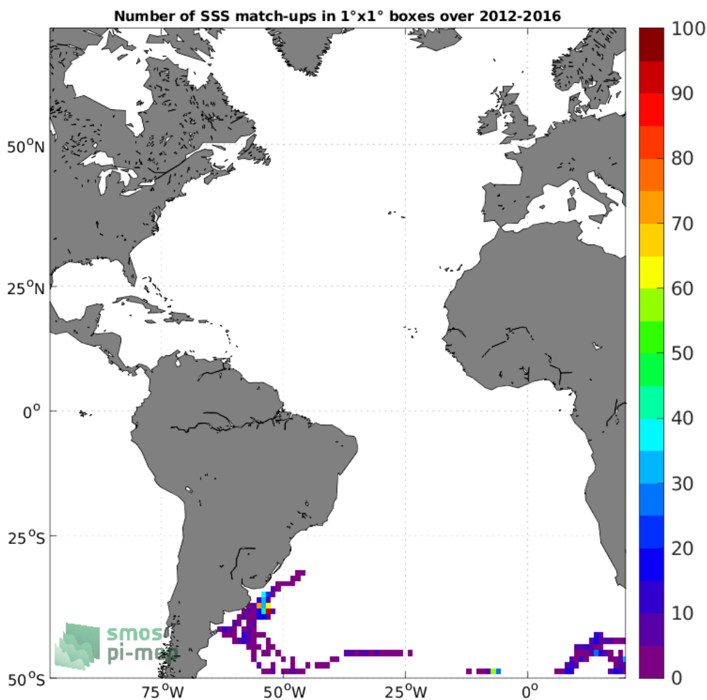
Figure 4: Number of SSS match-ups between Marine mammals SSS and the SMOS SSS L4 v2 - Daily (BEC) SSS product for the Atlantic Ocean Pi-MEP region over 1°×1° boxes and for the full satellite product period.
