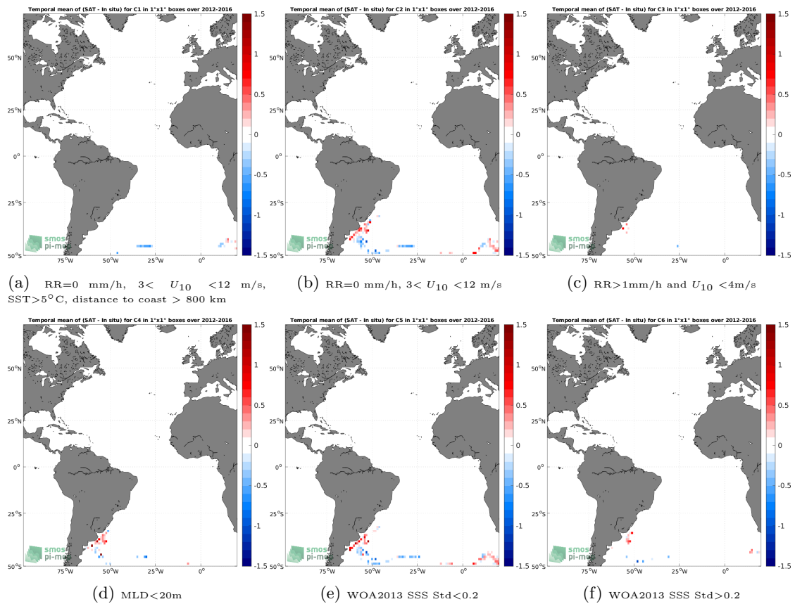
Figure 12: Temporal mean gridded over spatial boxes of size 1^\circ \times 1^\circ of \Delta SSS (SMOS SSS L4 v2 - Daily (BEC) - Marine mammals) for 6 different subdatasets corresponding to: RR=0 mm/h, 3 < U_{10} < 12 m/s, SST > 5^\circ\text{C} , distance to coast > 800 km (a), RR=0 mm/h, 3 < U_{10} < 12 m/s (b), RR > 1 mm/h and U_{10} < 4 m/s (c), MLD < 20 m (d), WOA2013 SSS Std < 0.2 (e), WOA2013 SSS Std > 0.2 (f).
