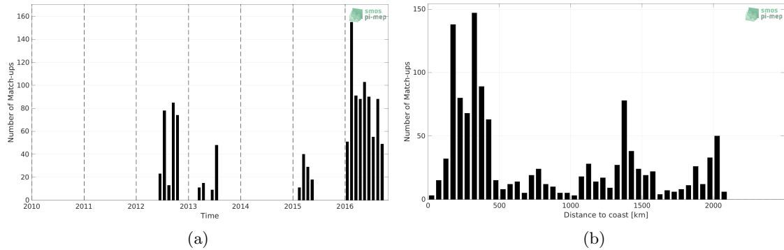
Figure 1: Number of match-ups between Marine mammals and SMOS SSS L4 v2 - Daily (BEC) SSS as a function of time (a) and as function of the distance to coast (b) over the Atlantic Ocean Pi-MEP region and for the full satellite product period.
