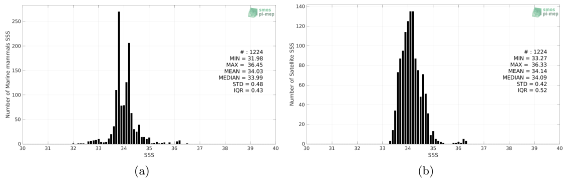
Figure 2: Histograms of SSS from Marine mammals (a) and SMOS SSS L4 v2 - Daily (BEC) (b) considering all match-up pairs per bins of 0.1 over the Atlantic Ocean Pi-MEP region and for the full satellite product period.
