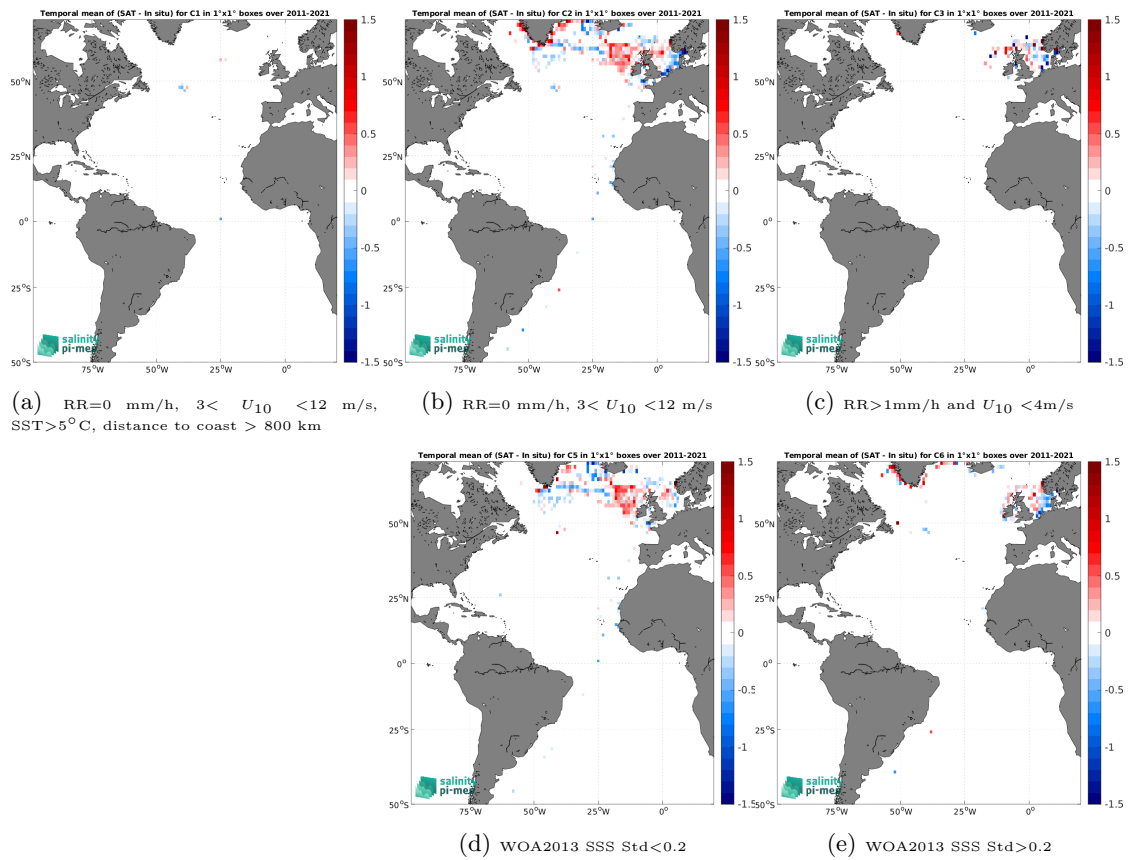
Figure 14: Temporal mean gridded over spatial boxes of size 1^\circ \times 1^\circ of \Delta\text{SSS} (SMOS SSS L4 v2 - Daily (BEC) - ICES) for 5 different subdatasets corresponding to:RR=0 mm/h, 3 < U_{10} < 12 m/s, SST>5°C, distance to coast > 800 km (a), RR=0 mm/h, 3 < U_{10} < 12 m/s (b), RR>1mm/h and U_{10} < 4 m/s (c), WOA2013 SSS Std<0.2 (d), WOA2013 SSS Std>0.2 (e).
