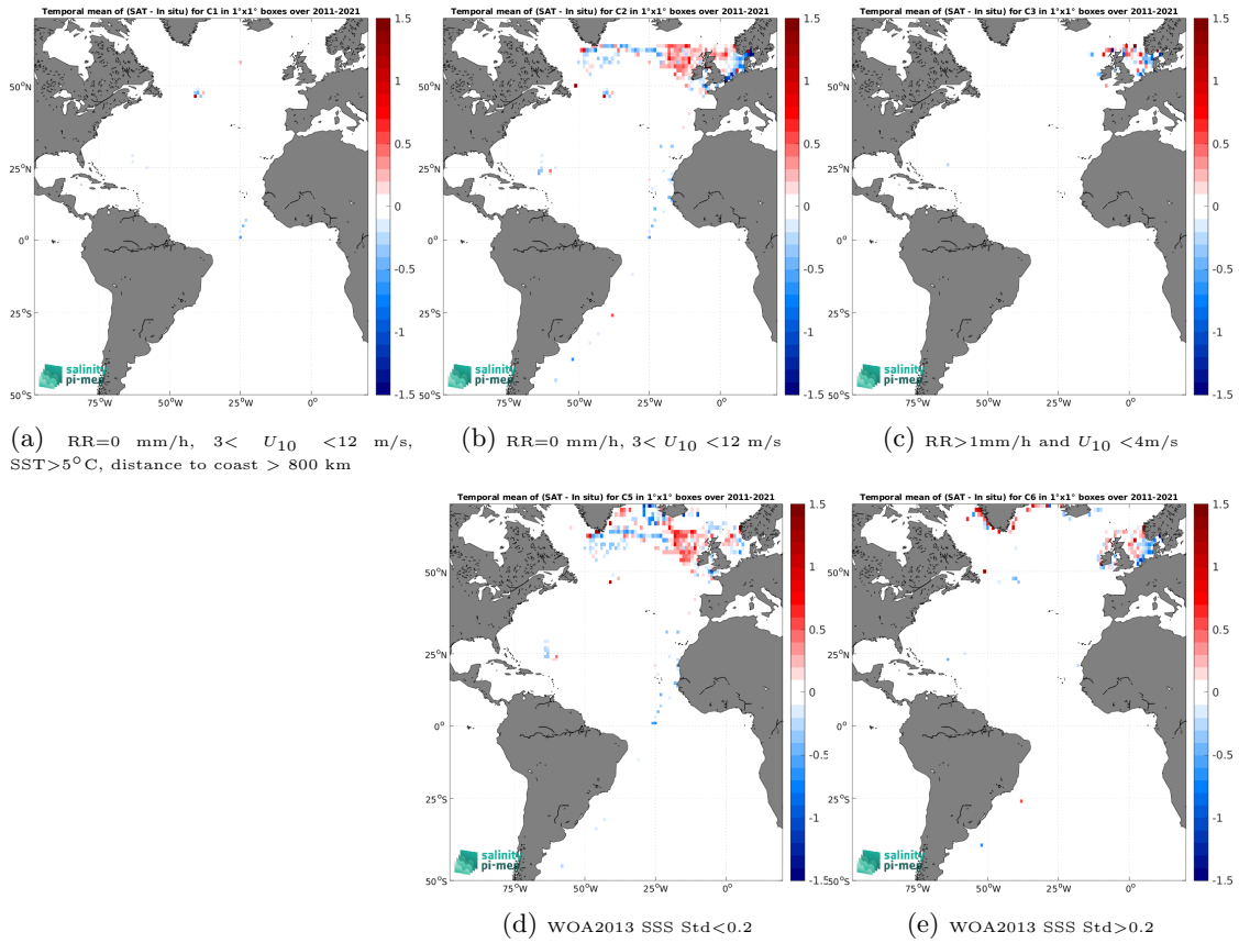
Figure 12: Temporal mean gridded over spatial boxes of size 1^\circ \times 1^\circ of \Delta SSS (SMOS SSS L4 v2 - Daily (BEC) - ICES) for 5 different subdatasets corresponding to:RR=0 mm/h, 3 < U_{10} < 12 m/s, SST >5^\circ\text{C} , distance to coast > 800 km (a), RR=0 mm/h, 3 < U_{10} < 12 m/s (b), RR >1 mm/h and U_{10} < 4 m/s (c), WOA2013 SSS Std <0.2 (d), WOA2013 SSS Std >0.2 (e).
