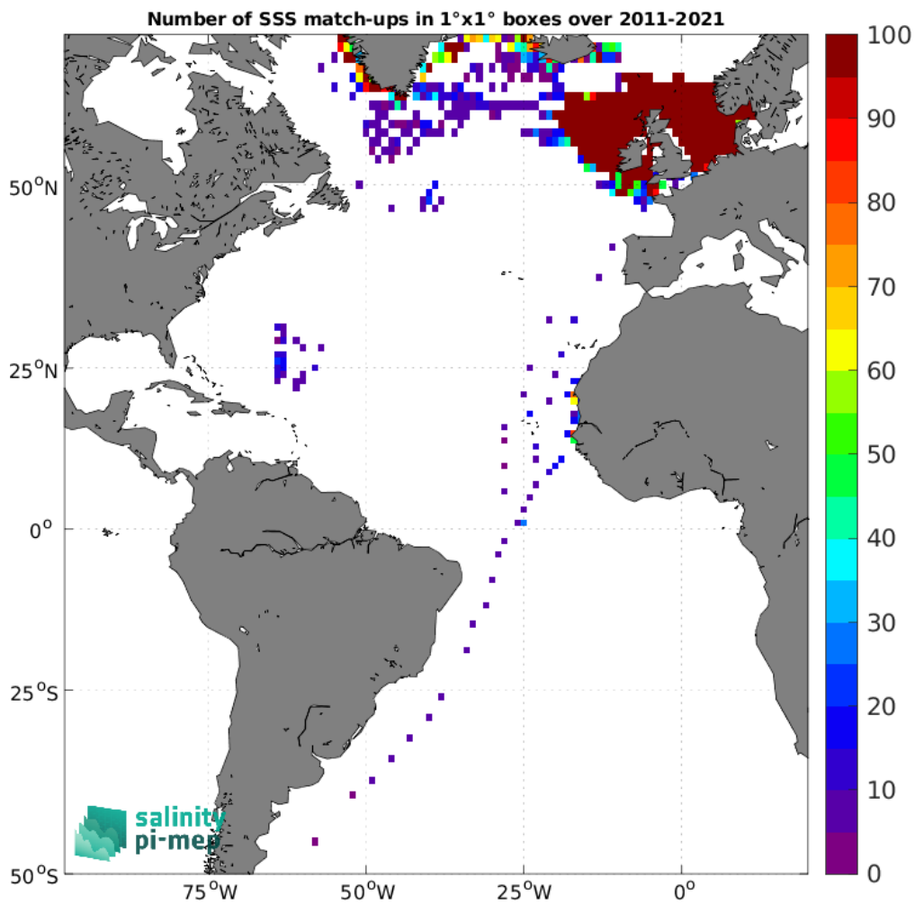
Figure 4: Number of SSS match-ups between ICES SSS and the SMOS SSS L4 v2 - Daily (BEC) SSS product for the Atlantic Ocean Pi-MEP region over 1^\circ \times 1^\circ boxes and for the full satellite product period.
