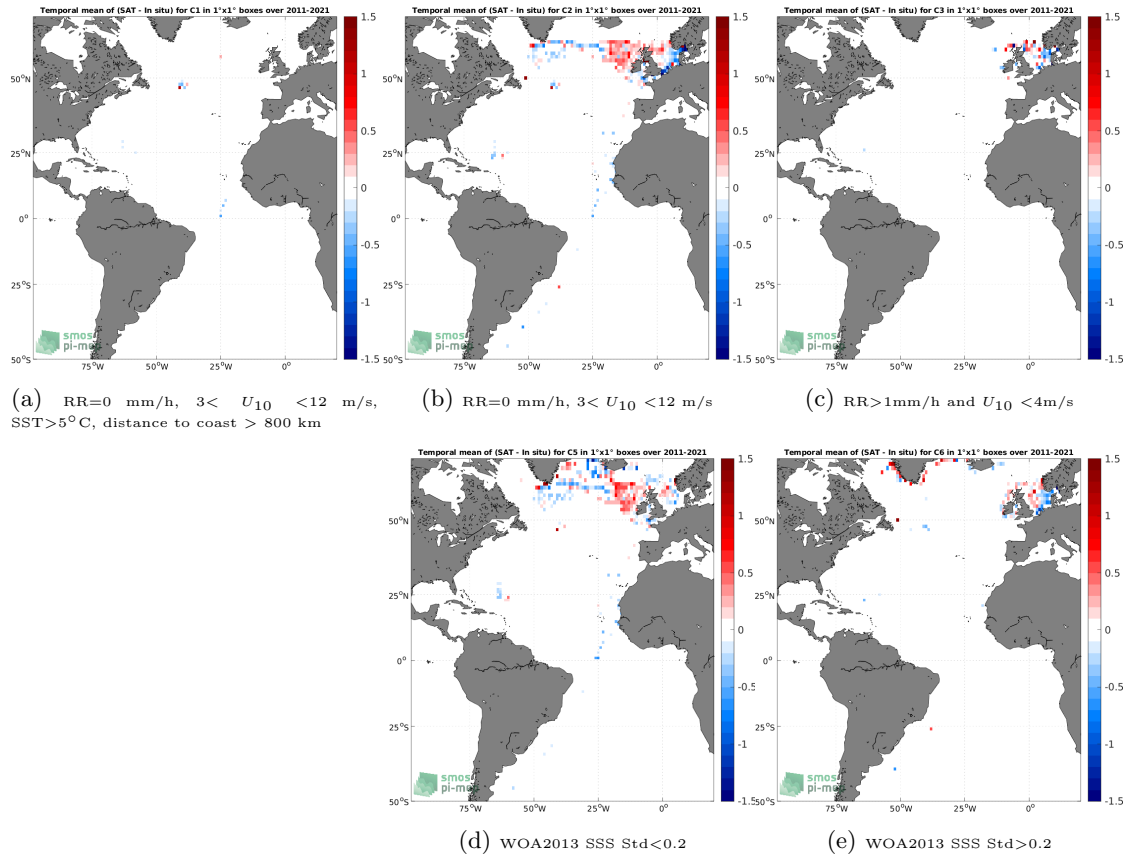
Figure 12: Temporal mean gridded over spatial boxes of size 1^\circ \times 1^\circ of \Delta SSS (SMOS SSS L4 v2 - Daily (BEC) - ICES) for 5 different subdatasets corresponding to:RR=0 mm/h, 3 < U_{10} < 12 m/s, SST >5^\circ\text{C} , distance to coast > 800 km (a), RR=0 mm/h, 3 < U_{10} < 12 m/s (b), RR >1 mm/h and U_{10} < 4 m/s (c), WOA2013 SSS Std <0.2 (d), WOA2013 SSS Std >0.2 (e).
