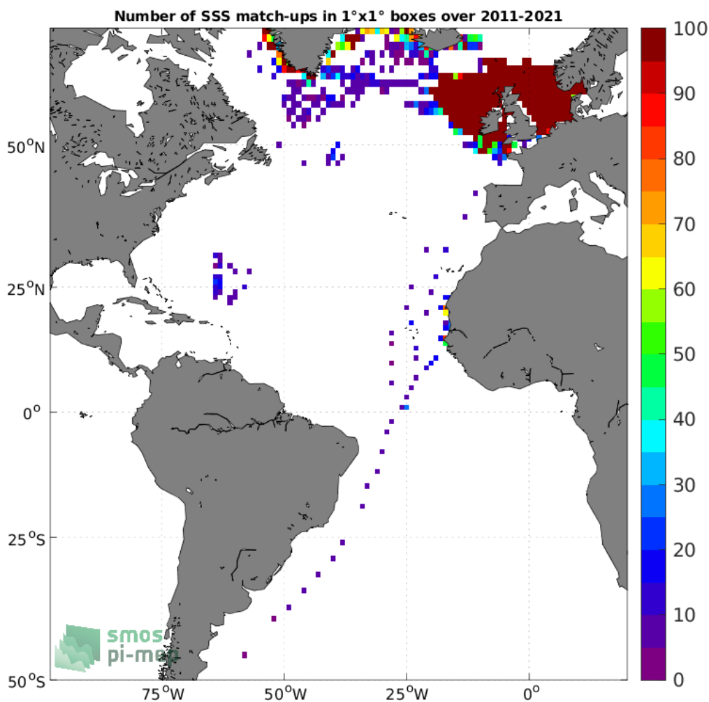
Figure 4: Number of SSS match-ups between ICES SSS and the SMOS SSS L4 v2 - Daily (BEC) SSS product for the Atlantic Ocean Pi-MEP region over 1°x1° boxes and for the full satellite product period.
