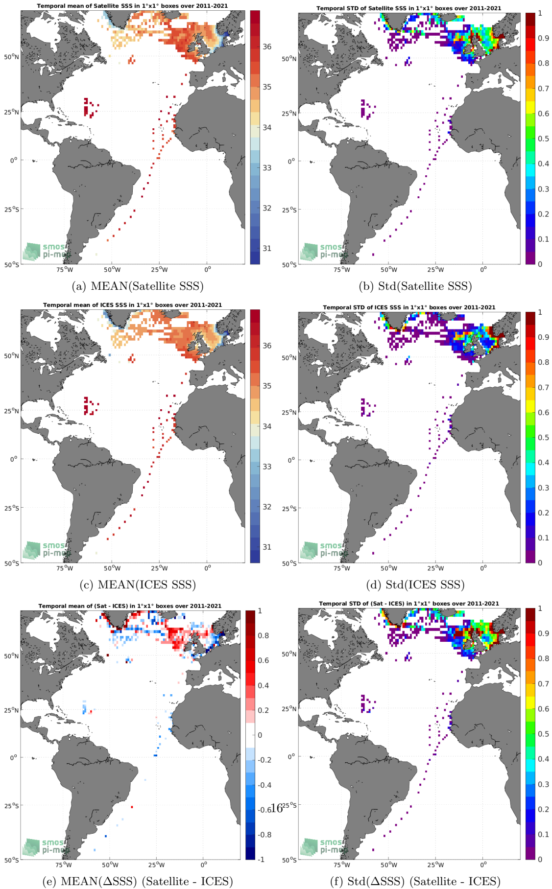
Figure 6: Temporal mean (left) and Std (right) of SSS from SMOS SSS L4 v2 - Daily (BEC) (top), ICES (middle), and of \Delta SSS (Satellite - ICES). Only match-up pairs are used to generate these maps.
