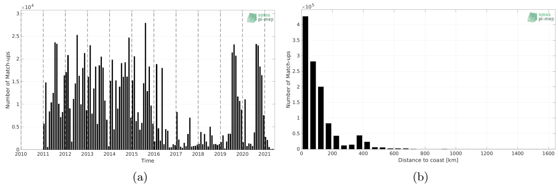
Figure 1: Number of match-ups between ICES and SMOS SSS L4 v2 - Daily (BEC) SSS as a function of time (a) and as function of the distance to coast (b) over the Atlantic Ocean Pi-MEP region and for the full satellite product period.
