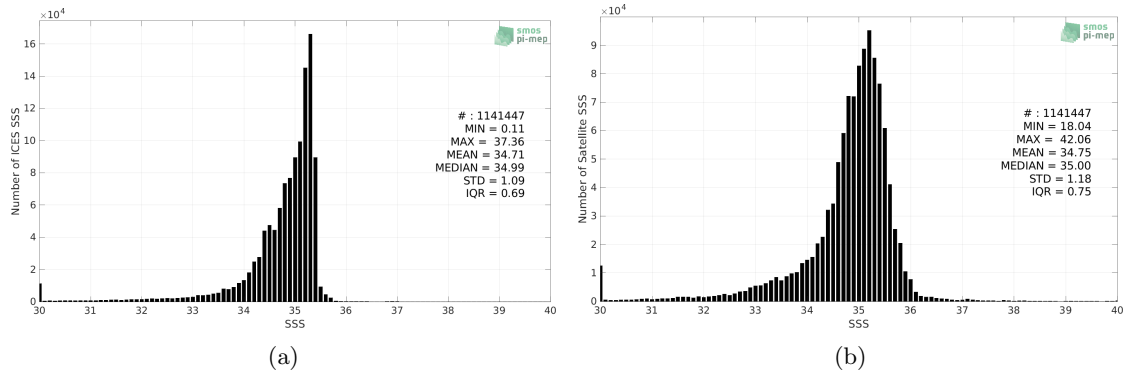
Figure 2: Histograms of SSS from ICES (a) and SMOS SSS L4 v2 - Daily (BEC) (b) considering all match-up pairs per bins of 0.1 over the Atlantic Ocean Pi-MEP region and for the full satellite product period.
