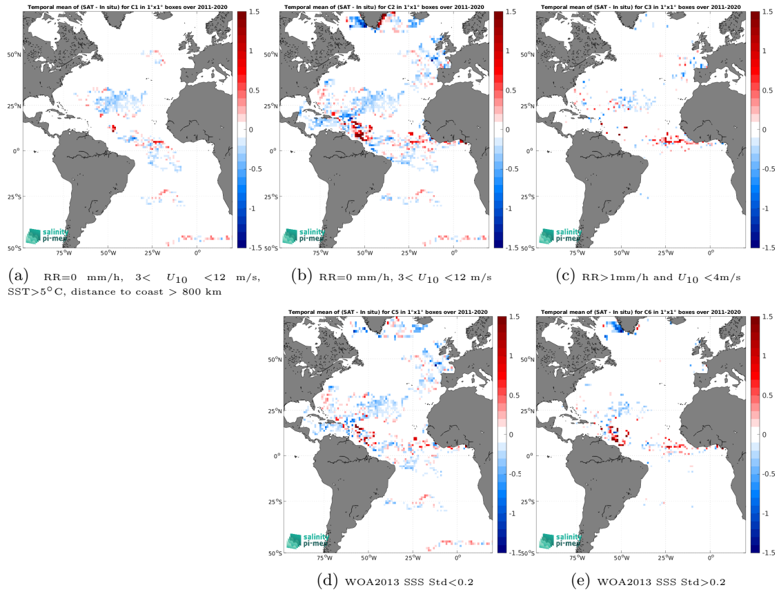
Figure 13: Temporal mean gridded over spatial boxes of size 1^\circ \times 1^\circ of \Delta SSS (SMOS SSS L4 v2 - Daily (BEC) - Surface drifters) for 5 different subdatasets corresponding to:RR=0 mm/h, 3 < U_{10} < 12 m/s, SST >5^\circ\text{C} , distance to coast > 800 km (a), RR=0 mm/h, 3 < U_{10} < 12 m/s (b), RR >1 mm/h and U_{10} < 4 m/s (c), WOA2013 SSS Std <0.2 (d), WOA2013 SSS Std >0.2 (e).
