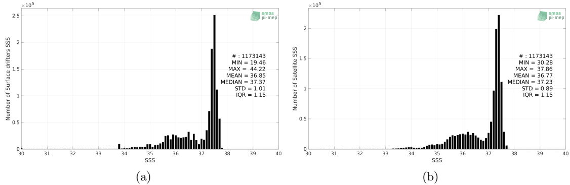
Figure 2: Histograms of SSS from Surface drifters (a) and SMOS SSS L4 v2 - Daily (BEC) (b) considering all match-up pairs per bins of 0.1 over the Atlantic Ocean Pi-MEP region and for the full satellite product period.
