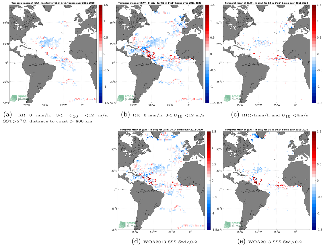
Figure 11: Temporal mean gridded over spatial boxes of size 1^\circ \times 1^\circ of \Delta SSS (SMOS SSS L4 v2 - Daily (BEC) - Surface drifters) for 5 different subdatasets corresponding to:RR=0 mm/h, 3 < U_{10} < 12 m/s, SST >5^\circ\text{C} , distance to coast > 800 km (a), RR=0 mm/h, 3 < U_{10} < 12 m/s (b), RR >1 mm/h and U_{10} < 4 m/s (c), WOA2013 SSS Std <0.2 (d), WOA2013 SSS Std >0.2 (e).
