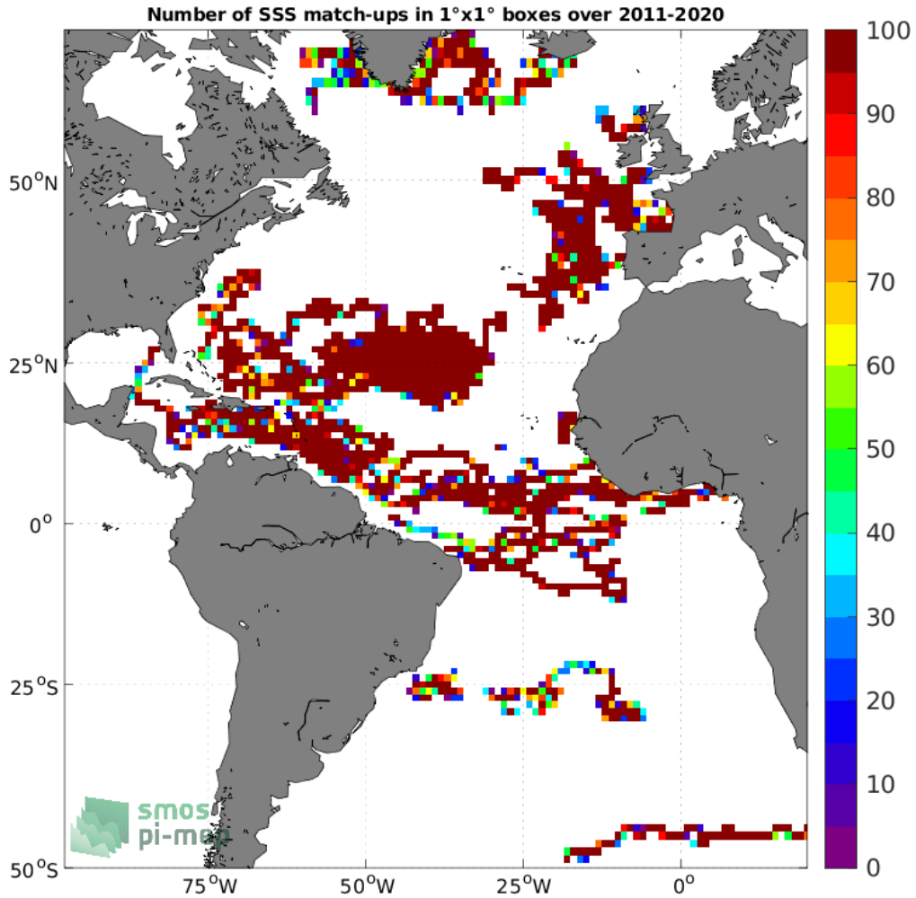
Figure 3: Number of SSS match-ups between Surface drifters SSS and the SMOS SSS L4 v2 - Daily (BEC) SSS product for the Atlantic Ocean Pi-MEP region over 1^\circ \times 1^\circ boxes and for the full satellite product period.
