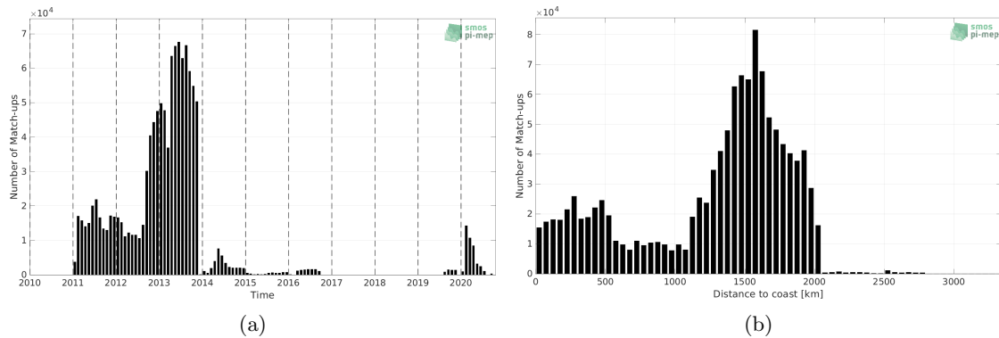
Figure 1: Number of match-ups between Surface drifters and SMOS SSS L4 v2 - Daily (BEC) SSS as a function of time (a) and as function of the distance to coast (b) over the Atlantic Ocean Pi-MEP region and for the full satellite product period.
