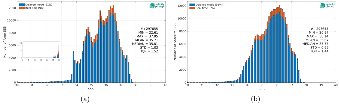
Figure 2: Histograms of SSS from Argo (a) and SMOS SSS L4 v2 - Daily (BEC) (b) considering all match-up pairs per bins of 0.1 over the Atlantic Ocean Pi-MEP region and for the full satellite product period.
