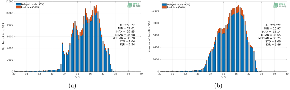
Figure 2: Histograms of SSS from Argo (a) and SMOS SSS L4 v2 - Daily (BEC) (b) considering all match-up pairs per bins of 0.1 over the Atlantic Ocean Pi-MEP region and for the full satellite product period.
