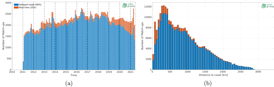
Figure 1: Number of match-ups between Argo and SMOS SSS L4 v2 - Daily (BEC) SSS as a function of time (a) and as function of the distance to coast (b) over the Atlantic Ocean Pi-MEP region and for the full satellite product period.
