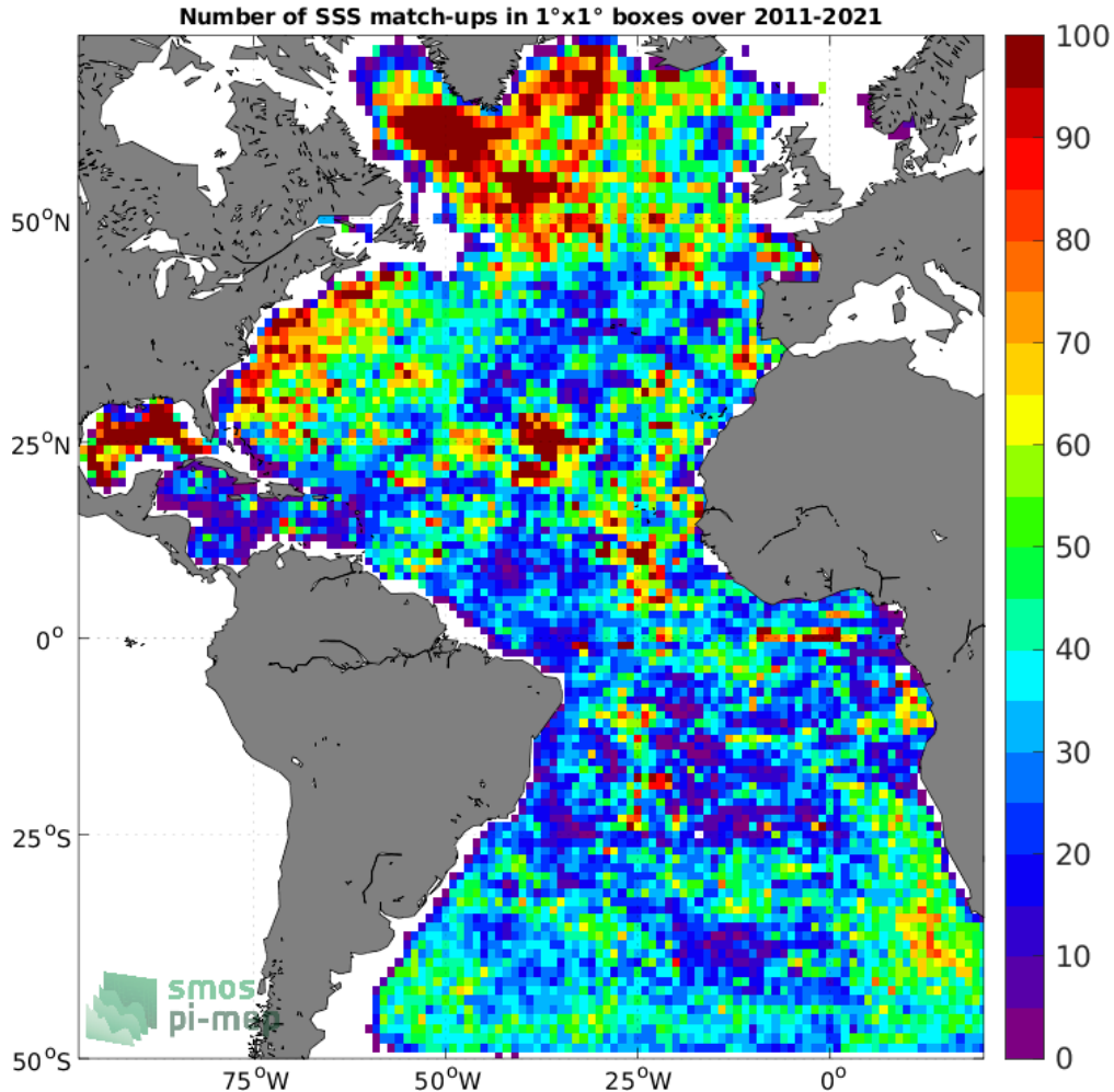
Figure 4: Number of SSS match-ups between Argo SSS and the SMOS SSS L4 v2 - Daily (BEC) SSS product for the Atlantic Ocean Pi-MEP region over 1^\circ \times 1^\circ boxes and for the full satellite product period.
