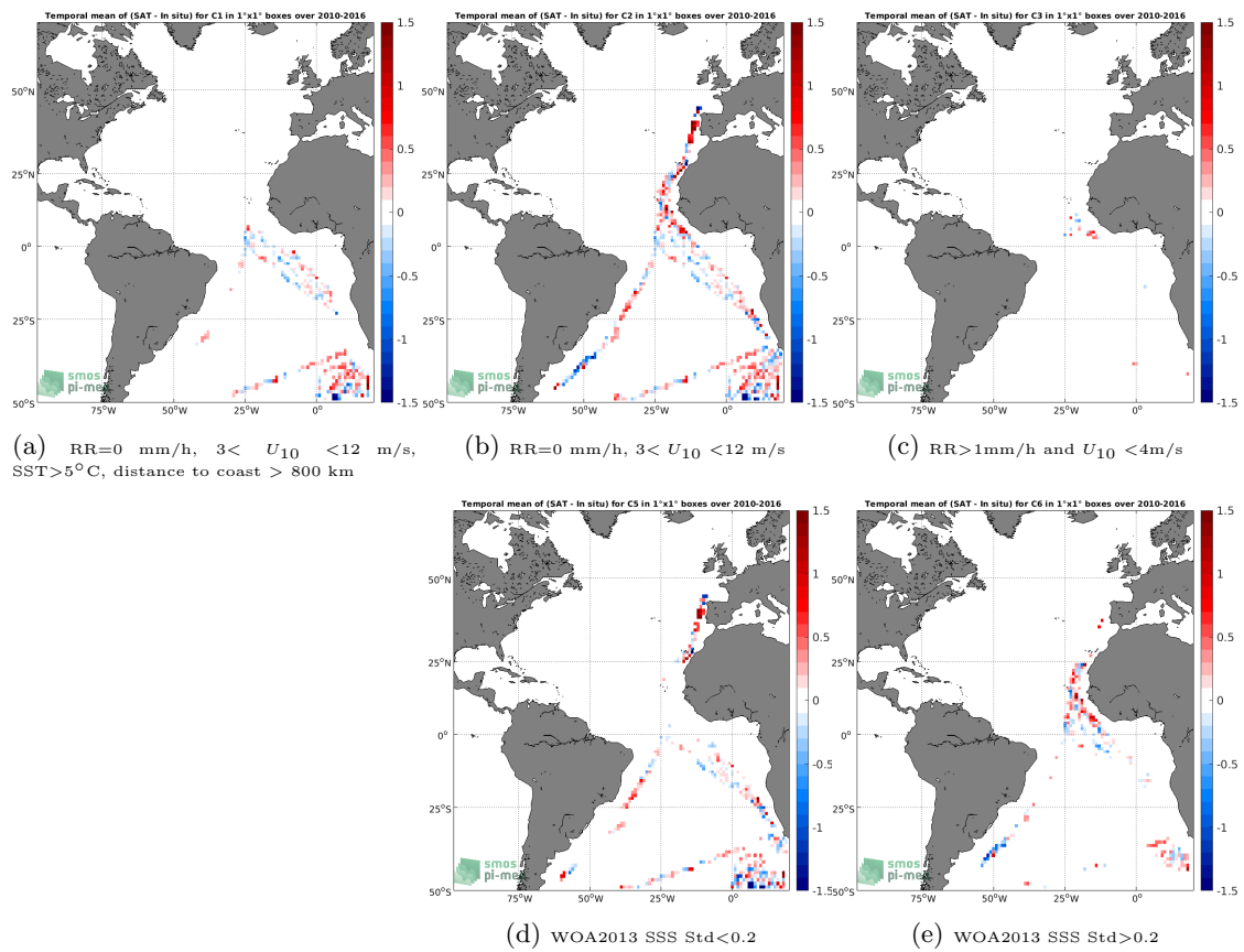
Figure 12: Temporal mean gridded over spatial boxes of size 1^\circ \times 1^\circ of \Delta SSS (SMOS SSS L3 v3 Monthly (ICDC) - TSG (Polarstern)) for 5 different subdatasets corresponding to:RR=0 mm/h, 3 < U_{10} < 12 m/s, SST>5°C, distance to coast > 800 km (a), RR=0 mm/h, 3 < U_{10} < 12 m/s (b), RR>1mm/h and U_{10} < 4 m/s (c), WOA2013 SSS Std<0.2 (d), WOA2013 SSS Std>0.2 (e).
