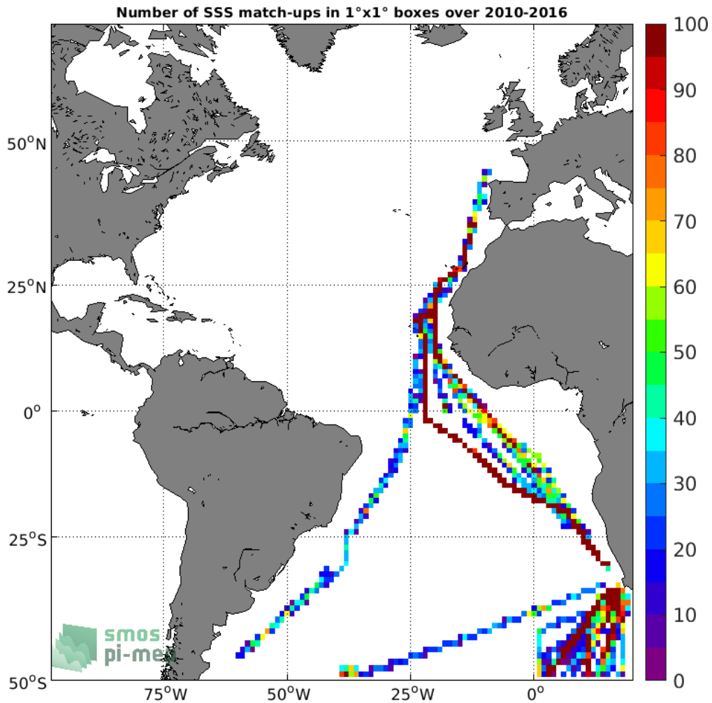
Figure 4: Number of SSS match-ups between TSG (Polarstern) SSS and the SMOS SSS L3 v3 Monthly (ICDC) SSS product for the Atlantic Ocean Pi-MEP region over 1^\circ \times 1^\circ boxes and for the full satellite product period.
