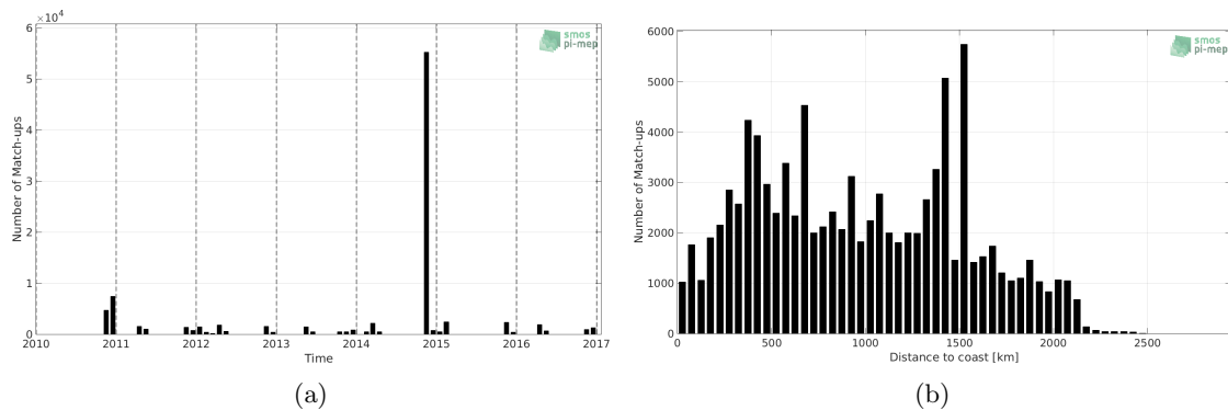
Figure 1: Number of match-ups between TSG-POLARSTERN and SMOS-L3-ICDC-V3-MONTHLY-0.5DEG SSS as a function of time (a) and as function of the distance to coast (b) over the Atlantic Ocean Pi-MEP region and for the full satellite product period.
