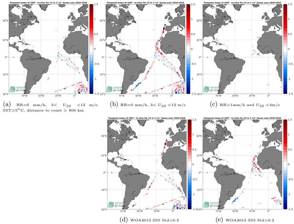
Figure 12: Temporal mean gridded over spatial boxes of size 1^\circ \times 1^\circ of \Delta SSS (SMOS-L3-ICDC-V3-MONTHLY-0.5DEG - TSG-POLARSTERN) for 5 different subdatasets corresponding to:RR=0 mm/h, 3 < U_{10} < 12 m/s, SST >5^\circ\text{C} , distance to coast > 800 km (a), RR=0 mm/h, 3 < U_{10} < 12 m/s (b), RR >1 mm/h and U_{10} < 4 m/s (c), WOA2013 SSS Std <0.2 (d), WOA2013 SSS Std >0.2 (e).
