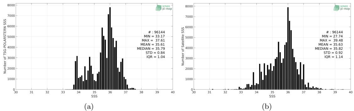
Figure 2: Histograms of SSS from TSG-POLARSTERN (a) and SMOS-L3-ICDC-V3-MONTHLY-0.5DEG (b) considering all match-up pairs per bins of 0.1 over the Atlantic Ocean Pi-MEP region and for the full satellite product period.
