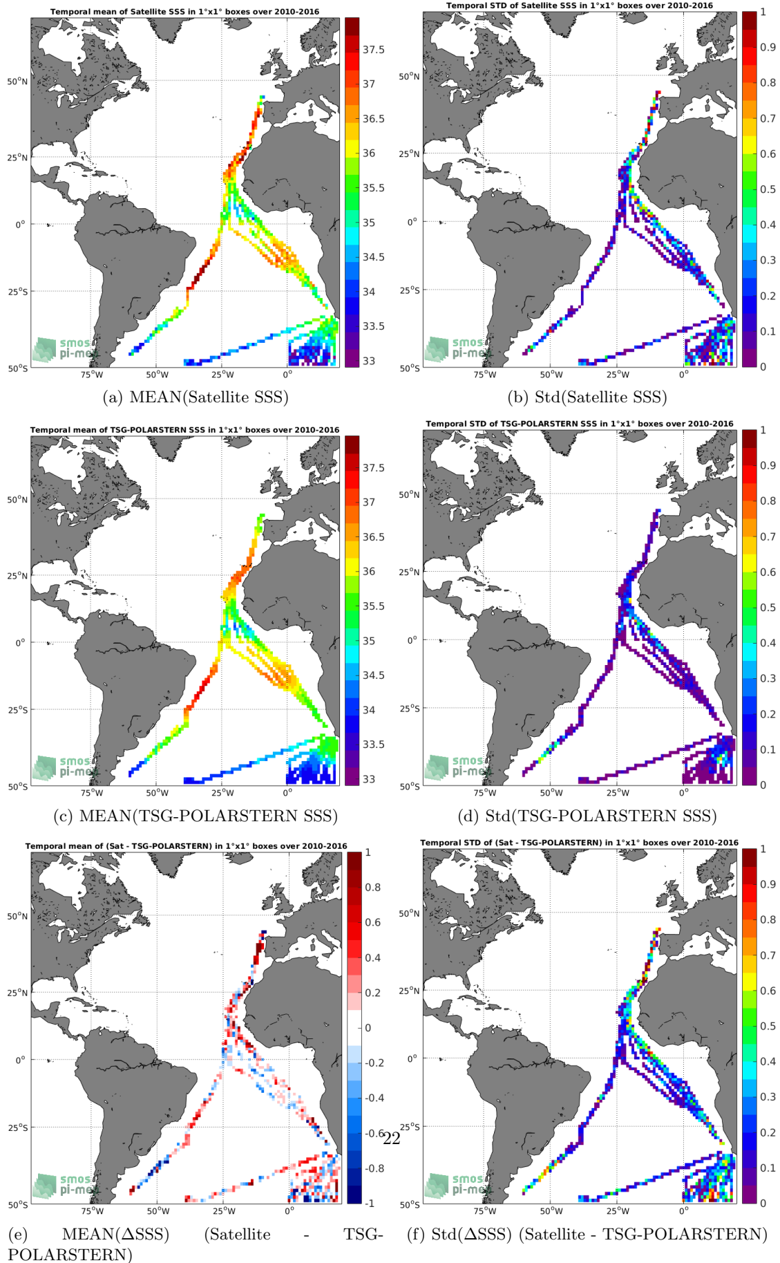
Figure 6: Temporal mean (left) and Std (right) of SSS from SMOS-L3-ICDC-V3-MONTHLY-0.5DEG (top), TSG-POLARSTERN (middle), and of \Delta SSS (Satellite - TSG-POLARSTERN). Only match-up pairs are used to generate these maps.
