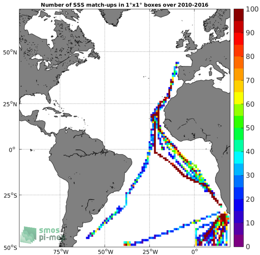
Figure 4: Number of SSS match-ups between TSG-POLARSTERN SSS and the SMOS-L3-ICDC-V3-MONTHLY-0.5DEG SSS product for the Atlantic Ocean Pi-MEP region over 1°x1° boxes and for the full satellite product period.
