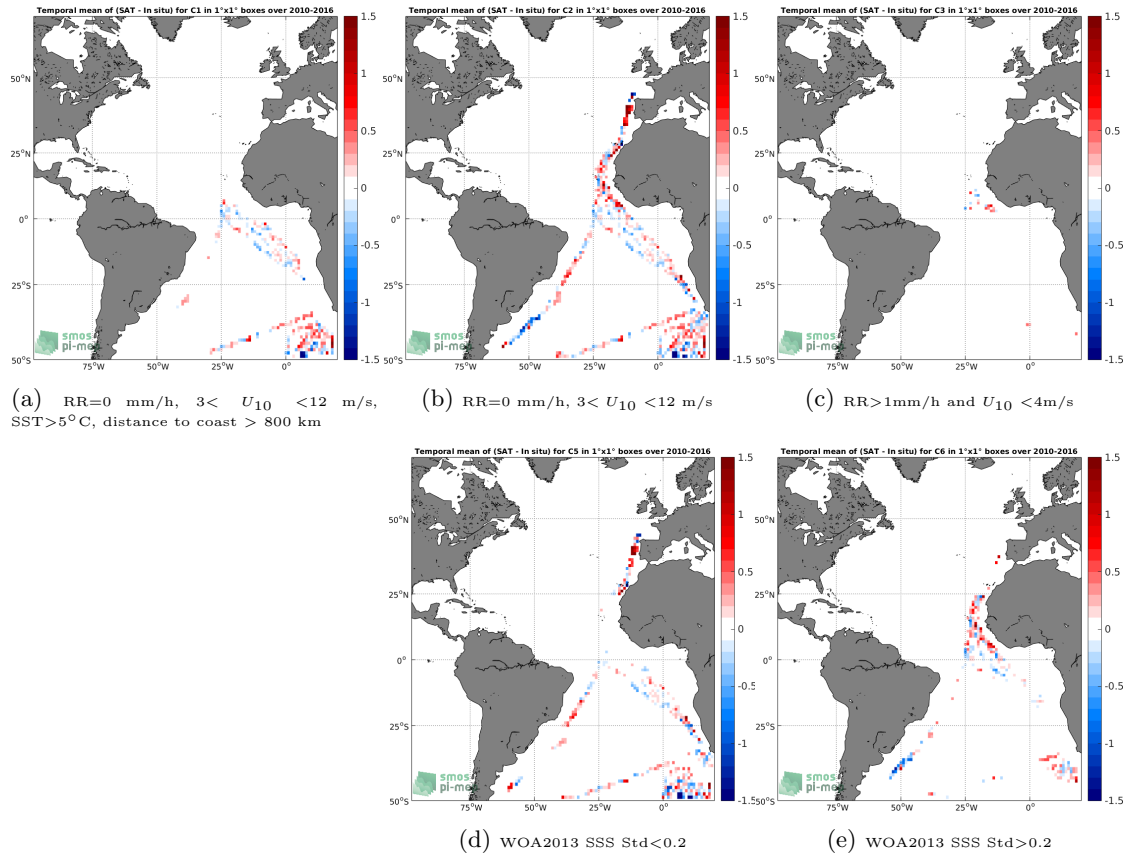
Figure 12: Temporal mean gridded over spatial boxes of size 1^\circ \times 1^\circ of \Delta SSS (SMOS-L3-ICDC-V3-MONTHLY-0.5DEG - TSG-POLARSTERN) for 5 different subdatasets corresponding to: RR=0 mm/h, 3 < U_{10} < 12 m/s, SST > 5^\circ C , distance to coast > 800 km (a), RR=0 mm/h, 3 < U_{10} < 12 m/s (b), RR > 1 mm/h and U_{10} < 4 m/s (c), WOA2013 SSS Std < 0.2 (d), WOA2013 SSS Std > 0.2 (e).
