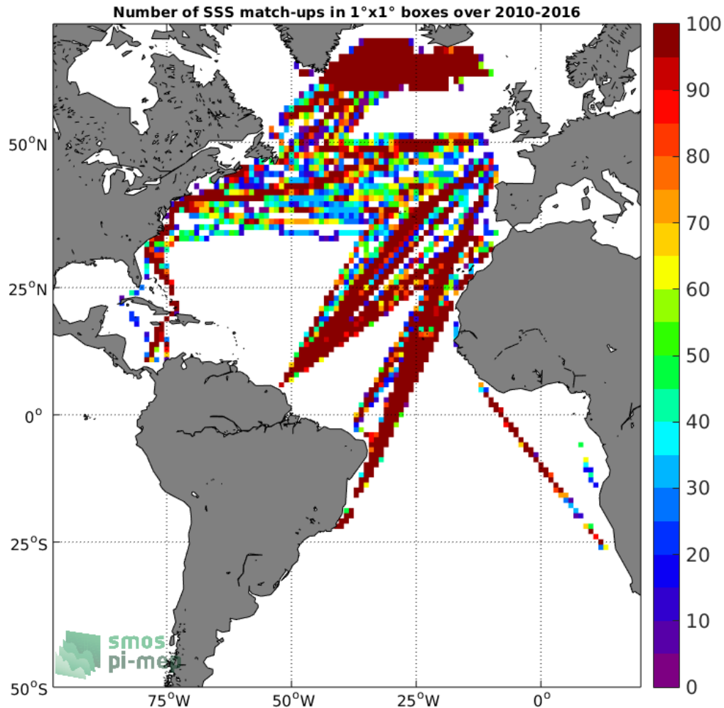
Figure 4: Number of SSS match-ups between TSG (LEGOS-DM) SSS and the SMOS SSS L3 v3 Monthly (ICDC) SSS product for the Atlantic Ocean Pi-MEP region over 1^\circ \times 1^\circ boxes and for the full satellite product period.
