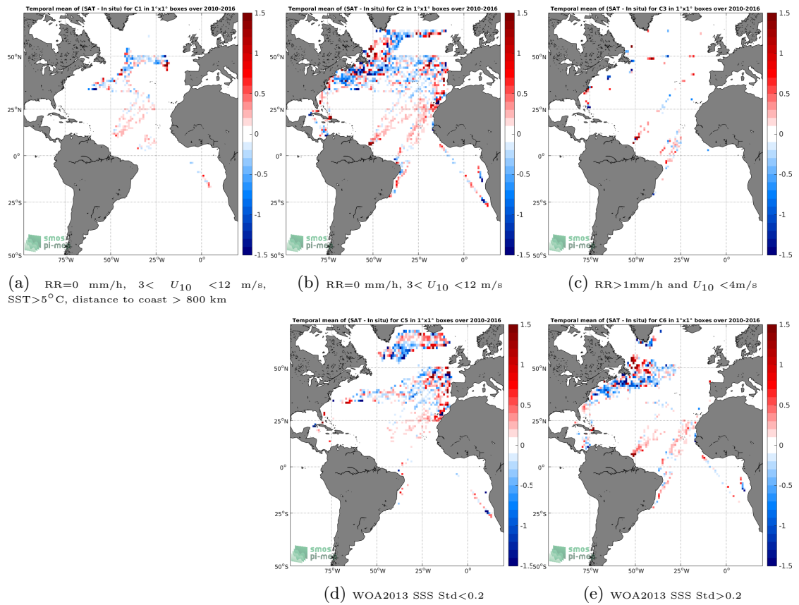
Figure 12: Temporal mean gridded over spatial boxes of size 1^\circ \times 1^\circ of \Delta SSS (SMOS SSS L3 v3 Monthly (ICDC) - TSG (LEGOS-DM)) for 5 different subdatasets corresponding to:RR=0 mm/h, 3 < U_{10} < 12 m/s, SST>5°C, distance to coast > 800 km (a), RR=0 mm/h, 3 < U_{10} < 12 m/s (b), RR>1mm/h and U_{10} < 4 m/s (c), WOA2013 SSS Std<0.2 (d), WOA2013 SSS Std>0.2 (e).
