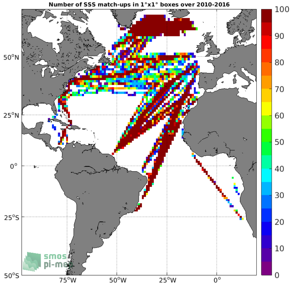
Figure 4: Number of SSS match-ups between TSG (LEGOS-DM) SSS and the SMOS SSS L3 v3 Monthly (ICDC) SSS product for the Atlantic Ocean Pi-MEP region over 1°x1° boxes and for the full satellite product period.
