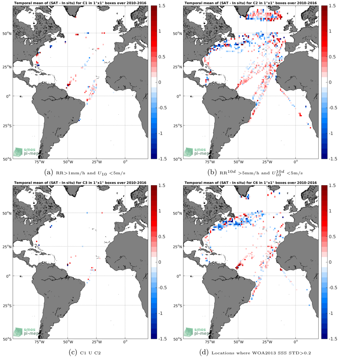
Figure 12: Temporal mean gridded over spatial boxes of size 1^\circ \times 1^\circ of \Delta SSS (SMOS-L3-ICDC-V3-MONTHLY-0.5DEG - TSG-LEGOS-DM) for 4 different subdatasets corresponding to: RR > 1\text{mm/h} and U_{10} < 5\text{m/s} (a), RR^{10d} > 5\text{mm/h} and U_{10}^{10d} < 5\text{m/s} (b), C1 U C2 (c), Locations where WOA2013 SSS STD > 0.2 (d).
