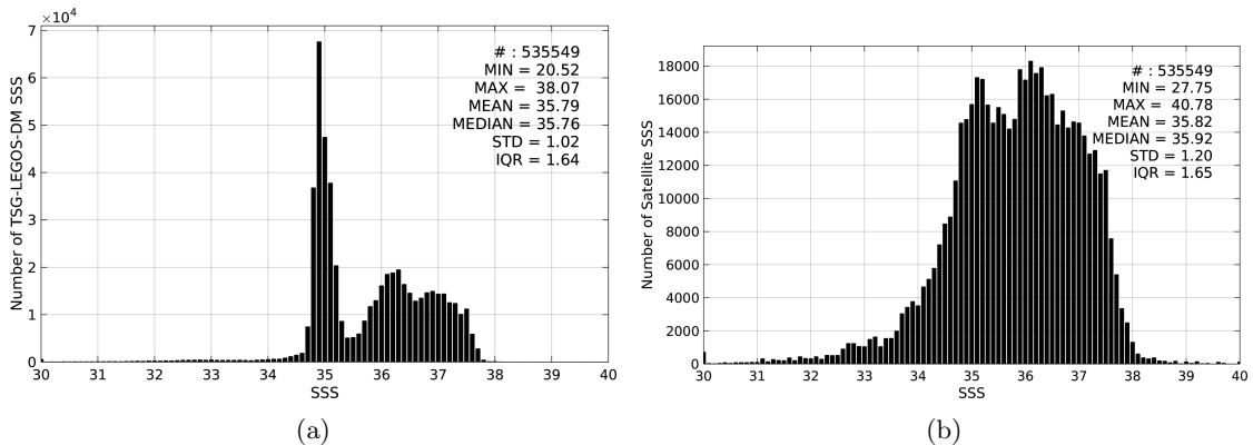
Figure 2: Histograms of SSS from TSG-LEGOS-DM (a) and SMOS-L3-ICDC-V3-MONTHLY-0.5DEG (b) considering all match-up pairs per bins of 0.1 over the Atlantic Ocean Pi-MEP region and for the full satellite product period.
