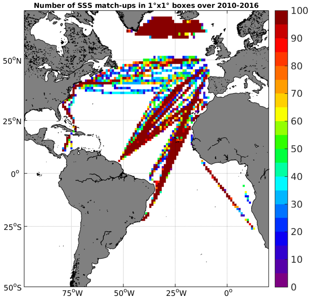
Figure 4: Number of SSS match-ups between TSG-LEGOS-DM SSS and the SMOS-L3-ICDC-V3-MONTHLY-0.5DEG SSS product for the Atlantic Ocean Pi-MEP region over 1^{\circ} \times 1^{\circ} boxes and for the full satellite product period.
