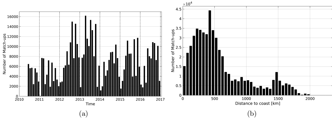
Figure 1: Number of match-ups between TSG-LEGOS-DM and SMOS-L3-ICDC-V3-MONTHLY-0.5DEG SSS as a function of time (a) and as function of the distance to coast (b) over the Atlantic Ocean Pi-MEP region and for the full satellite product period.
