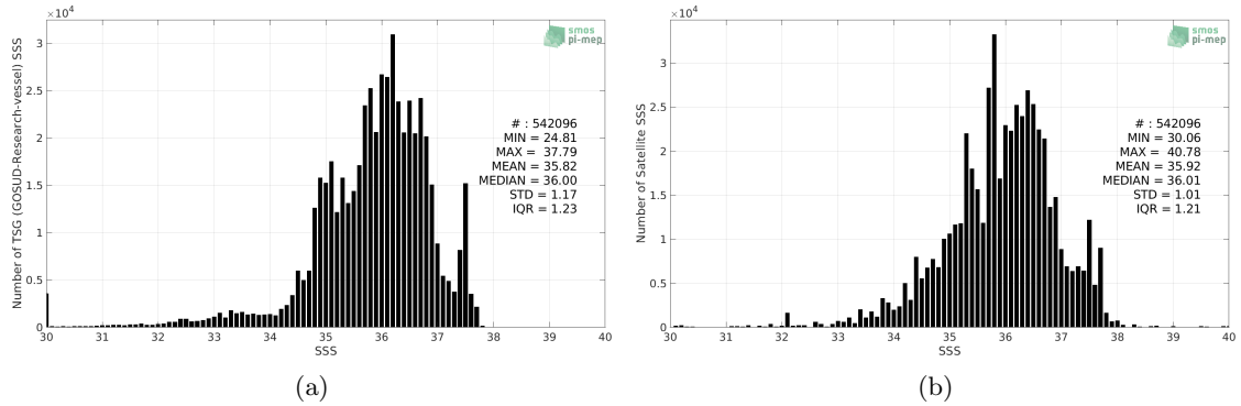
Figure 2: Histograms of SSS from TSG (GOSUD-Research-vessel) (a) and SMOS SSS L3 v3 Monthly (ICDC) (b) considering all match-up pairs per bins of 0.1 over the Atlantic Ocean Pi-MEP region and for the full satellite product period.
