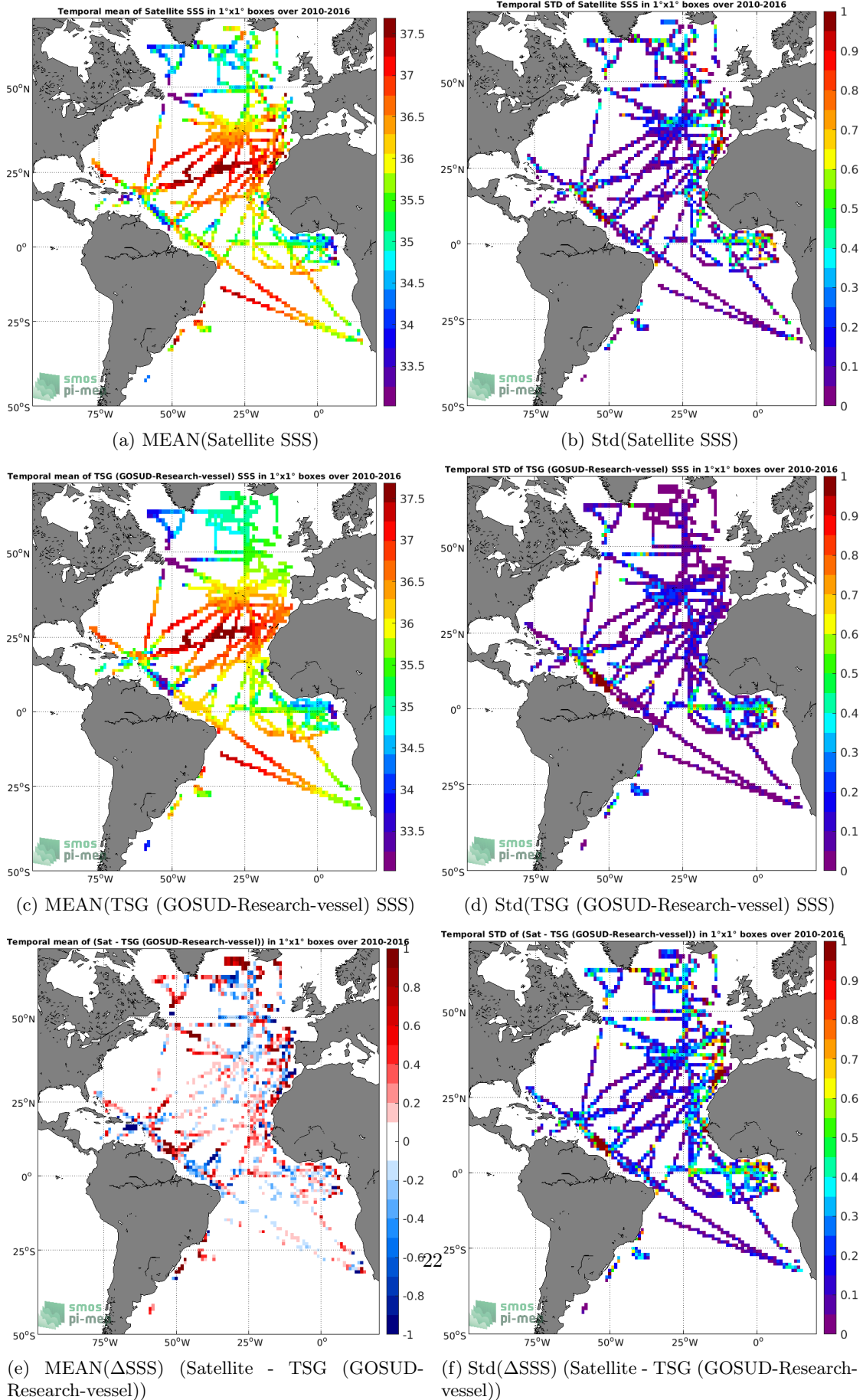
Figure 6: Temporal mean (left) and Std (right) of SSS from SMOS SSS L3 v3 Monthly (ICDC) (top), TSG (GOSUD-Research-vessel) (middle), and of \Delta SSS (Satellite - TSG (GOSUD-Research-vessel)). Only match-up pairs are used to generate these maps.
