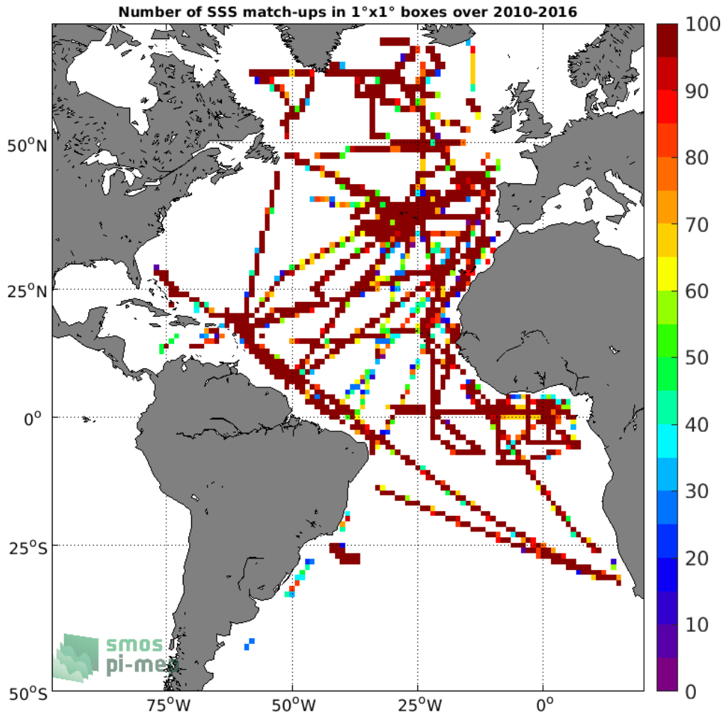
Figure 4: Number of SSS match-ups between TSG (GOSUD-Research-vessel) SSS and the SMOS SSS L3 v3 Monthly (ICDC) SSS product for the Atlantic Ocean Pi-MEP region over 1^\circ \times 1^\circ boxes and for the full satellite product period.
