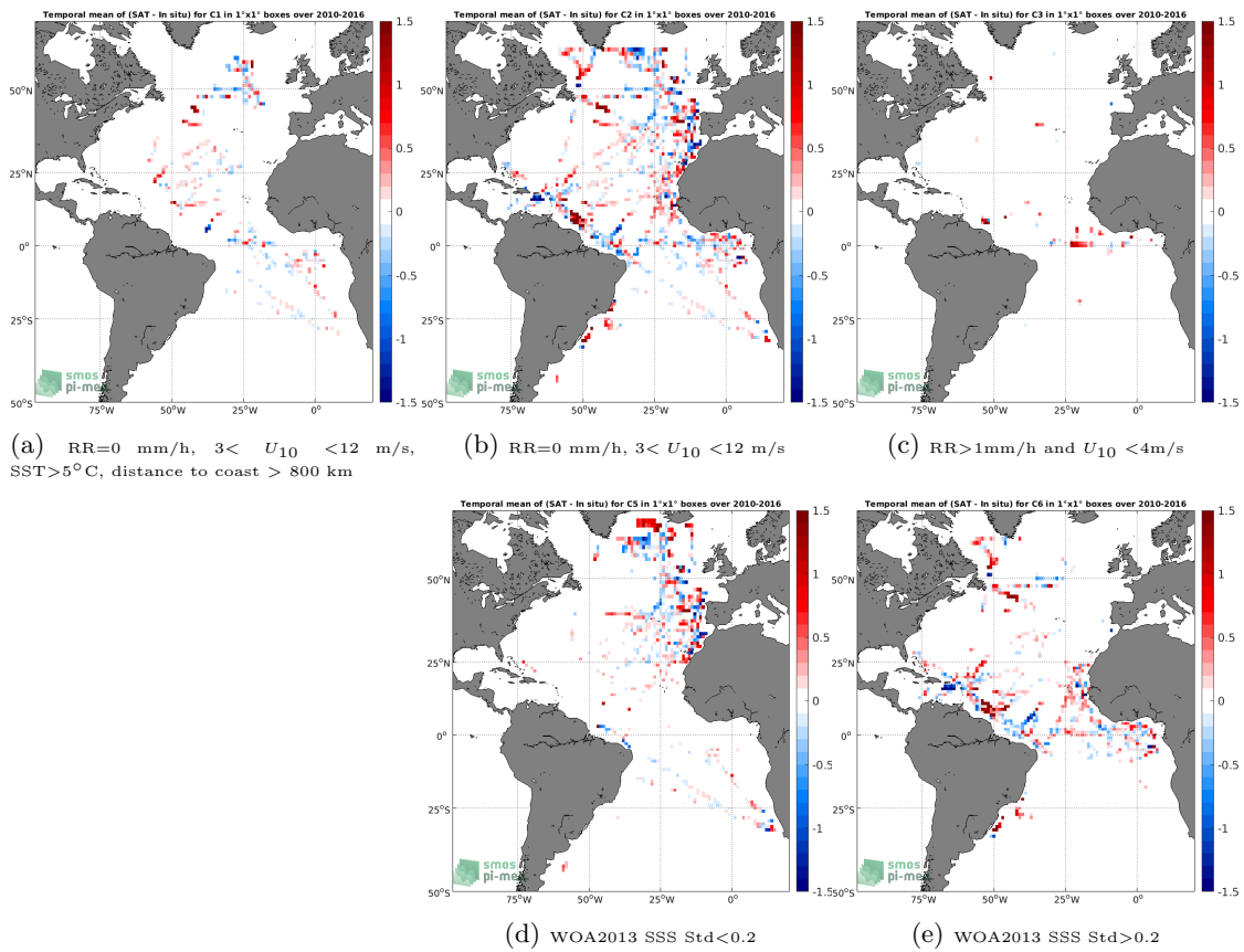
Figure 12: Temporal mean gridded over spatial boxes of size 1^\circ \times 1^\circ of \Delta SSS (SMOS SSS L3 v3 Monthly (ICDC) - TSG (GOSUD-Research-vessel)) for 5 different subdatasets corresponding to:RR=0 mm/h, 3 < U_{10} < 12 m/s, SST>5°C, distance to coast > 800 km (a), RR=0 mm/h, 3 < U_{10} < 12 m/s (b), RR>1mm/h and U_{10} < 4 m/s (c), WOA2013 SSS Std<0.2 (d), WOA2013 SSS Std>0.2 (e).
