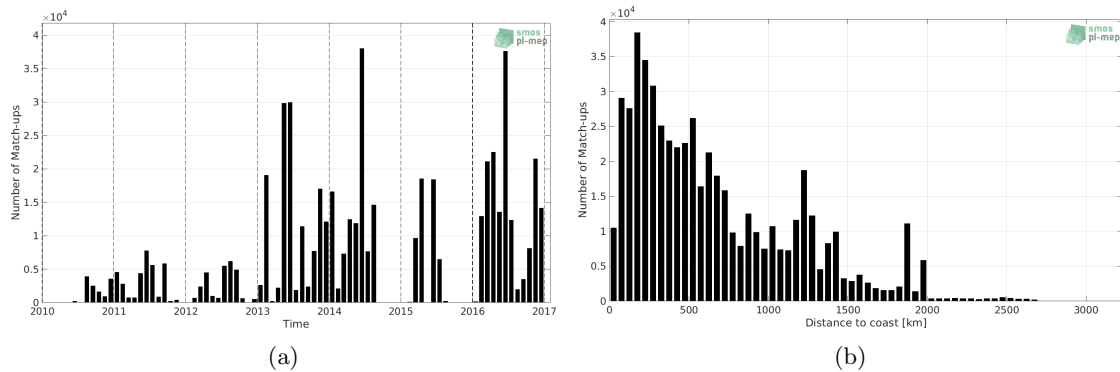
Figure 1: Number of match-ups between TSG (GOSUD-Research-vessel) and SMOS SSS L3 v3 Monthly (ICDC) SSS as a function of time (a) and as function of the distance to coast (b) over the Atlantic Ocean Pi-MEP region and for the full satellite product period.
