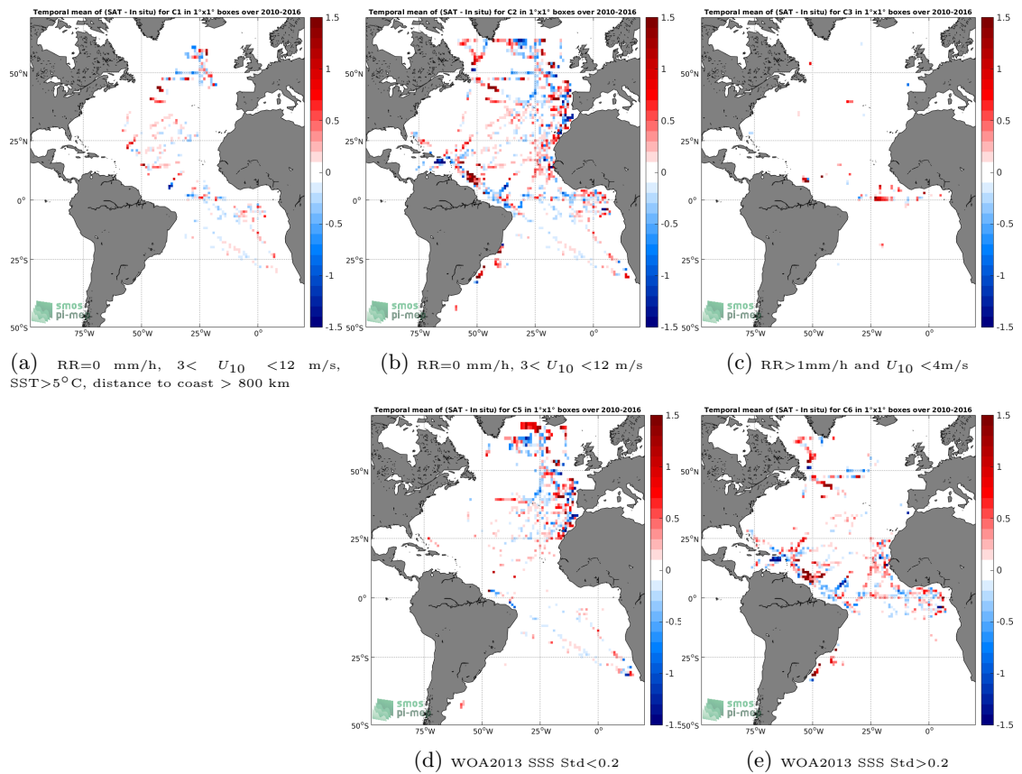
Figure 12: Temporal mean gridded over spatial boxes of size 1^\circ \times 1^\circ of \Delta\text{SSS} (SMOS-L3-ICDC-V3-MONTHLY-0.5DEG - TSG-GOSUD-Research-vessel) for 5 different subdatasets corresponding to:RR=0 mm/h, 3 < U_{10} < 12 m/s, SST>5°C, distance to coast > 800 km (a), RR=0 mm/h, 3 < U_{10} < 12 m/s (b), RR>1mm/h and U_{10} < 4 m/s (c), WOA2013 SSS Std<0.2 (d), WOA2013 SSS Std>0.2 (e).
