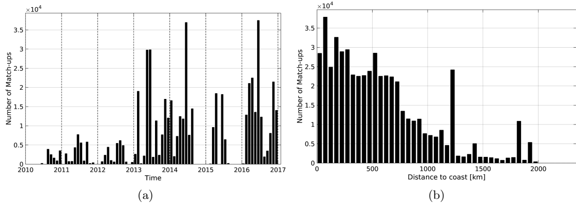
Figure 1: Number of match-ups between TSG-GOSUD-Research-vessel and SMOS-L3-ICDC-V3-MONTHLY-0.5DEG SSS as a function of time (a) and as function of the distance to coast (b) over the Atlantic Ocean Pi-MEP region and for the full satellite product period.
