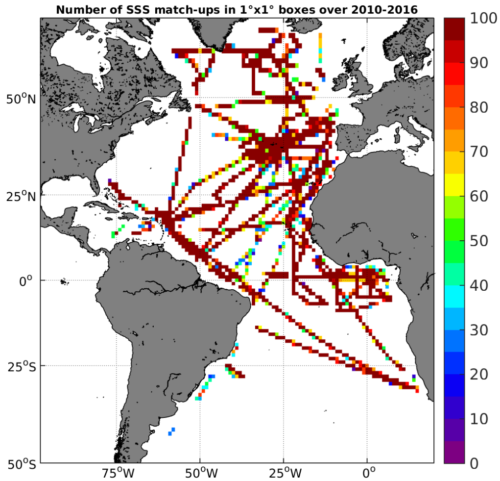
Figure 4: Number of SSS match-ups between TSG-GOSUD-Research-vessel SSS and the SMOS-L3-ICDC-V3-MONTHLY-0.5DEG SSS product for the Atlantic Ocean Pi-MEP region over 1°x1° boxes and for the full satellite product period.
