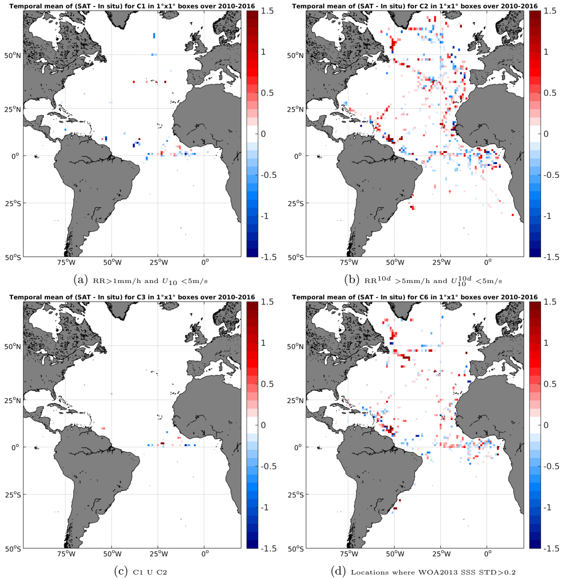
Figure 12: Temporal mean gridded over spatial boxes of size 1^\circ \times 1^\circ of \Delta\text{SSS} (SMOS-L3-ICDC-V3-MONTHLY-0.5DEG - TSG-GOSUD-Research-vessel) for 4 different subdatasets corresponding to: RR > 1\text{mm/h} and U_{10} < 5\text{m/s} (a), RR^{10d} > 5\text{mm/h} and U_{10}^{10d} < 5\text{m/s} (b), C1 U C2 (c), Locations where WOA2013 SSS STD > 0.2 (d).
