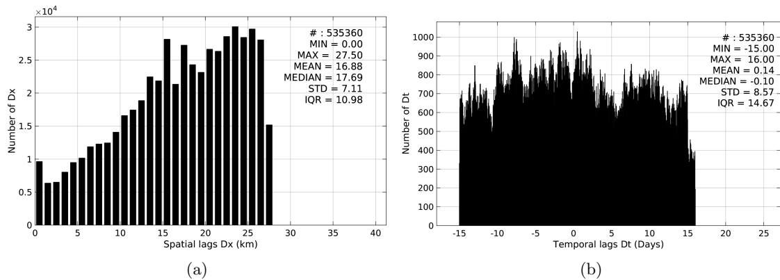
Figure 5: Histograms of the spatial (a) and temporal (b) lags between the time of the TSG-GOSUD-Research-vessel measurements and the date of the corresponding SMOS-L3-ICDC-V3-MONTHLY-0.5DEG SSS product.
