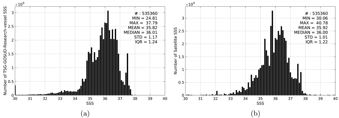
Figure 2: Histograms of SSS from TSG-GOSUD-Research-vessel (a) and SMOS-L3-ICDC-V3-MONTHLY-0.5DEG (b) considering all match-up pairs per bins of 0.1 over the Atlantic Ocean Pi-MEP region and for the full satellite product period.
