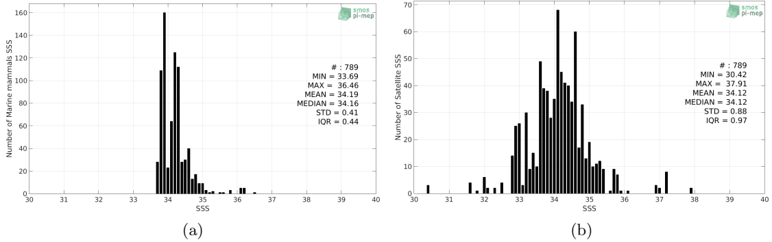
Figure 2: Histograms of SSS from Marine mammals (a) and SMOS SSS L3 v3 Monthly (ICDC) (b) considering all match-up pairs per bins of 0.1 over the Atlantic Ocean Pi-MEP region and for the full satellite product period.
