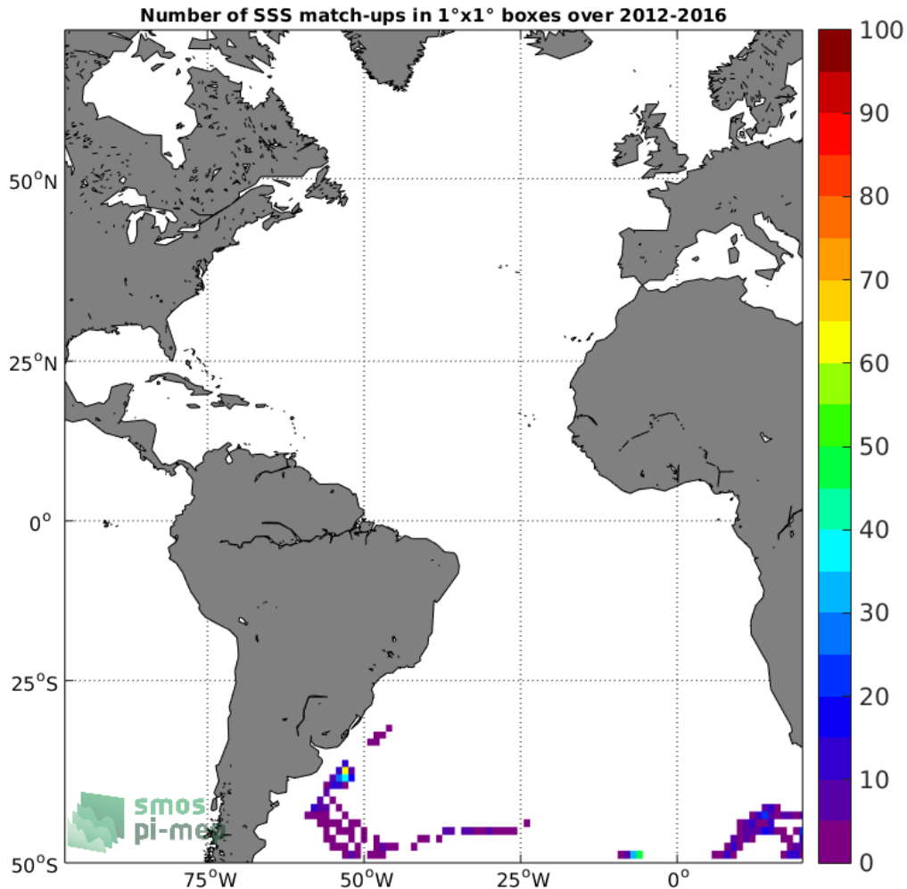
Figure 4: Number of SSS match-ups between Marine mammals SSS and the SMOS SSS L3 v3 Monthly (ICDC) SSS product for the Atlantic Ocean Pi-MEP region over 1^\circ \times 1^\circ boxes and for the full satellite product period.
