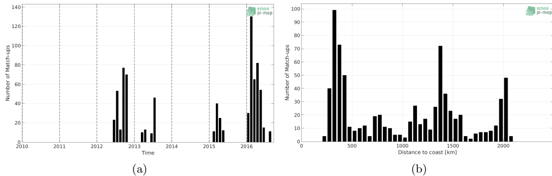
Figure 1: Number of match-ups between Marine mammals and SMOS SSS L3 v3 Monthly (ICDC) SSS as a function of time (a) and as function of the distance to coast (b) over the Atlantic Ocean Pi-MEP region and for the full satellite product period.
