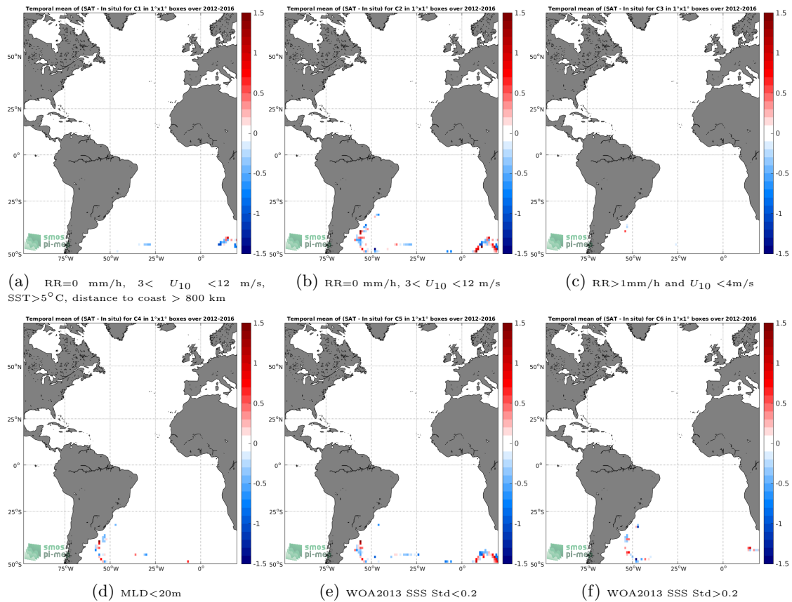
Figure 12: Temporal mean gridded over spatial boxes of size 1^\circ \times 1^\circ of \Delta SSS (SMOS SSS L3 v3 Monthly (ICDC) - Marine mammals) for 6 different subdatasets corresponding to:RR=0 mm/h, 3 < U_{10} < 12 m/s, SST >5^\circ C, distance to coast > 800 km (a), RR=0 mm/h, 3 < U_{10} < 12 m/s (b), RR >1 mm/h and U_{10} < 4 m/s (c),MLD <20 m (d),WOA2013 SSS Std <0.2 (e),WOA2013 SSS Std >0.2 (f).
