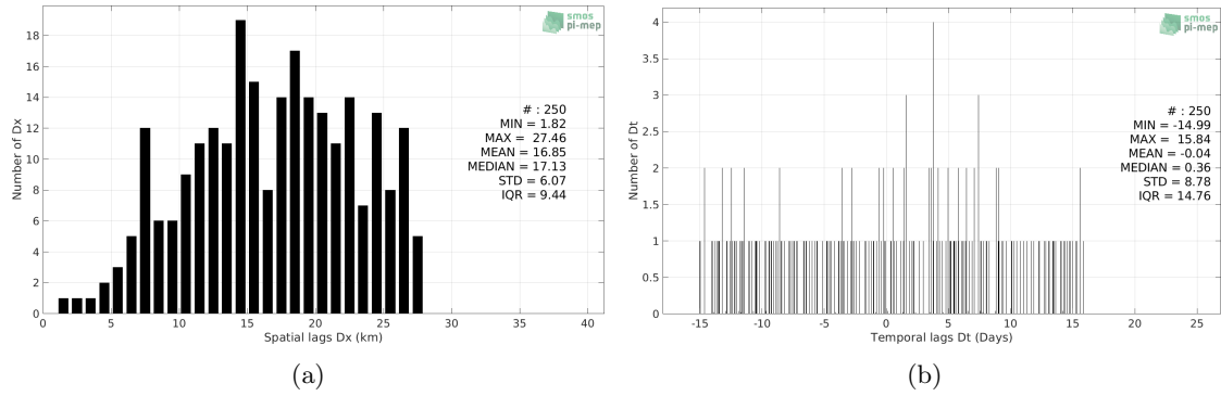
Figure 5: Histograms of the spatial (a) and temporal (b) lags between the location/time of the Sea mammals measurement and the date of the corresponding SMOS SSS L3 v3 Monthly (ICDC) SSS pixel.
