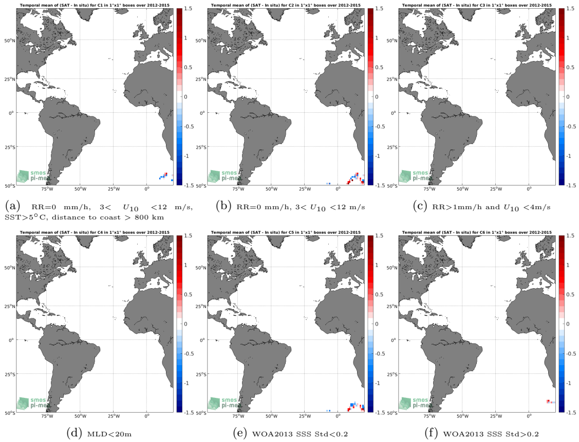
Figure 12: Temporal mean gridded over spatial boxes of size 1°x1° of \Delta SSS (SMOS SSS L3 v3 Monthly (ICDC) - Sea mammals) for 6 different subdatasets corresponding to:RR=0 mm/h, 3 < U_{10} < 12 m/s, SST>5°C, distance to coast > 800 km (a), RR=0 mm/h, 3 < U_{10} < 12 m/s (b), RR>1mm/h and U_{10} < 4 m/s (c),MLD<20m (d),WOA2013 SSS Std<0.2 (e),WOA2013 SSS Std>0.2 (f).
