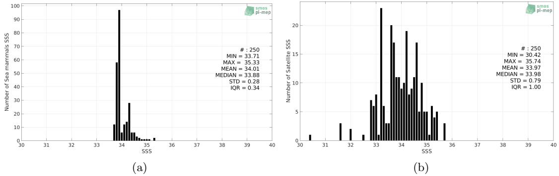
Figure 2: Histograms of SSS from Sea mammals (a) and SMOS SSS L3 v3 Monthly (ICDC) (b) considering all match-up pairs per bins of 0.1 over the Atlantic Ocean Pi-MEP region and for the full satellite product period.
