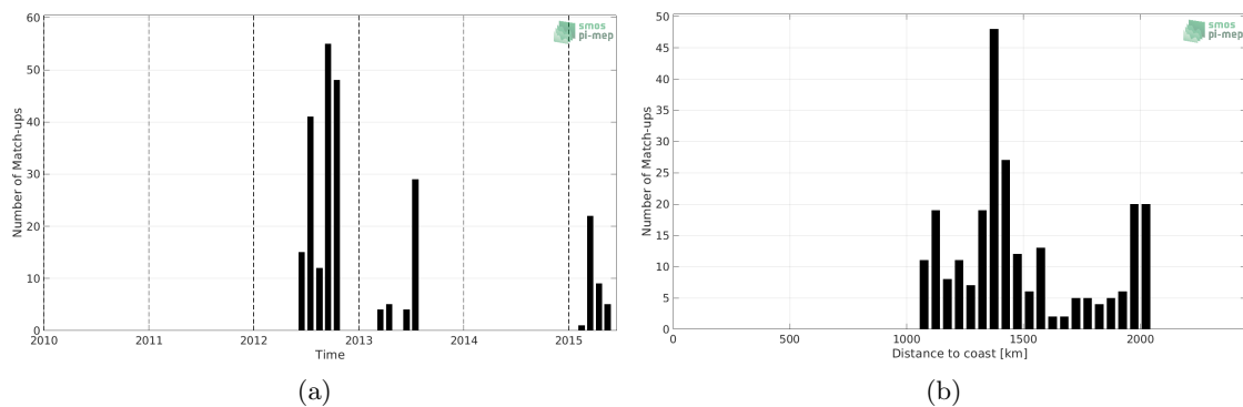
Figure 1: Number of match-ups between Sea mammals and SMOS SSS L3 v3 Monthly (ICDC) SSS as a function of time (a) and as function of the distance to coast (b) over the Atlantic Ocean Pi-MEP region and for the full satellite product period.
