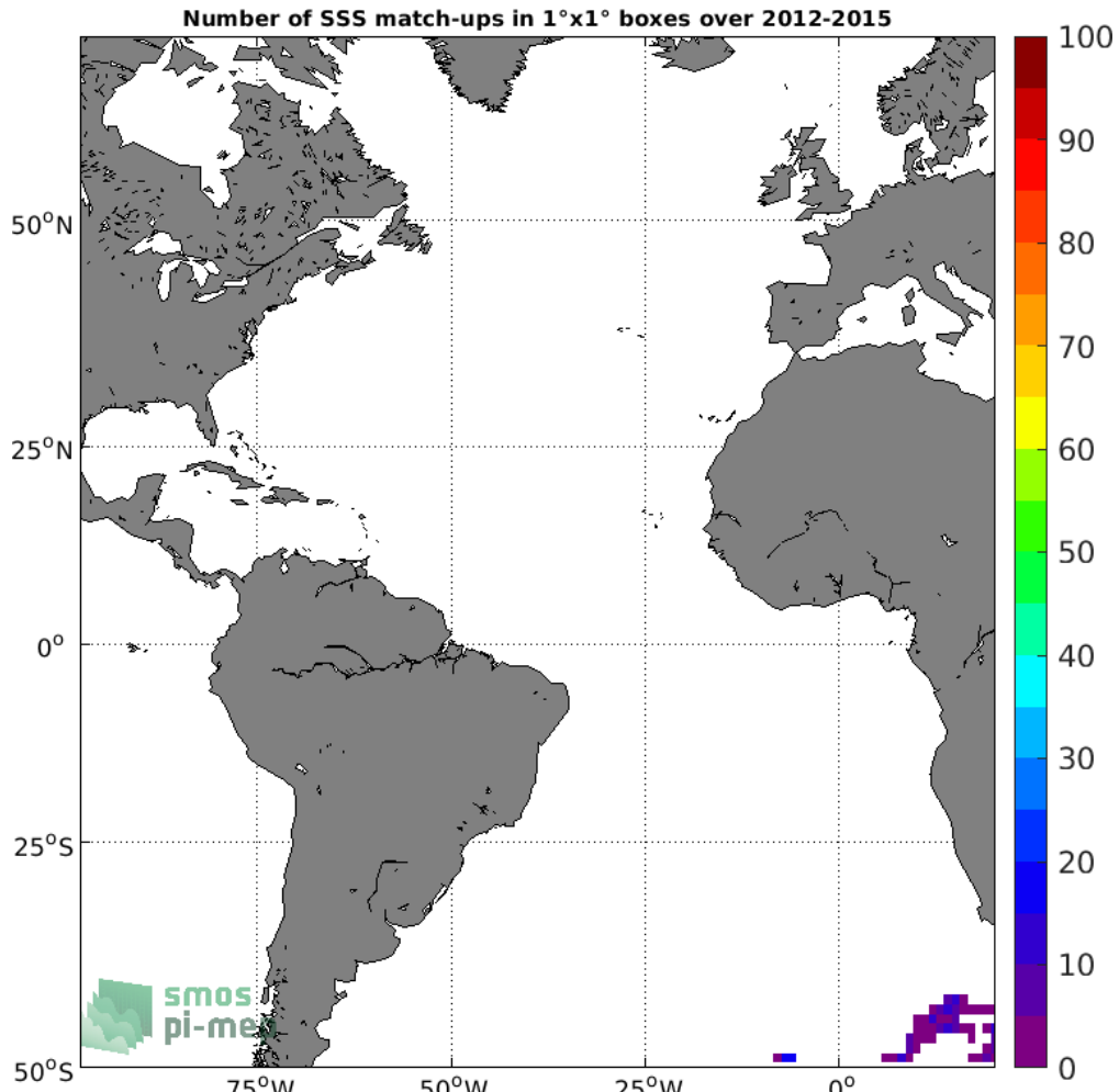
Figure 4: Number of SSS match-ups between Sea mammals SSS and the SMOS SSS L3 v3 Monthly (ICDC) SSS product for the Atlantic Ocean Pi-MEP region over 1^\circ \times 1^\circ boxes and for the full satellite product period.
