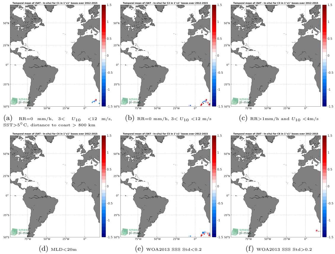
Figure 12: Temporal mean gridded over spatial boxes of size 1^\circ \times 1^\circ of \Delta SSS (SMOS SSS L3 v3 Monthly (ICDC) - Sea mammals) for 6 different subdatasets corresponding to:RR=0 mm/h, 3 < U_{10} < 12 m/s, SST>5°C, distance to coast > 800 km (a), RR=0 mm/h, 3 < U_{10} < 12 m/s (b), RR>1mm/h and U_{10} < 4 m/s (c),MLD<20m (d),WOA2013 SSS Std<0.2 (e),WOA2013 SSS Std>0.2 (f).
