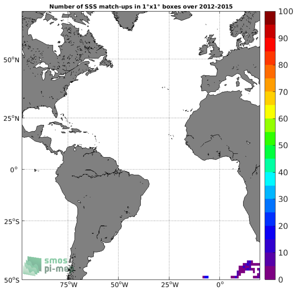
Figure 4: Number of SSS match-ups between Sea mammals SSS and the SMOS SSS L3 v3 Monthly (ICDC) SSS product for the Atlantic Ocean Pi-MEP region over 1°x1° boxes and for the full satellite product period.
