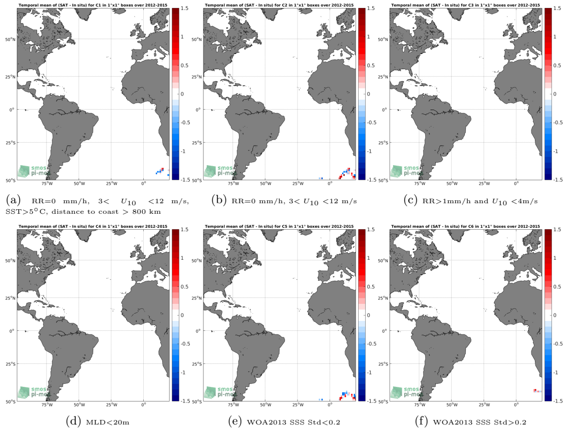
Figure 12: Temporal mean gridded over spatial boxes of size 1°x1° of \Delta SSS (SMOS-L3-ICDC-V3-MONTHLY-0.5DEG - Sea mammals) for 6 different subdatasets corresponding to:RR=0 mm/h, 3 < U_{10} < 12 m/s, SST>5°C, distance to coast > 800 km (a), RR=0 mm/h, 3 < U_{10} < 12 m/s (b), RR>1mm/h and U_{10} < 4 m/s (c),MLD<20m (d),WOA2013 SSS Std<0.2 (e),WOA2013 SSS Std>0.2 (f).
