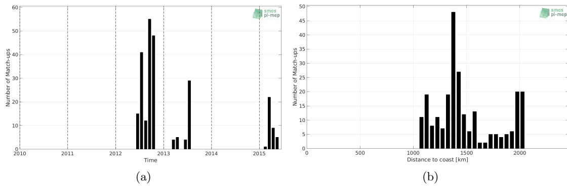
Figure 1: Number of match-ups between Sea mammals and SMOS-L3-ICDC-V3-MONTHLY-0.5DEG SSS as a function of time (a) and as function of the distance to coast (b) over the Atlantic Ocean Pi-MEP region and for the full satellite product period.
