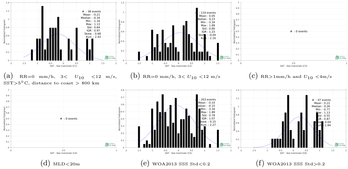
Figure 13: Normalized histogram of \Delta SSS (SMOS-L3-ICDC-V3-MONTHLY-0.5DEG - Sea mammals) for 6 different subdatasets corresponding to: RR=0 mm/h, 3 < U_{10} < 12 m/s, SST>5°C, distance to coast > 800 km (a), RR=0 mm/h, 3 < U_{10} < 12 m/s (b), RR>1mm/h and U_{10} < 4 m/s (c), MLD<20m (d), WOA2013 SSS Std<0.2 (e), WOA2013 SSS Std>0.2 (f).
