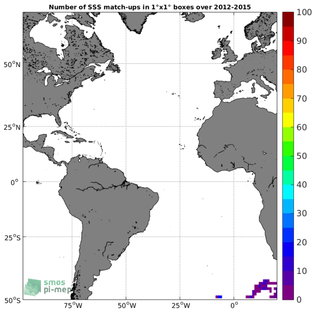
Figure 4: Number of SSS match-ups between Sea mammals SSS and the SMOS-L3-ICDC-V3-MONTHLY-0.5DEG SSS product for the Atlantic Ocean Pi-MEP region over 1°x1° boxes and for the full satellite product period.
