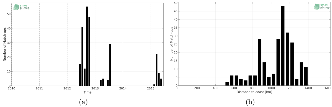
Figure 1: Number of match-ups between Sea mammals and SMOS-L3-ICDC-V3-MONTHLY-0.5DEG SSS as a function of time (a) and as function of the distance to coast (b) over the Atlantic Ocean Pi-MEP region and for the full satellite product period.
