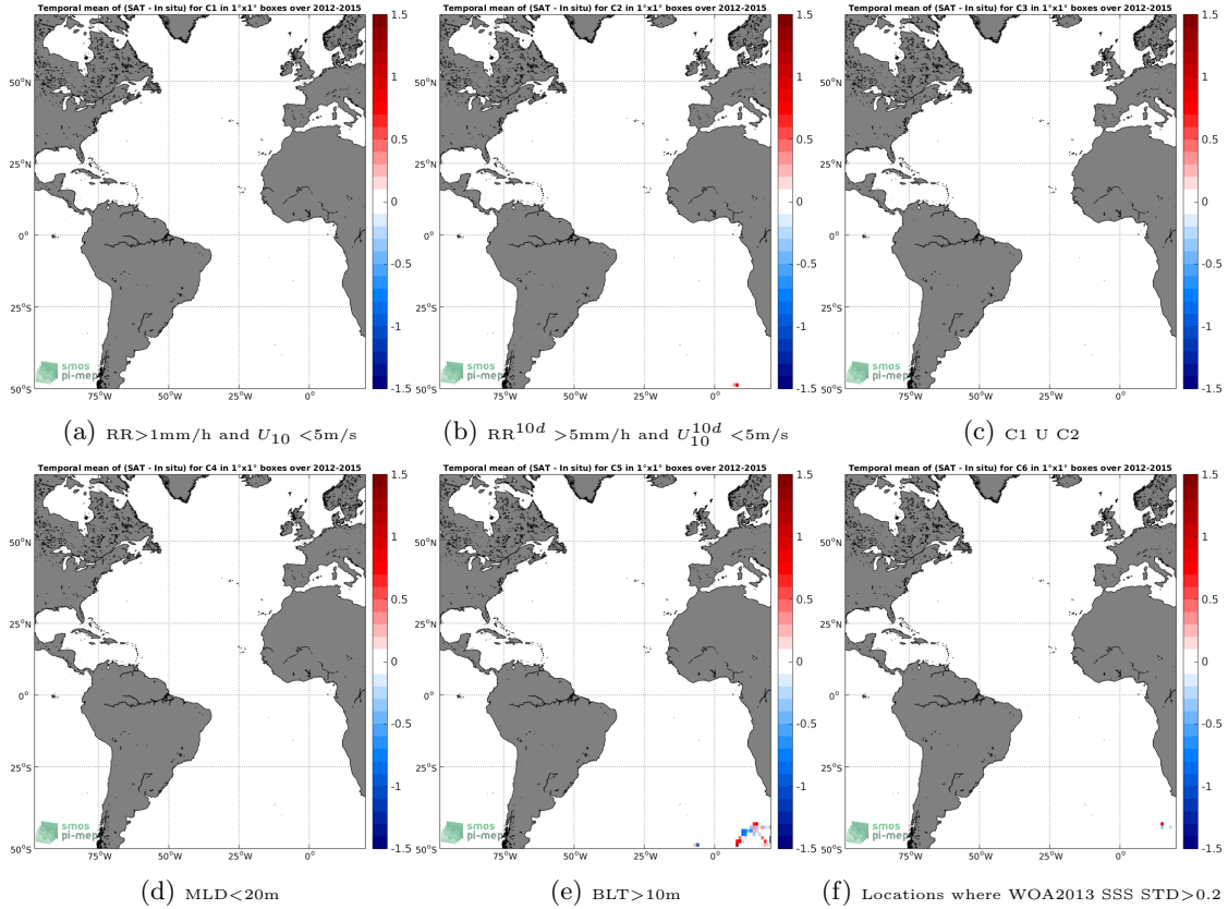
Figure 12: Temporal mean gridded over spatial boxes of size 1^\circ \times 1^\circ of \Delta\text{SSS} (SMOS-L3-ICDC-V3-MONTHLY-0.5DEG - Sea mammals) for 6 different subdatasets corresponding to: \text{RR} > 1\text{mm/h} and U_{10} < 5\text{m/s} (a), \text{RR}^{10d} > 5\text{mm/h} and U_{10}^{10d} < 5\text{m/s} (b), C1 U C2 (c), \text{MLD} < 20\text{m} (d), \text{BLT} > 10\text{m} (e), Locations where WOA2013 SSS STD > 0.2 (f).
