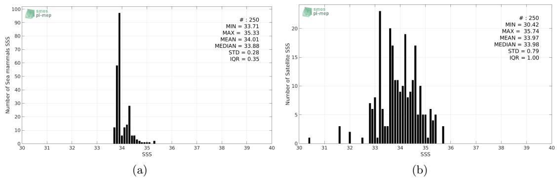
Figure 2: Histograms of SSS from Sea mammals (a) and SMOS-L3-ICDC-V3-MONTHLY-0.5DEG (b) considering all match-up pairs per bins of 0.1 over the Atlantic Ocean Pi-MEP region and for the full satellite product period.
