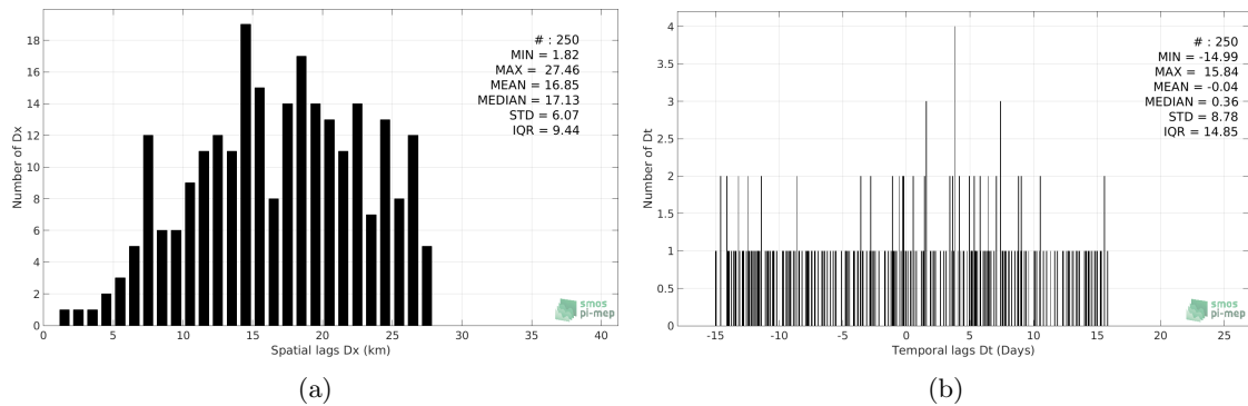
Figure 5: Histograms of the spatial (a) and temporal (b) lags between the time of the Sea mammals measurements and the date of the corresponding SMOS-L3-ICDC-V3-MONTHLY-0.5DEG SSS product.
