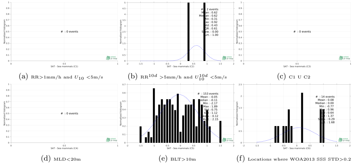
Figure 13: Normalized histogram of \Delta\text{SSS} (SMOS-L3-ICDC-V3-MONTHLY-0.5DEG - Sea mammals) for 6 different subdatasets corresponding to: RR>1mm/h and U_{10} < 5\text{m/s} (a), \text{RR}^{10d} > 5\text{mm/h} and U_{10}^{10d} < 5\text{m/s} (b), C1 U C2 (c), MLD<20m (d), BLT>10m (e), Locations where WOA2013 SSS STD>0.2 (f).
