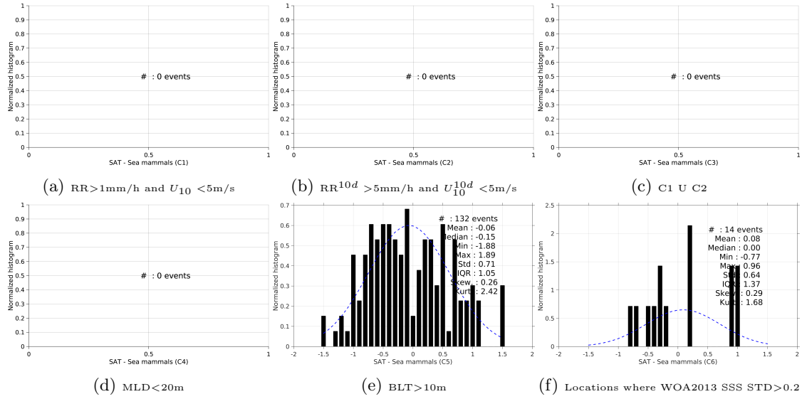
Figure 13: Normalized histogram of \Delta\text{SSS} (SMOS-L3-ICDC-V3-MONTHLY-0.5DEG - Sea mammals) for 6 different subdatasets corresponding to: RR>1mm/h and U_{10} < 5\text{m/s} (a), \text{RR}^{10d} > 5\text{mm/h} and U_{10}^{10d} < 5\text{m/s} (b), C1 U C2 (c), MLD<20m (d), BLT>10m (e), Locations where WOA2013 SSS STD>0.2 (f).
