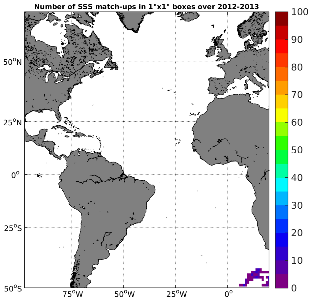
Figure 4: Number of SSS match-ups between Sea mammals SSS and the SMOS-L3-ICDC-V3-MONTHLY-0.5DEG SSS product for the Atlantic Ocean Pi-MEP region over 1°x1° boxes and for the full satellite product period.
