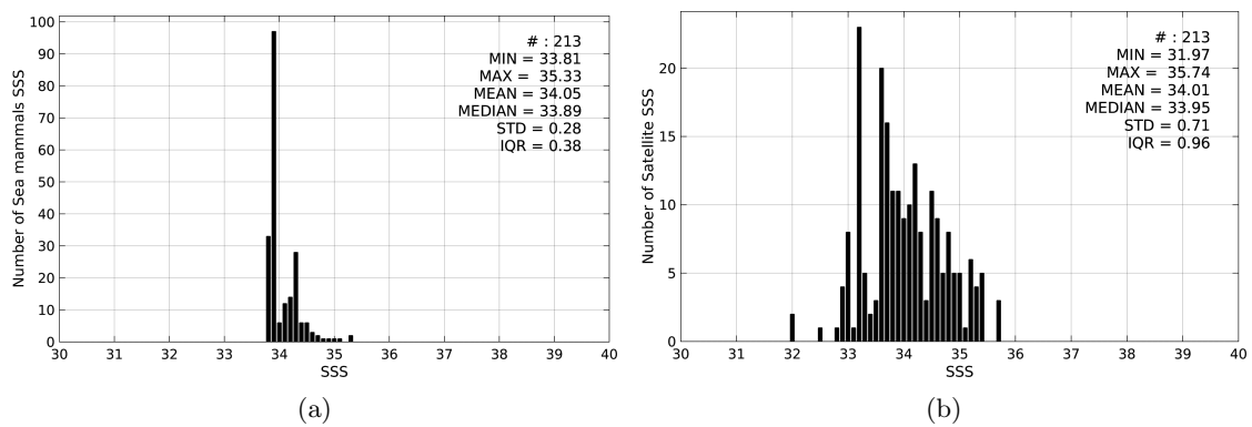
Figure 2: Histograms of SSS from Sea mammals (a) and SMOS-L3-ICDC-V3-MONTHLY-0.5DEG (b) considering all match-up pairs per bins of 0.1 over the Atlantic Ocean Pi-MEP region and for the full satellite product period.
