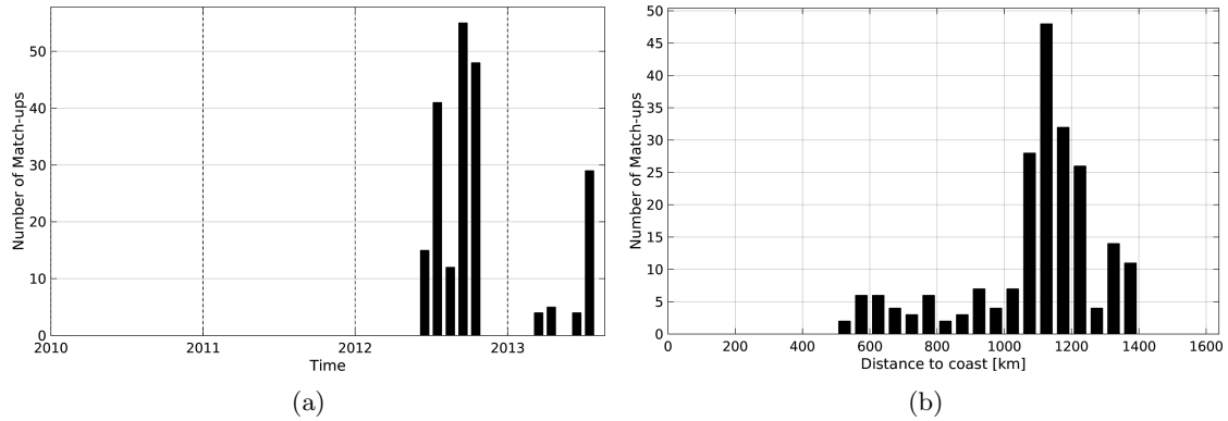
Figure 1: Number of match-ups between Sea mammals and SMOS-L3-ICDC-V3-MONTHLY-0.5DEG SSS as a function of time (a) and as function of the distance to coast (b) over the Atlantic Ocean Pi-MEP region and for the full satellite product period.
