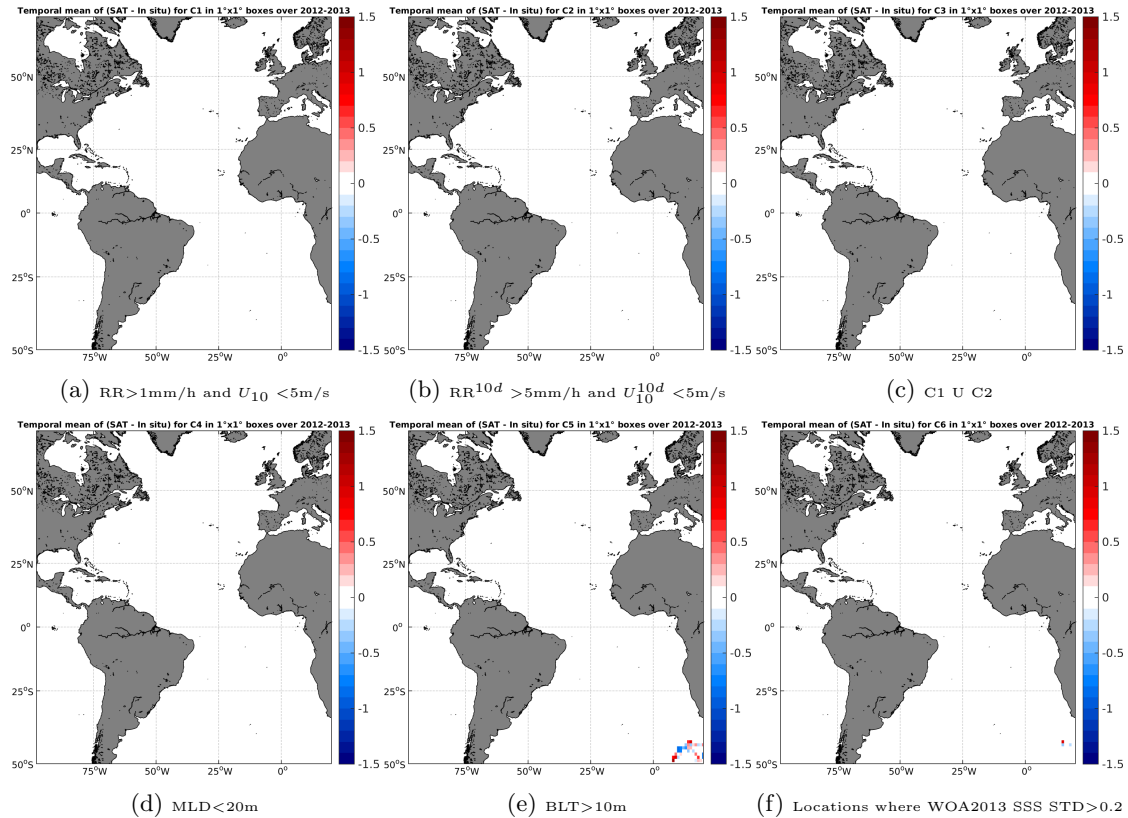
Figure 12: Temporal mean gridded over spatial boxes of size 1^\circ \times 1^\circ of \Delta SSS (SMOS-L3-ICDC-V3-MONTHLY-0.5DEG - Sea mammals) for 6 different subdatasets corresponding to:RR>1mm/h and U_{10} < 5 m/s (a), RR^{10d} > 5 mm/h and U_{10}^{10d} < 5 m/s (b), C1 U C2 (c),MLD<20m (d),BLT>10m (e),Locations where WOA2013 SSS STD>0.2 (f).
