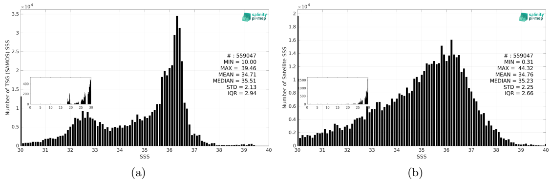
Figure 3: Histograms of SSS from TSG (SAMOS) (a) and SMOS SSS L2Q v331 - With FLAG (CMEMS-CATDS-CPDC) (b) considering all match-up pairs per bins of 0.1 over the Atlantic Ocean Pi-MEP region and for the full satellite product period.
