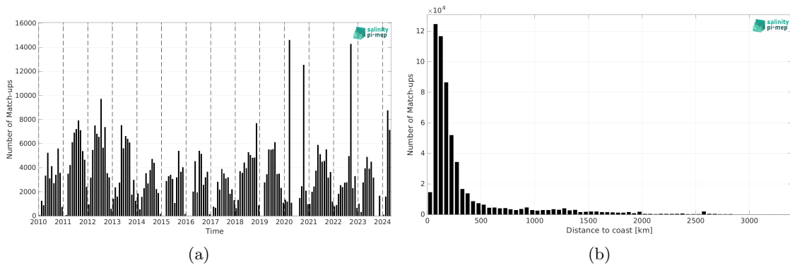
Figure 2: Number of match-ups between TSG (SAMOS) and SMOS SSS L2Q v331 - With FLAG (CMEMS-CATDS-CPDC) SSS as a function of time (a) and as function of the distance to coast (b) over the Atlantic Ocean Pi-MEP region and for the full satellite product period.
