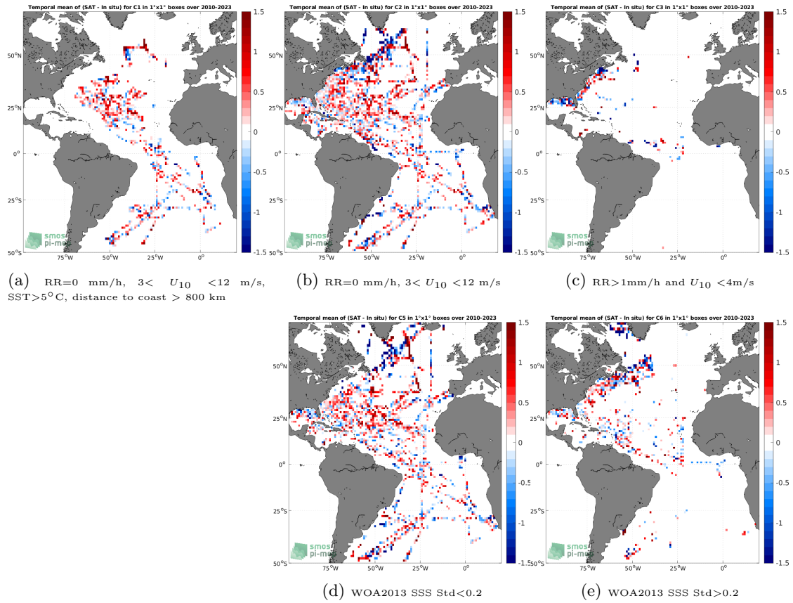
Figure 12: Temporal mean gridded over spatial boxes of size 1^\circ \times 1^\circ of \Delta\text{SSS} (SMOS SSS L2Q v331 - With FLAG (CMEMS-CATDS-CPDC) - TSG (SAMOS)) for 5 different subdatasets corresponding to:RR=0 mm/h, 3 < U_{10} < 12 m/s, SST >5^\circ\text{C} , distance to coast > 800 km (a), RR=0 mm/h, 3 < U_{10} < 12 m/s (b), RR >1 mm/h and U_{10} < 4 m/s (c), WOA2013 SSS Std <0.2 (d), WOA2013 SSS Std >0.2 (e).
