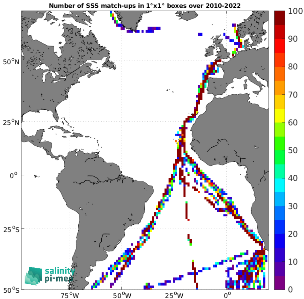
Figure 4: Number of SSS match-ups between TSG (Polarstern) SSS and the SMOS SSS L2Q v331 - With FLAG (CMEMS-CATDS-CPDC) SSS product for the Atlantic Ocean Pi-MEP region over 1^\circ \times 1^\circ boxes and for the full satellite product period.
