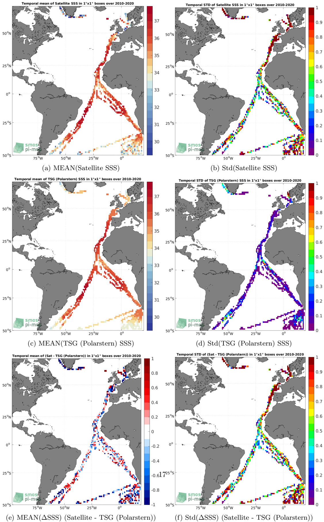
Figure 6: Temporal mean (left) and Std (right) of SSS from SMOS SSS L2Q v331 - With FLAG (CMEMS-CATDS-CPDC) (top), TSG (Polarstern) (middle), and of \Delta SSS (Satellite - TSG (Polarstern)). Only match-up pairs are used to generate these maps.
