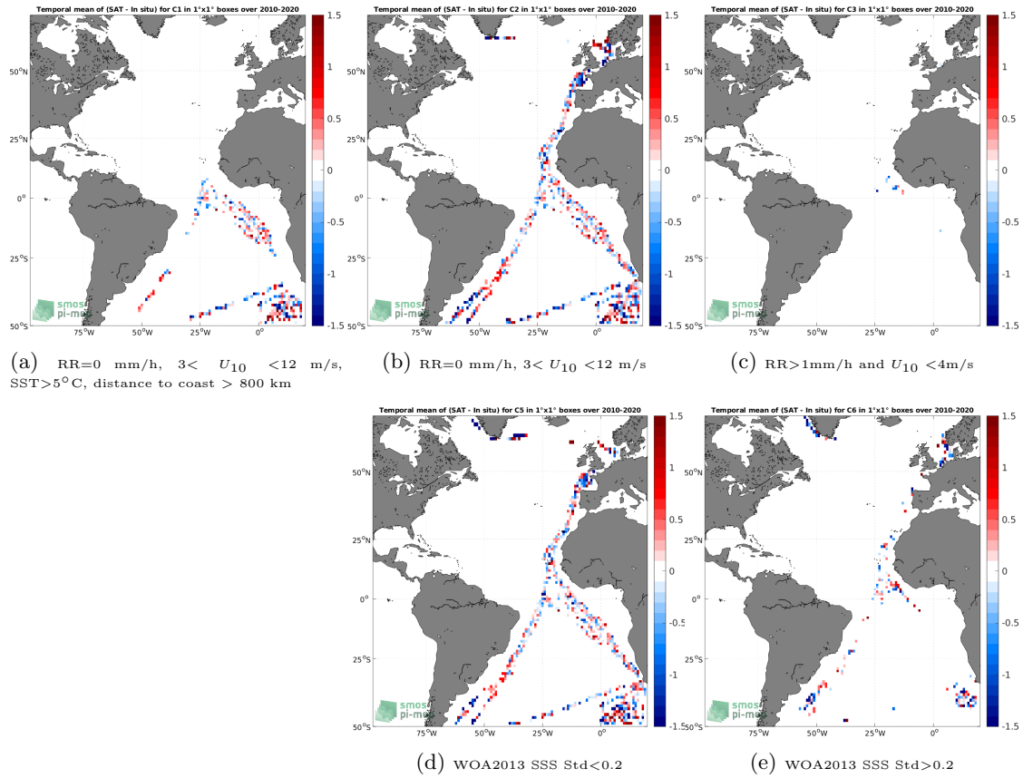
Figure 12: Temporal mean gridded over spatial boxes of size 1^\circ \times 1^\circ of \Delta SSS (SMOS SSS L2Q v331 - With FLAG (CMEMS-CATDS-CPDC) - TSG (Polarstern)) for 5 different subdatasets corresponding to:RR=0 mm/h, 3 < U_{10} < 12 m/s, SST >5^\circ C, distance to coast > 800 km (a), RR=0 mm/h, 3 < U_{10} < 12 m/s (b), RR >1 mm/h and U_{10} < 4 m/s (c), WOA2013 SSS Std <0.2 (d), WOA2013 SSS Std >0.2 (e).
