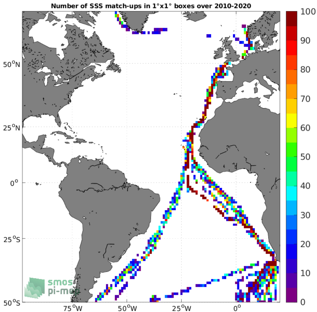
Figure 4: Number of SSS match-ups between TSG (Polarstern) SSS and the SMOS SSS L2Q v331 - With FLAG (CMEMS-CATDS-CPDC) SSS product for the Atlantic Ocean Pi-MEP region over 1°x1° boxes and for the full satellite product period.
