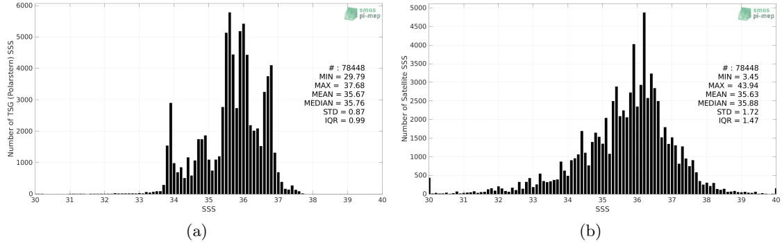
Figure 2: Histograms of SSS from TSG (Polarstern) (a) and SMOS SSS L2Q v331 - With FLAG (CMEMS-CATDS-CPDC) (b) considering all match-up pairs per bins of 0.1 over the Atlantic Ocean Pi-MEP region and for the full satellite product period.
