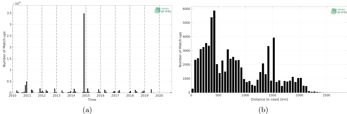
Figure 1: Number of match-ups between TSG (Polarstern) and SMOS SSS L2Q v331 - With FLAG (CMEMS-CATDS-CPDC) SSS as a function of time (a) and as function of the distance to coast (b) over the Atlantic Ocean Pi-MEP region and for the full satellite product period.
