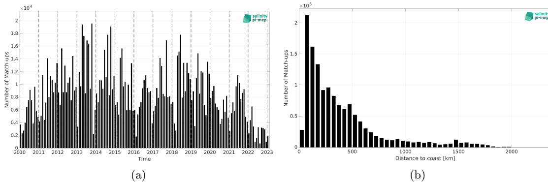
Figure 2: Number of match-ups between TSG (LEGOS-DM) and SMOS SSS L2Q v331 - With FLAG (CMEMS-CATDS-CPDC) SSS as a function of time (a) and as function of the distance to coast (b) over the Atlantic Ocean Pi-MEP region and for the full satellite product period.
