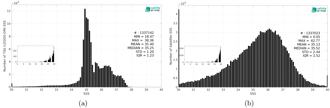
Figure 3: Histograms of SSS from TSG (LEGOS-DM) (a) and SMOS SSS L2Q v331 - With FLAG (CMEMS-CATDS-CPDC) (b) considering all match-up pairs per bins of 0.1 over the Atlantic Ocean Pi-MEP region and for the full satellite product period.
