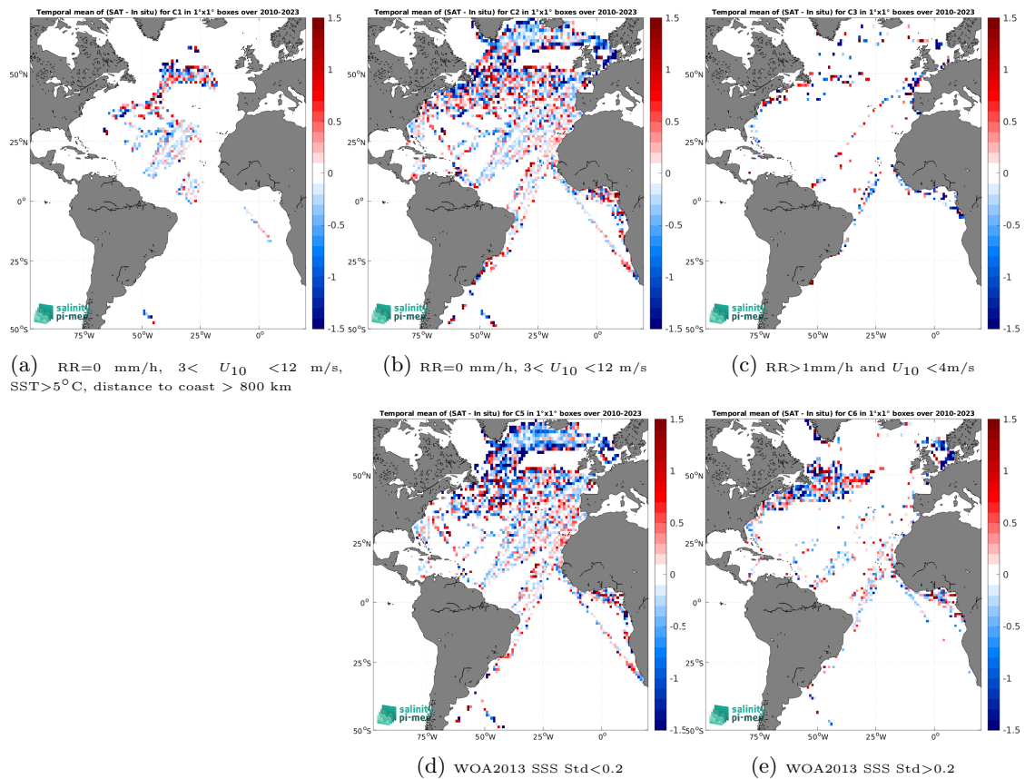
Figure 14: Temporal mean gridded over spatial boxes of size 1^\circ \times 1^\circ of \Delta\text{SSS} (SMOS SSS L2Q v331 - With FLAG (CMEMS-CATDS-CPDC) - TSG (LEGOS-DM)) for 5 different subdatasets corresponding to:RR=0 mm/h, 3 < U_{10} < 12 m/s, SST >5^\circ\text{C} , distance to coast > 800 km (a), RR=0 mm/h, 3 < U_{10} < 12 m/s (b), RR >1 mm/h and U_{10} < 4 m/s (c), WOA2013 SSS Std <0.2 (d), WOA2013 SSS Std >0.2 (e).
