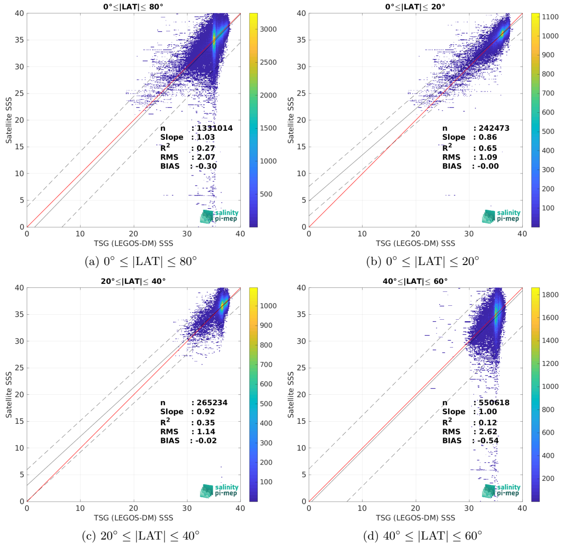
Figure 10: Contour maps of the concentration of SMOS SSS L2Q v331 - With FLAG (CMEMS-CATDS-CPDC) SSS (y-axis) versus TSG (LEGOS-DM) SSS (x-axis) at match-up pairs for different latitude bands. For each plot, the red line shows x=y . The black thin and dashed lines indicate a linear fit through the data cloud and the \pm 95\% confidence levels, respectively. The number match-up pairs n , the slope and R^2 coefficient of the linear fit, the root mean square (RMS) and the mean bias between satellite and in situ data are indicated for each latitude band in each plots.
