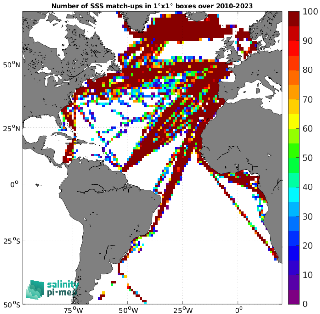
Figure 5: Number of SSS match-ups between TSG (LEGOS-DM) SSS and the SMOS SSS L2Q v331 - With FLAG (CMEMS-CATDS-CPDC) SSS product for the Atlantic Ocean Pi-MEP region over 1^\circ \times 1^\circ boxes and for the full satellite product period.
