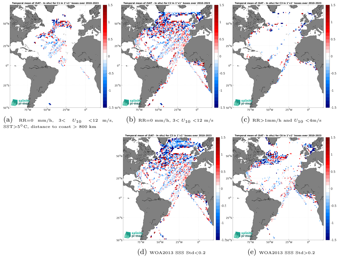
Figure 12: Temporal mean gridded over spatial boxes of size 1^\circ \times 1^\circ of \Delta SSS (SMOS SSS L2Q v331 - With FLAG (CMEMS-CATDS-CPDC) - TSG (LEGOS-DM)) for 5 different subdatasets corresponding to:RR=0 mm/h, 3 < U_{10} < 12 m/s, SST >5^\circ\text{C} , distance to coast > 800 km (a), RR=0 mm/h, 3 < U_{10} < 12 m/s (b), RR >1 mm/h and U_{10} < 4 m/s (c), WOA2013 SSS Std <0.2 (d), WOA2013 SSS Std >0.2 (e).
