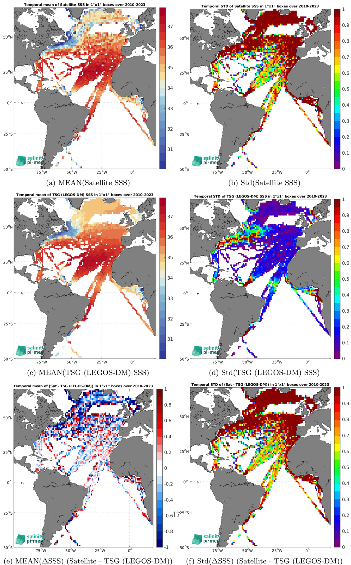
Figure 6: Temporal mean (left) and Std (right) of SSS from SMOS SSS L2Q v331 - With FLAG (CMEMS-CATDS-CPDC) (top), TSG (LEGOS-DM) (middle), and of \Delta SSS (Satellite - TSG (LEGOS-DM)). Only match-up pairs are used to generate these maps.
