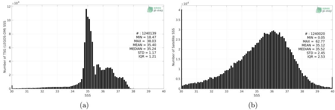
Figure 2: Histograms of SSS from TSG (LEGOS-DM) (a) and SMOS SSS L2Q v331 - With FLAG (CMEMS-CATDS-CPDC) (b) considering all match-up pairs per bins of 0.1 over the Atlantic Ocean Pi-MEP region and for the full satellite product period.
