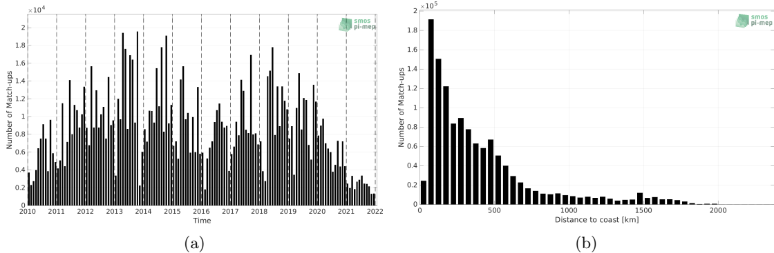
Figure 1: Number of match-ups between TSG (LEGOS-DM) and SMOS SSS L2Q v331 - With FLAG (CMEMS-CATDS-CPDC) SSS as a function of time (a) and as function of the distance to coast (b) over the Atlantic Ocean Pi-MEP region and for the full satellite product period.
