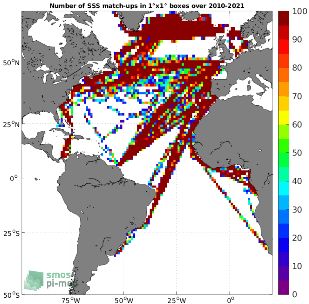
Figure 4: Number of SSS match-ups between TSG (LEGOS-DM) SSS and the SMOS SSS L2Q v331 - With FLAG (CMEMS-CATDS-CPDC) SSS product for the Atlantic Ocean Pi-MEP region over 1^\circ \times 1^\circ boxes and for the full satellite product period.
