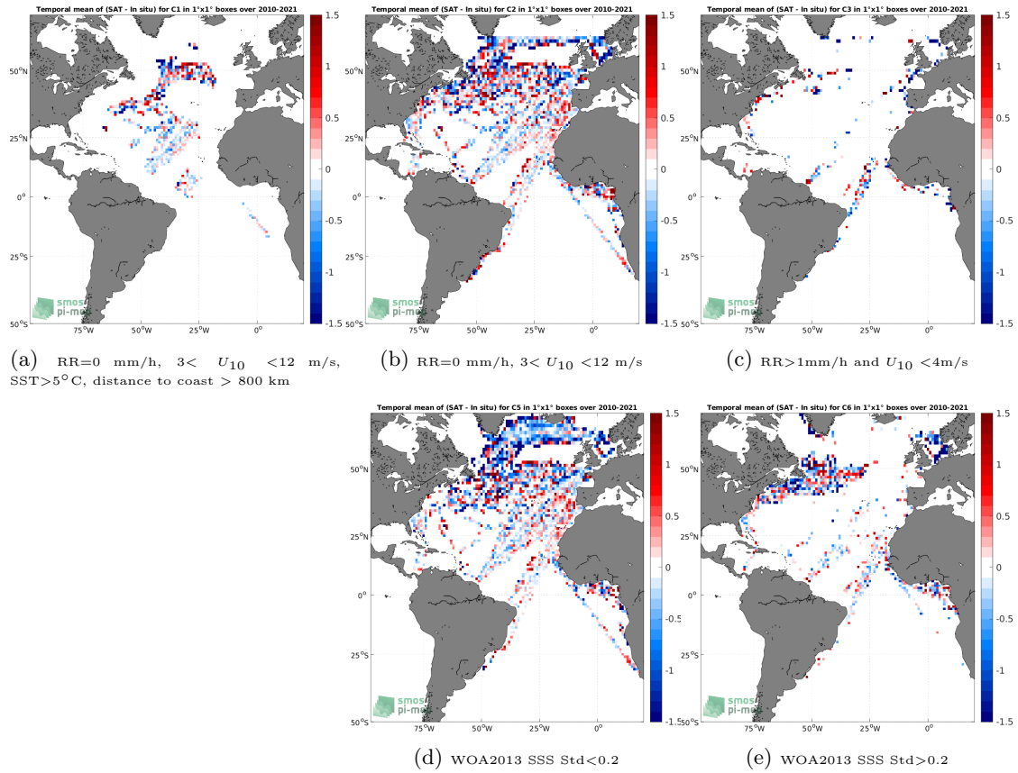
Figure 12: Temporal mean gridded over spatial boxes of size 1^\circ \times 1^\circ of \Delta\text{SSS} (SMOS SSS L2Q v331 - With FLAG (CMEMS-CATDS-CPDC) - TSG (LEGOS-DM)) for 5 different subdatasets corresponding to:RR=0 mm/h, 3 < U_{10} < 12 m/s, SST >5^\circ\text{C} , distance to coast > 800 km (a), RR=0 mm/h, 3 < U_{10} < 12 m/s (b), RR >1 mm/h and U_{10} < 4 m/s (c), WOA2013 SSS Std <0.2 (d), WOA2013 SSS Std >0.2 (e).
