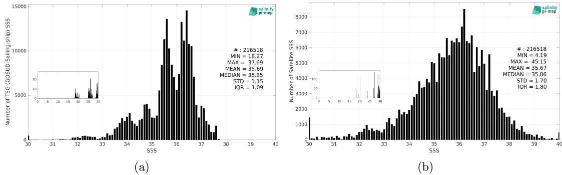
Figure 3: Histograms of SSS from TSG (GOSUD-Sailing-ship) (a) and SMOS SSS L2Q v331 - With FLAG (CMEMS-CATDS-CPDC) (b) considering all match-up pairs per bins of 0.1 over the Atlantic Ocean Pi-MEP region and for the full satellite product period.
