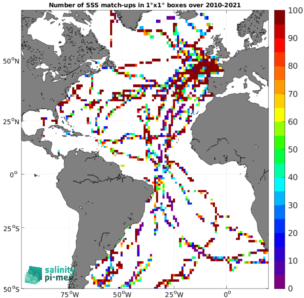
Figure 5: Number of SSS match-ups between TSG (GOSUD-Sailing-ship) SSS and the SMOS SSS L2Q v331 - With FLAG (CMEMS-CATDS-CPDC) SSS product for the Atlantic Ocean Pi-MEP region over 1^\circ \times 1^\circ boxes and for the full satellite product period.
