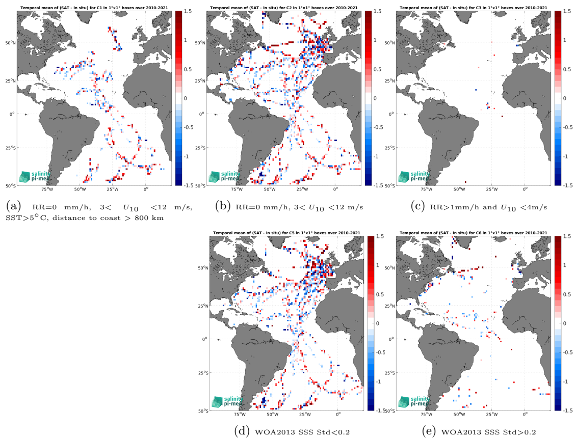
Figure 14: Temporal mean gridded over spatial boxes of size 1^\circ \times 1^\circ of \Delta\text{SSS} (SMOS SSS L2Q v331 - With FLAG (CMEMS-CATDS-CPDC) - TSG (GOSUD-Sailing-ship)) for 5 different subdatasets corresponding to:RR=0 mm/h, 3 < U_{10} < 12 m/s, SST>5°C, distance to coast > 800 km (a), RR=0 mm/h, 3 < U_{10} < 12 m/s (b), RR>1mm/h and U_{10} < 4 m/s (c), WOA2013 SSS Std<0.2 (d), WOA2013 SSS Std>0.2 (e).
